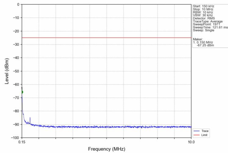
Band7 15MHz QPSK MCH 2535MHz RB 1 0 NTN
