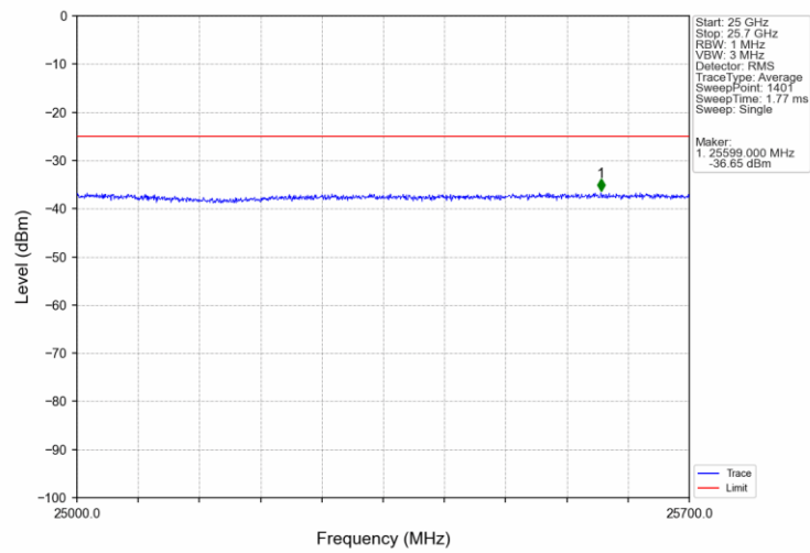
Band7 10MHz 16QAM MCH 2535MHz RB 1 0 NTV
