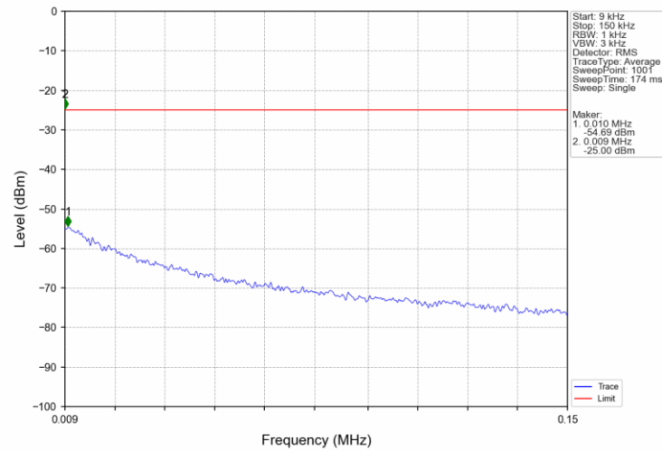
Band7 15MHz QPSK MCH 2535MHz RB 1 0 NTN
