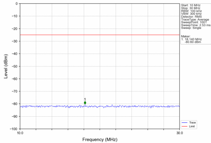
Band7 15MHz 16QAM MCH 2535MHz RB 1 0 NTV
