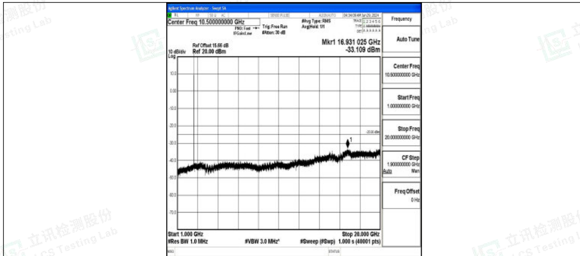
Band7_5MHz_QPSK_21425_1RB#0_1000~20000_1000~20000
