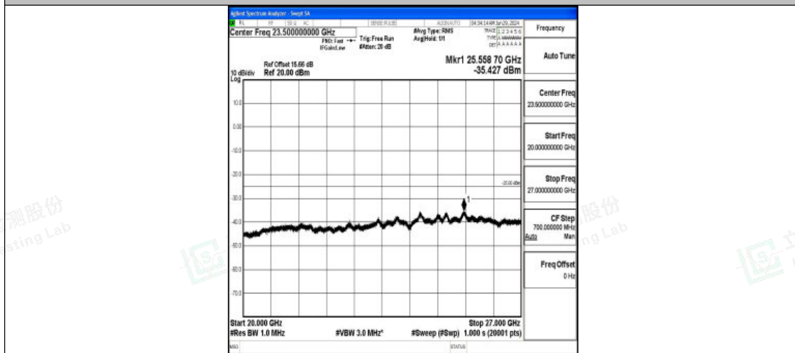
Band7_5MHz_QPSK_21425_1RB#0_20000~27000_20000~27000
