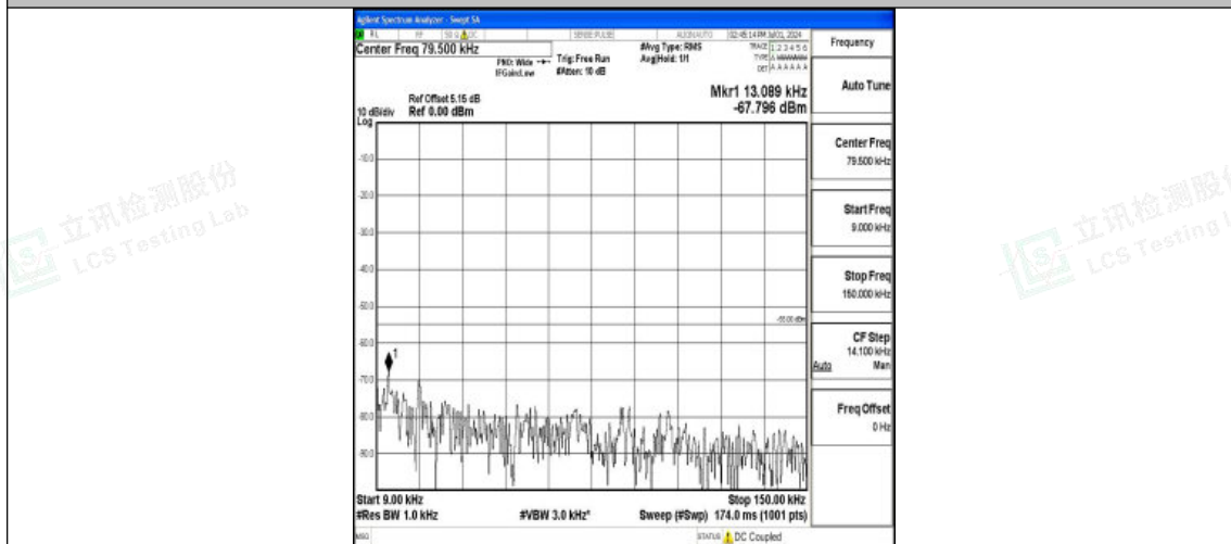
Band7_20MHz_16QAM_21350_1RB#0_0.009~0.15_0.009~0.15
