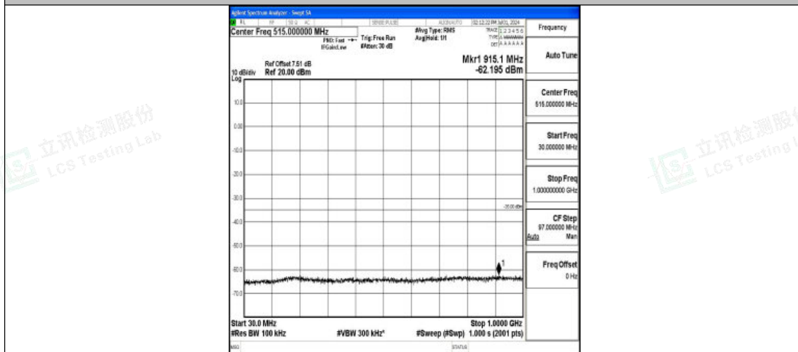
Band7_10MHz_QPSK_21400_1RB#0_30~1000_30~1000
