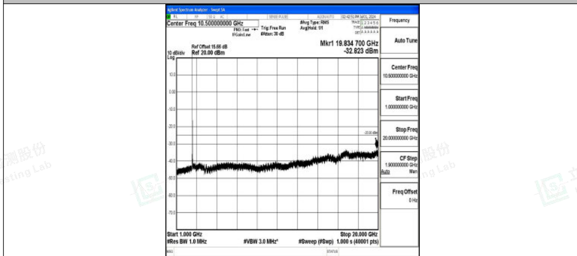
Band7_20MHz_QPSK_20850_1RB#0_1000~20000_1000~20000
