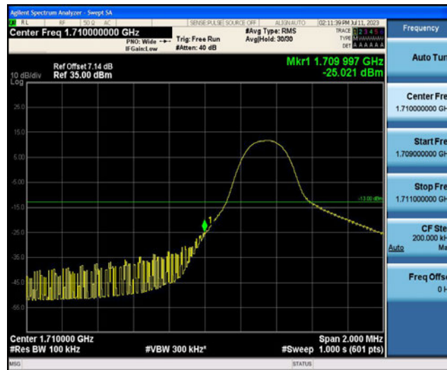
Band4-5MHz-16QAM-19975-1RB#24
