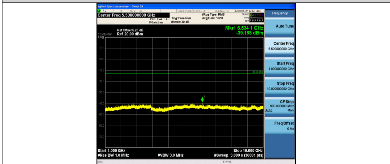
Band5-4182-1000~10000MHz
