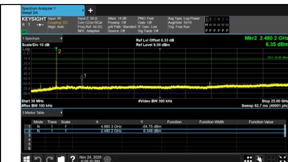
30.0 MHz - 25000.0 MHz BLE 1M_Channel 39
