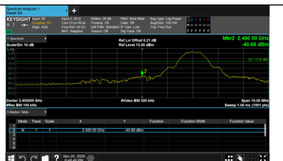
Out Of Band Emission BLE 1M Channel 0
