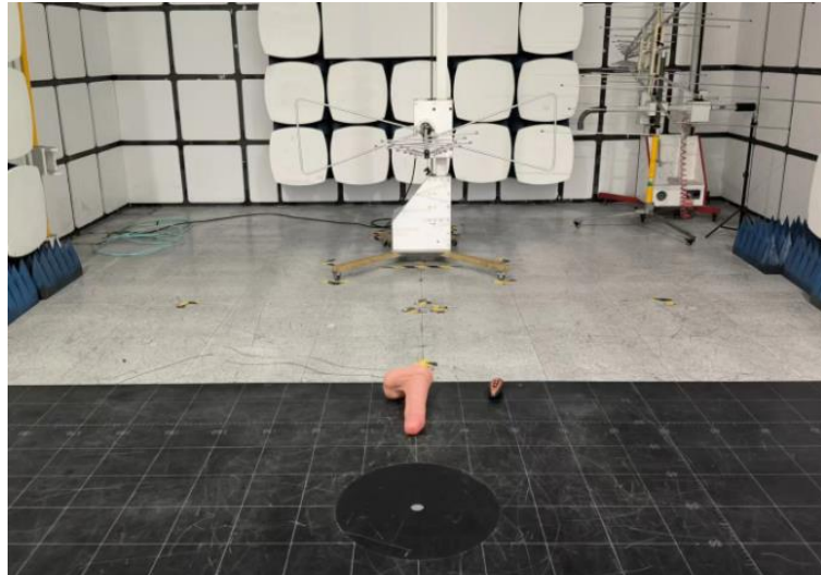
Radiated emission 30MHz~1GHz
