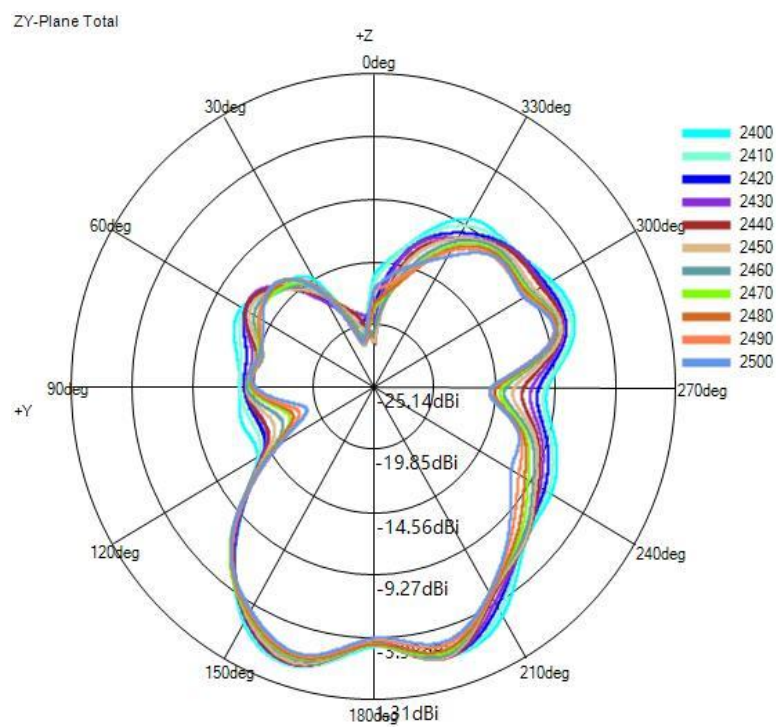
(2) Y-Z Plane(unit:dBi):
