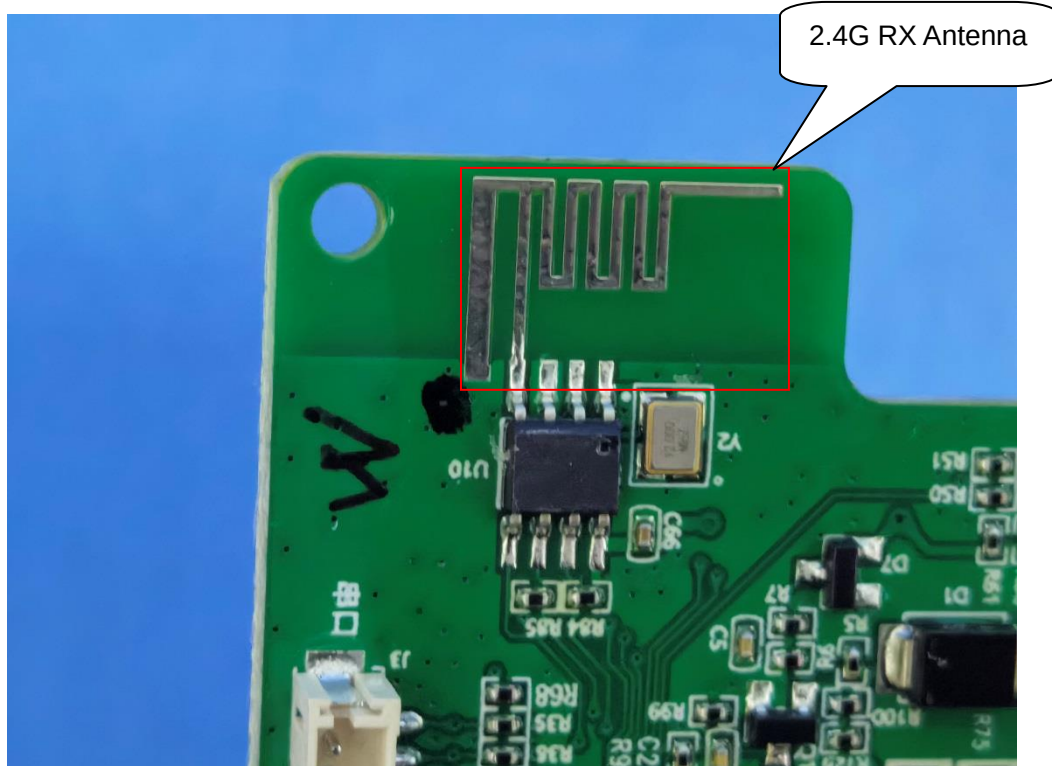
INTERNAL VIEW OF EUT (FIGURE 6)
