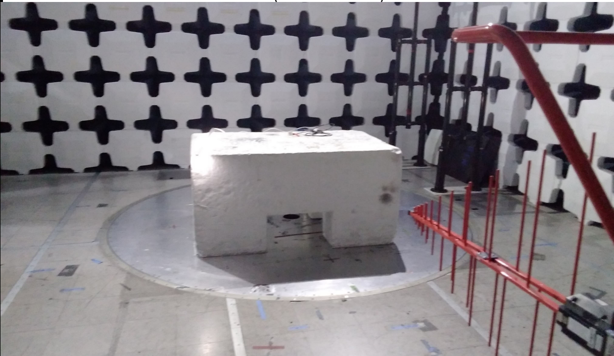
Test Configuration Photograph #2 (Radiated Emissions)
