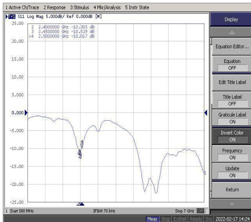
WIFI 2.4G
