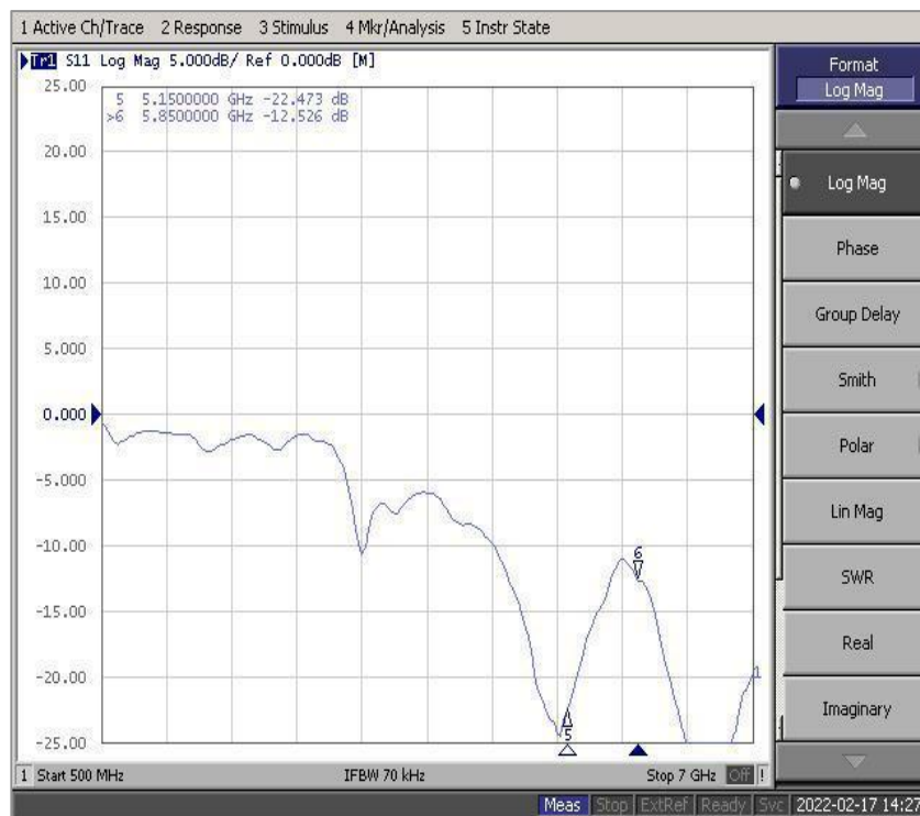
WIFI 5.8G
