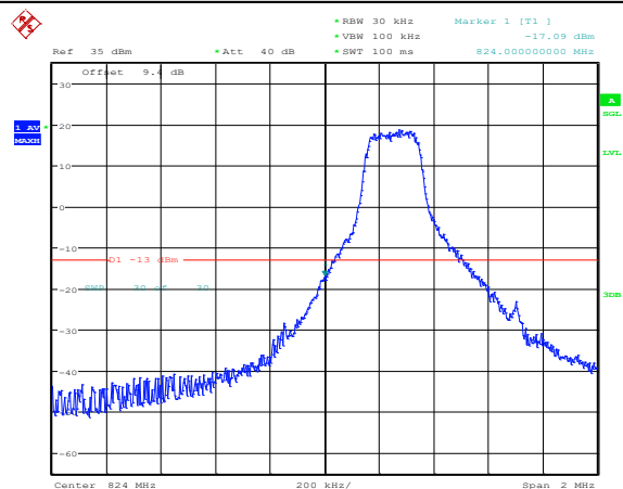
Band5-1.4MHz-16QAM-20407-1RB#0
