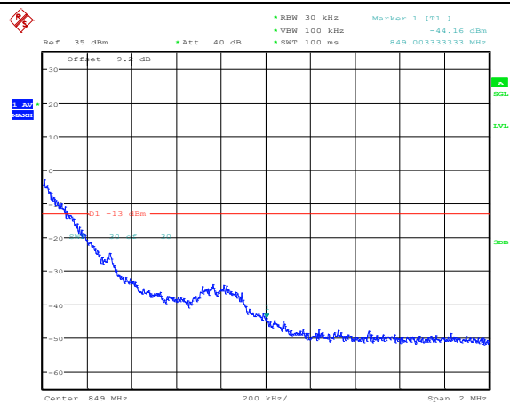
Band5-1.4MHz-QPSK-20643-1RB#5
