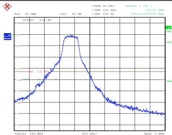
Band5-1.4MHz-QPSK-20643-1RB#5
