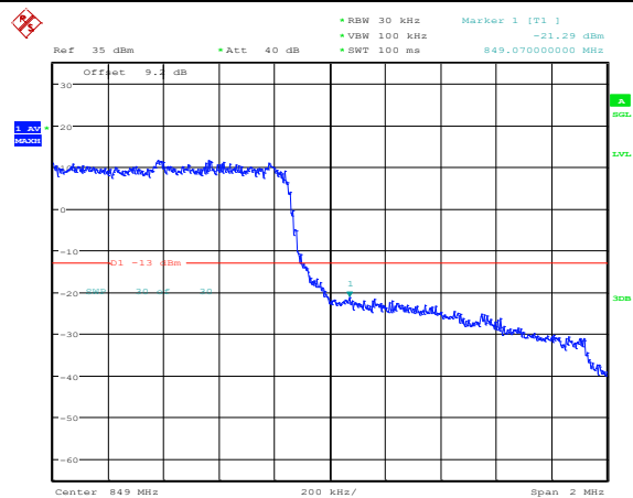
Band5-1.4MHz-QPSK-20643-6RB#0
