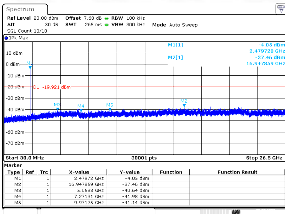
Tx. Spurious NVNT 3-DH1 2480MHz Ant1 Emission
