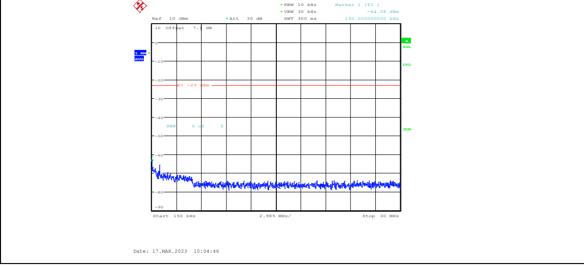
Band4-5MHz-16QAM-20375-1RB#0-Range2:0.15~30MHz
