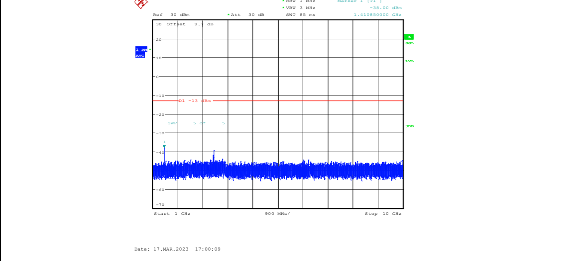
Band12-5MHz-QPSK-23095-1RB#0-Range4:1000~10000MHz
