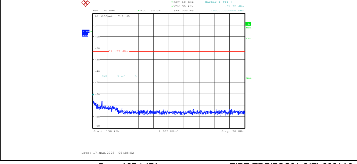
Band4-1.4MHz-16QAM-19957-1RB#0-Range2:0.15~30MHz
