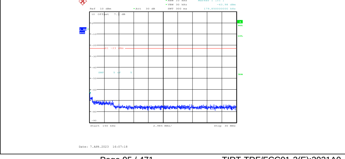
Band2-1.4MHz-16QAM-18607-1RB#0-Range2:0.15~30MHz
