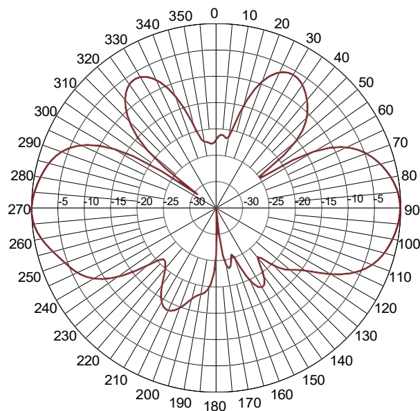
Elevation Pattern at 2450MHz
