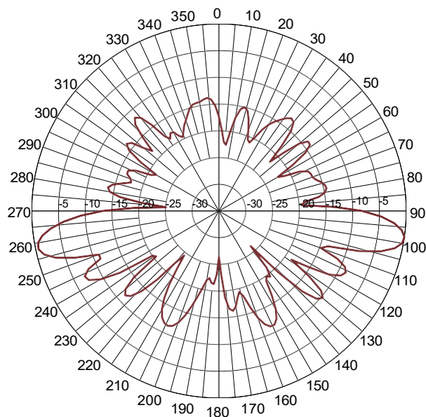
Elevation Pattern at 2440MHz
