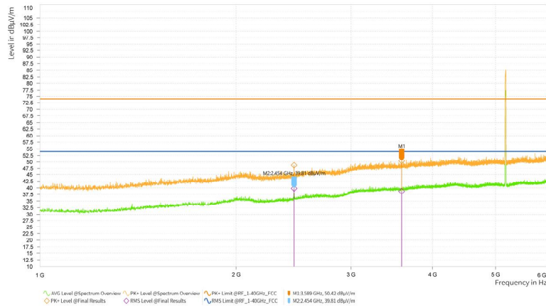
RE(Above 1 GHz)_802.11a_5 180 MHz
