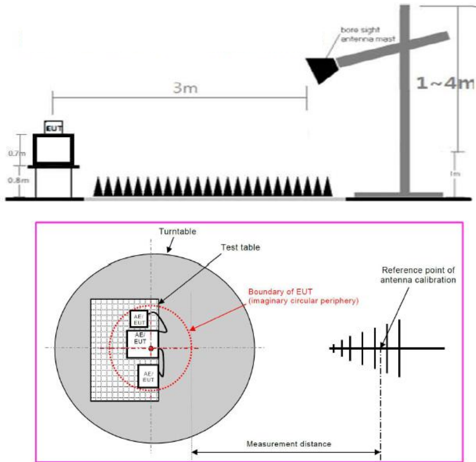
[Radiated Emission Test Setup Above 1 GHz]
