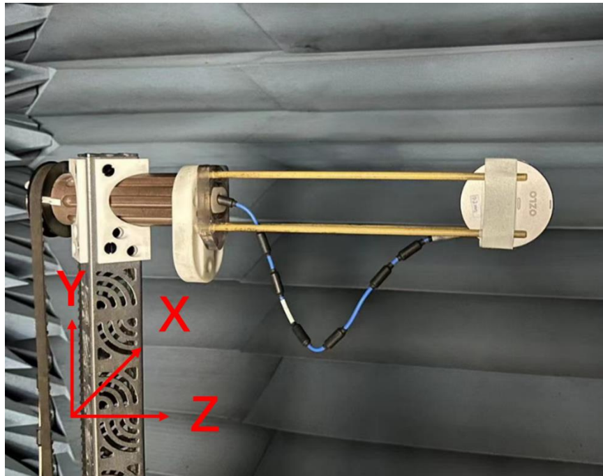
Charge Case
