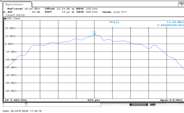
BLE_2M_Ant2_2402_0~Reference
