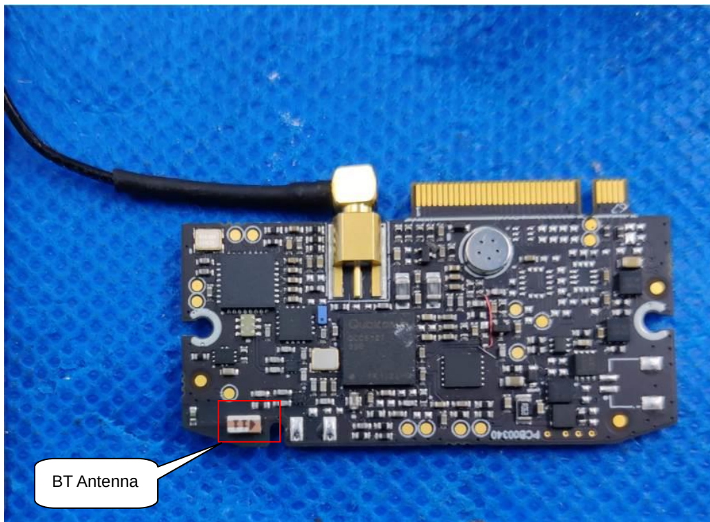
BT Antenna
