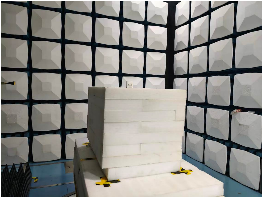
Radiated Emission 60-90GHz View
