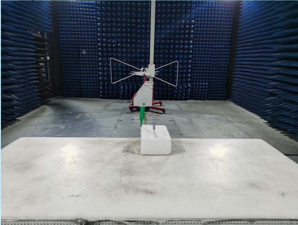
Radiated Spurious Emission Test View 2
