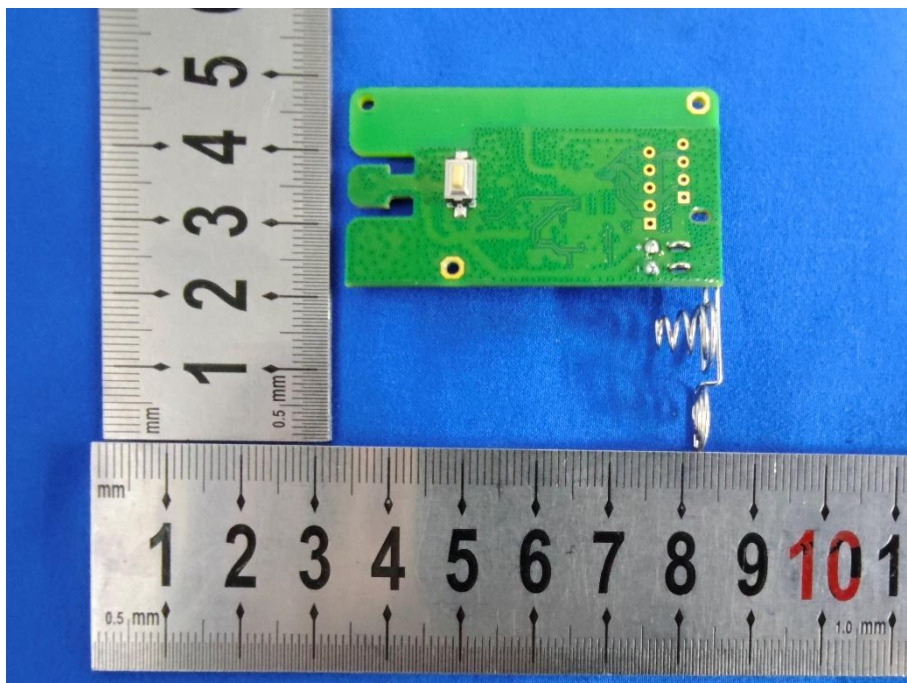
Photo 2: Internal View for PCB
