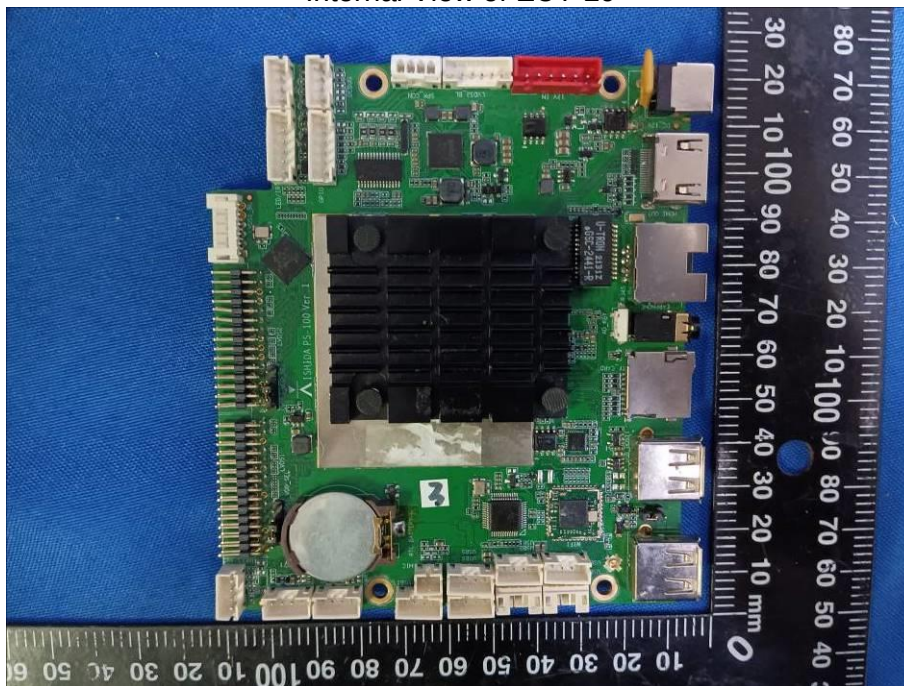
Internal View of EUT-29
