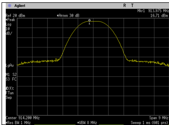
LoRa_High Ch_914.2MHz_500kHz_Output Power
