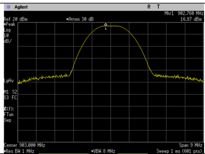
LoRa_Low Ch_903MHz_500kHz_Output Power
