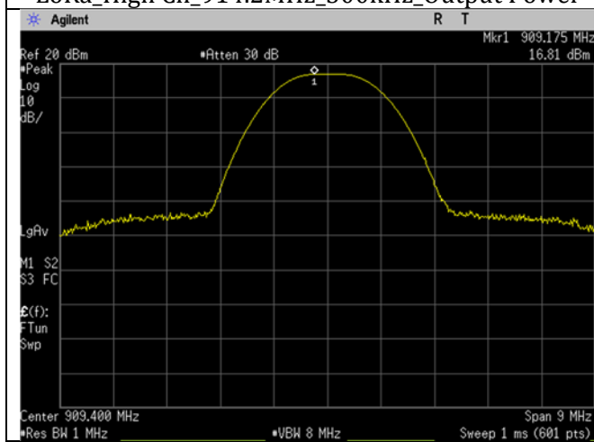
LoRa_Mid Ch_909.4MHz_500kHz_Output Power
