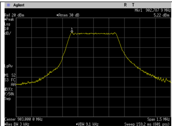
LoRa_Low Ch_903MHz_500kHz_Spectral Density
