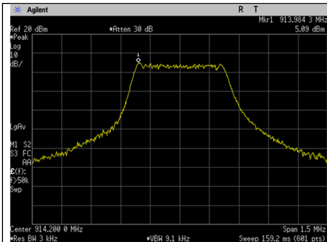
LoRa_High Ch_914.2MHz_500kHz_Spectral Density
