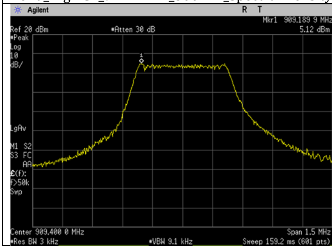
LoRa_Mid Ch_909.4MHz_500kHz_Spectral Density
