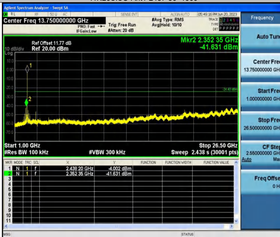
11N20SISO-Ant1-2437-1000~26500
