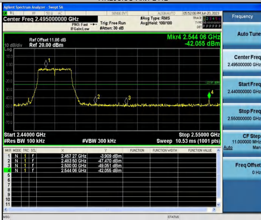
11N20SISO-Ant1-2462
