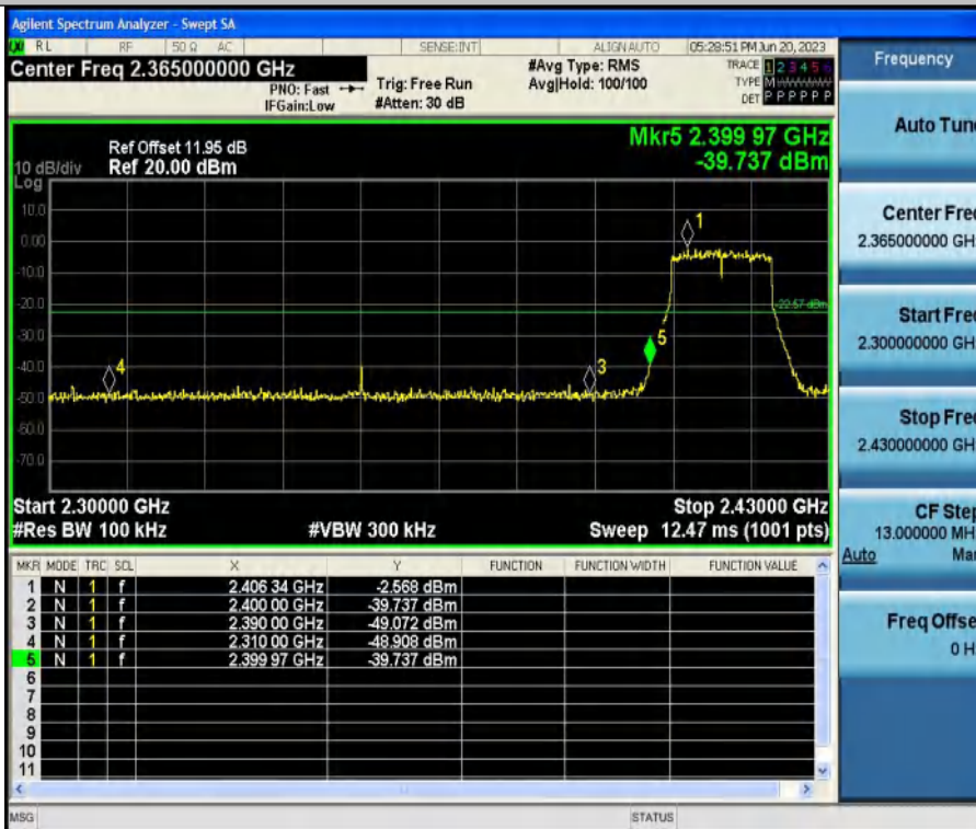
11G-Ant1-2412
