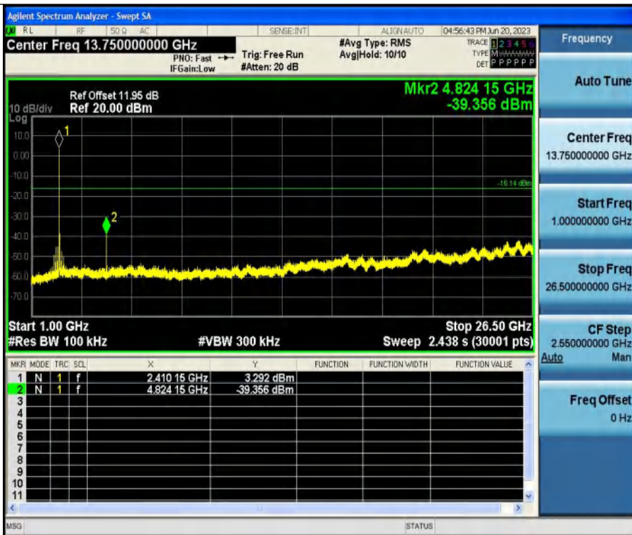
11B-Ant1-2412-1000~26500
