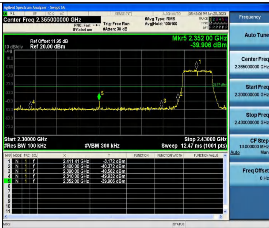
11N20SISO-Ant1-2412
