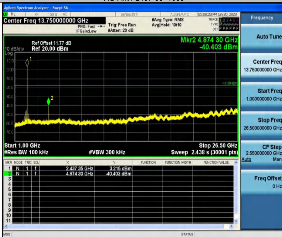
11B-Ant1-2437-1000~26500
