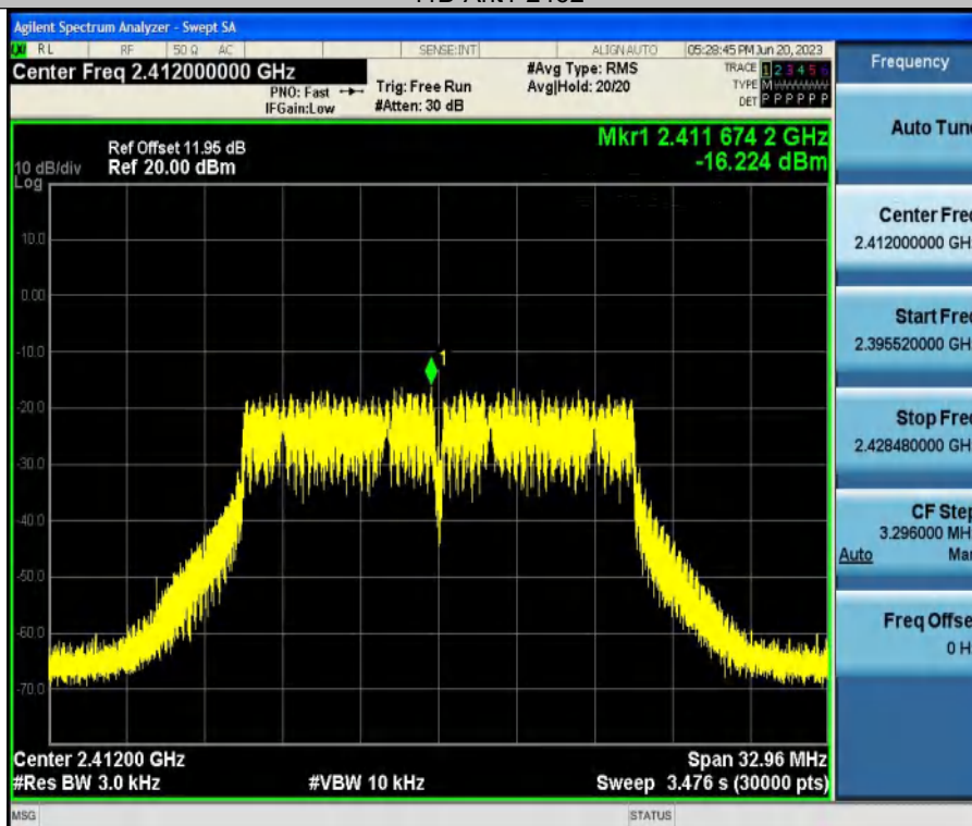
11G-Ant1-2412
