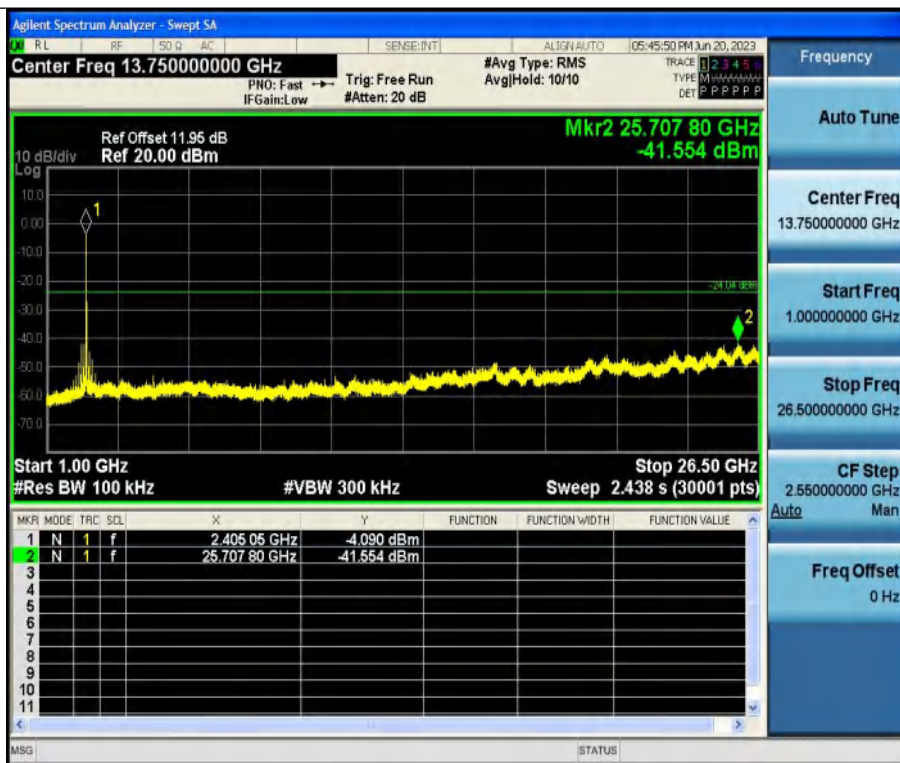
11N20SISO-Ant1-2412-1000~26500
