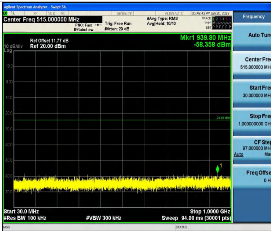
11N20SISO-Ant1-2437-30~1000
