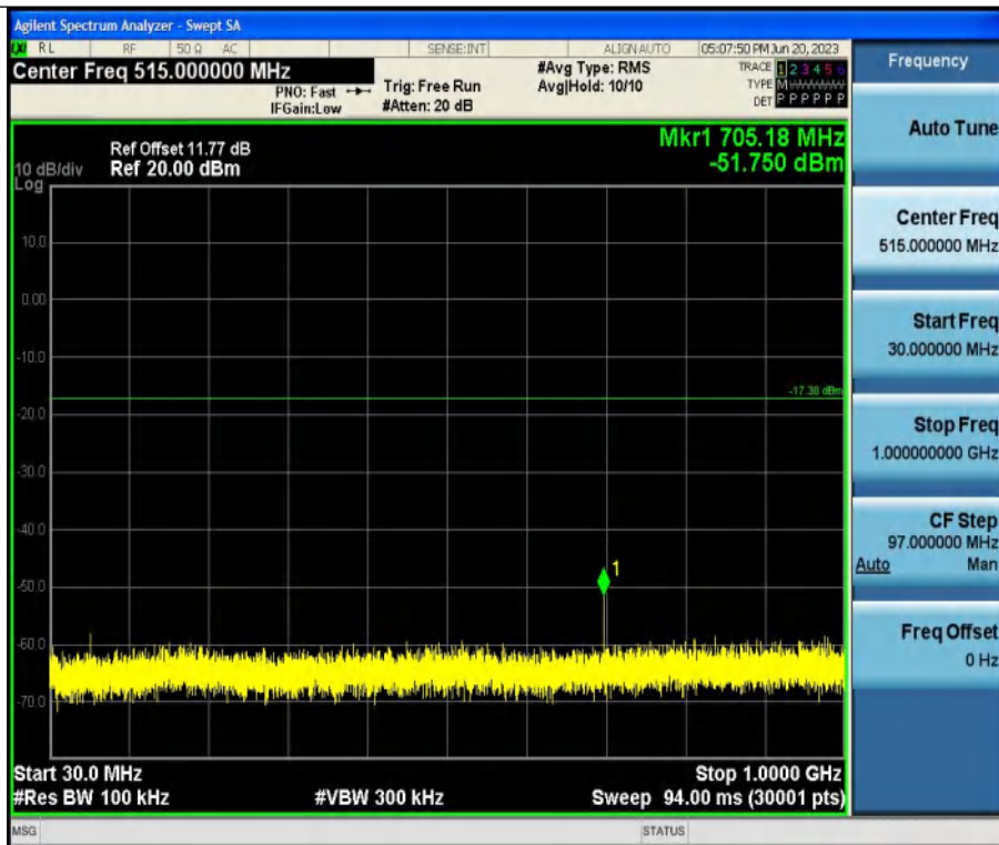
11B-Ant1-2437-30~1000
