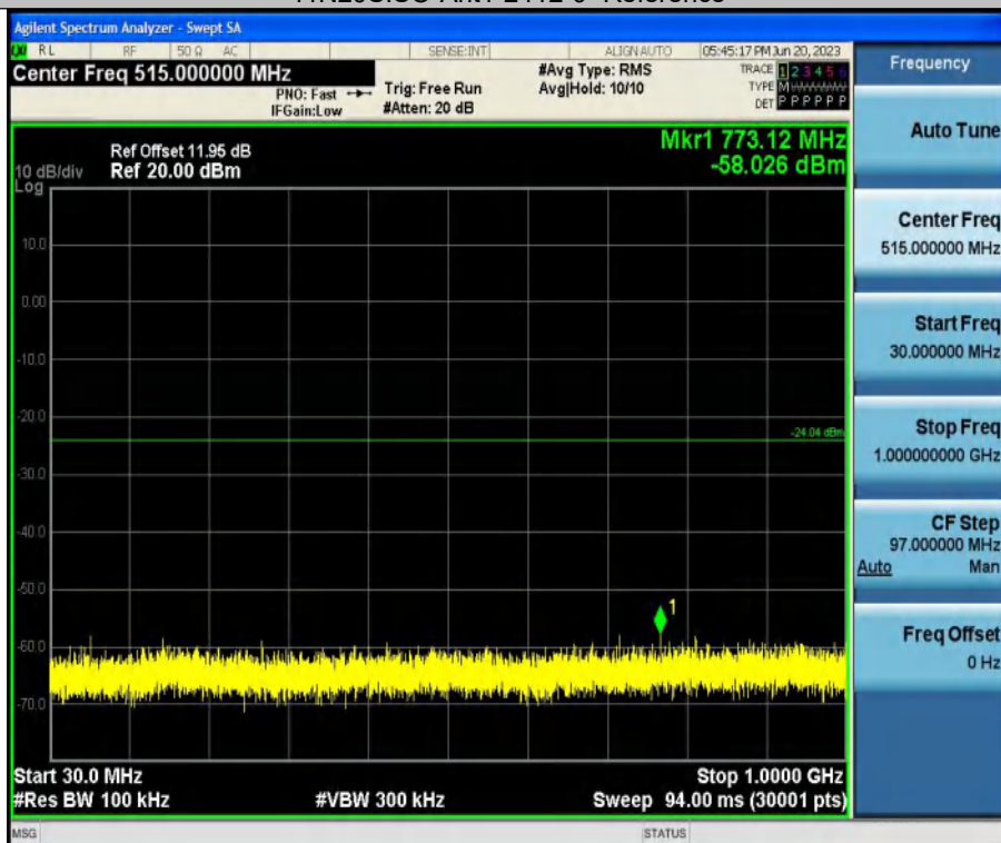
11N20SISO-Ant1-2412-30~1000
