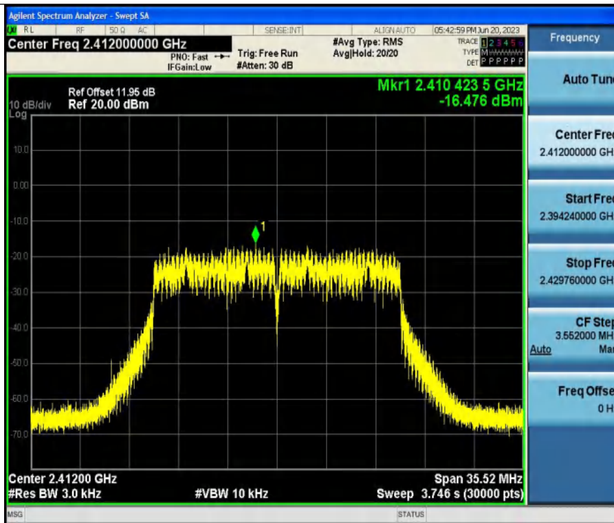
11N20SISO-Ant1-2412
