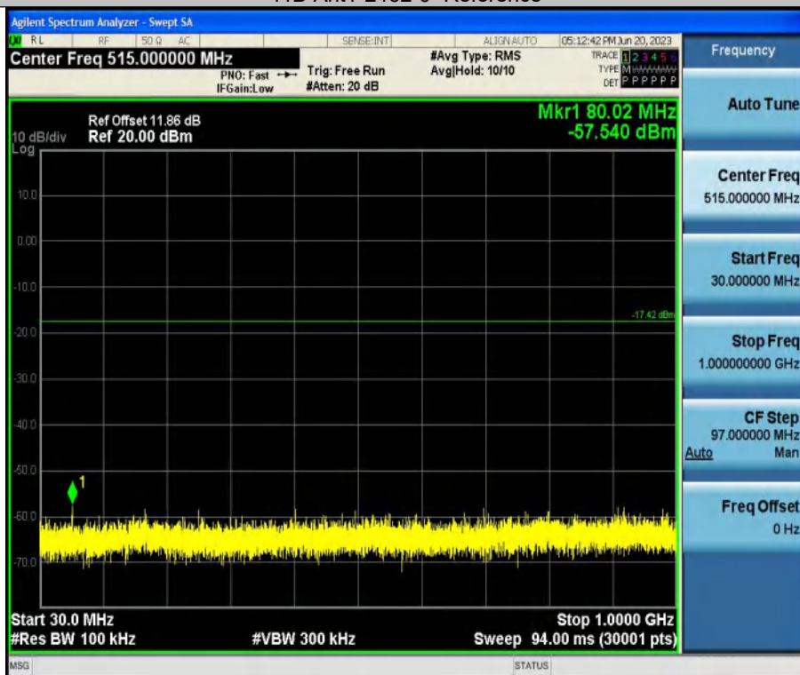
11B-Ant1-2462-30~1000
