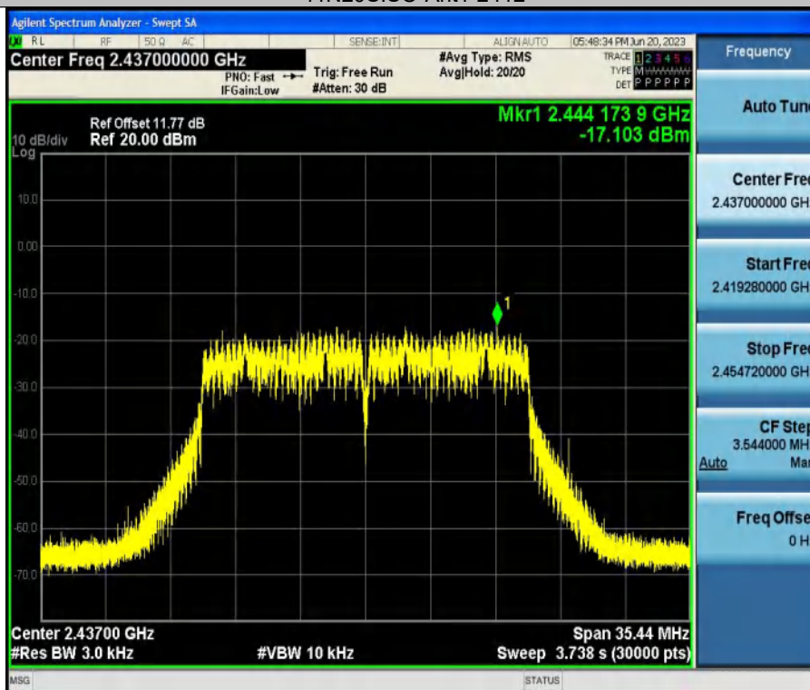
11N20SISO-Ant1-2437
