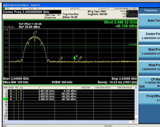
11B-Ant1-High-2462-4.10
