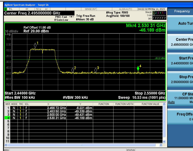
11N20SISO-Ant1-High-2462-6.22
