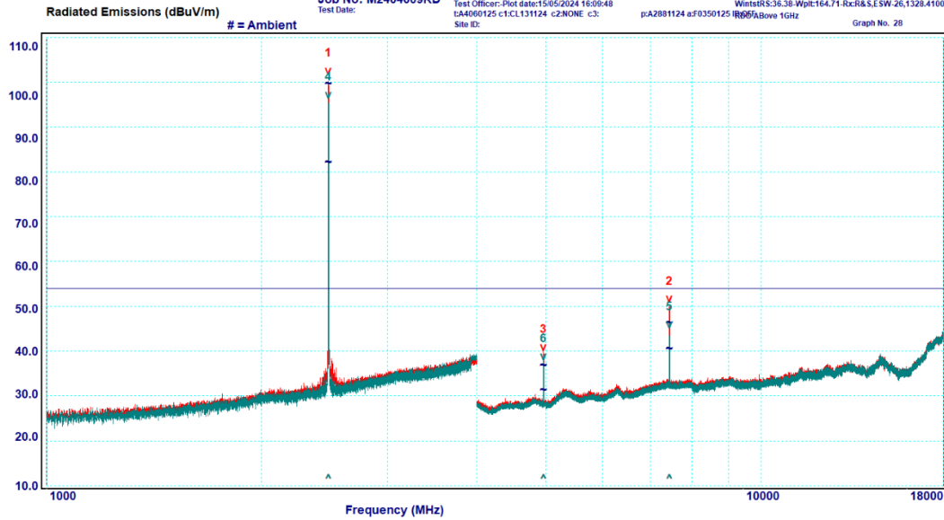
Graph 6-18: Transmitter Spurious Emissions, 1 – 18 GHz, 2480 MHz, Average
