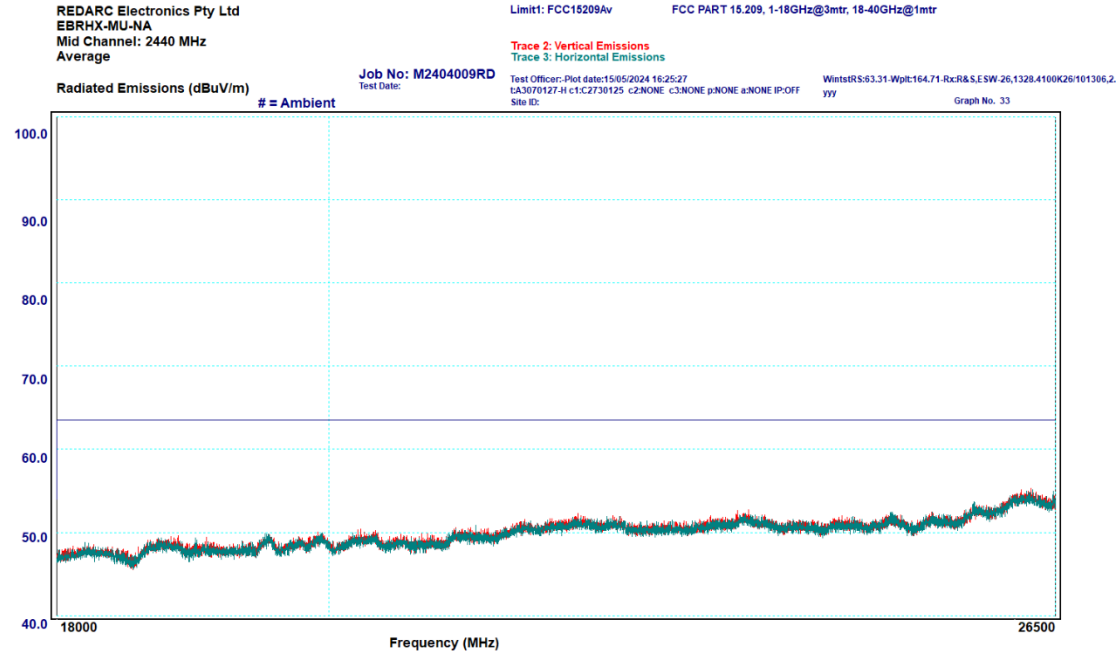
Graph 6-23: Transmitter Spurious Emissions, 18 – 26 GHz, 2440 MHz, Average
