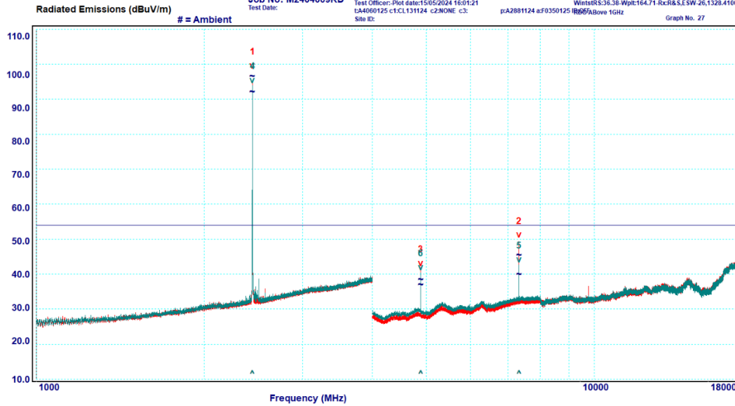
Graph 6-17: Transmitter Spurious Emissions, 1 – 18 GHz, 2440 MHz, Average
