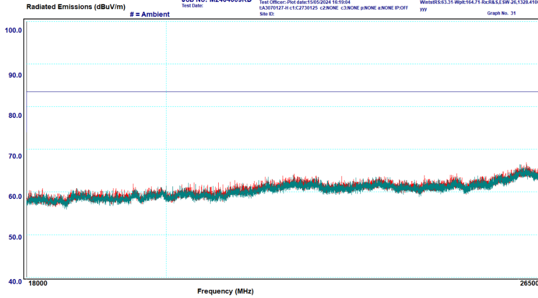
Graph 6-21: Transmitter Spurious Emissions, 18 – 26 GHz, 2480 MHz, Peak
