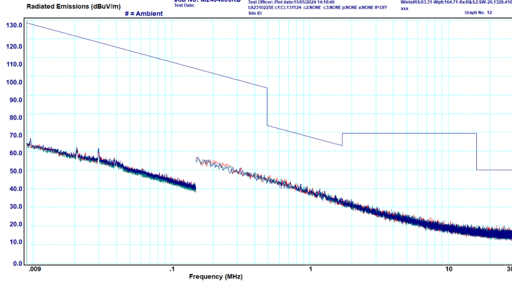
Graph 6-9: Transmitter Spurious Emissions, 9 kHz – 30 MHz, 2480 MHz
