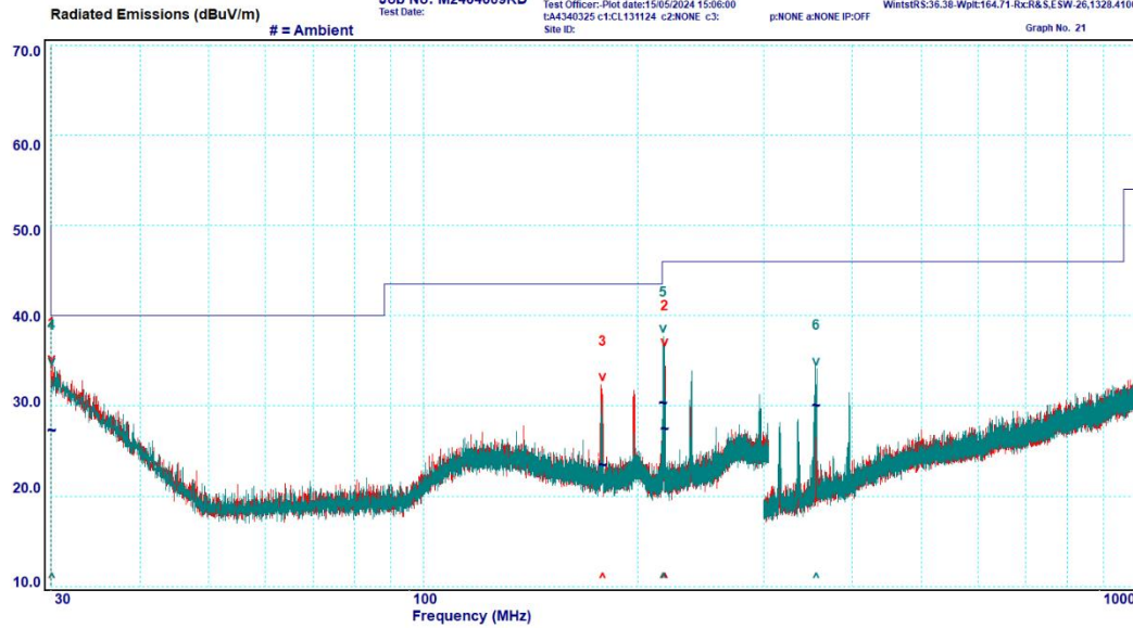
Graph 6-11: Transmitter Spurious Emissions, 30 – 1000 MHz, 2440 MHz
