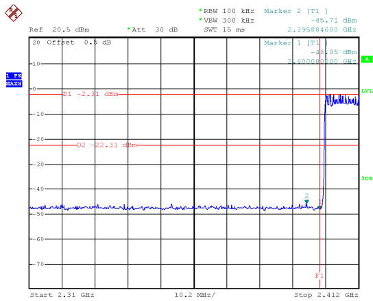
Hopping Band edge-left side
