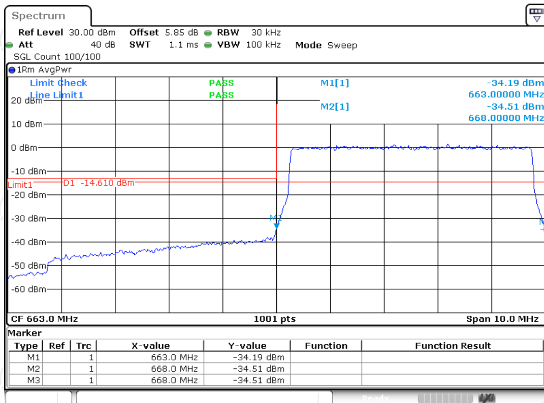
Band71 QPSK BW=5MHz Channel=133147 RB Size=25 Position=#0
