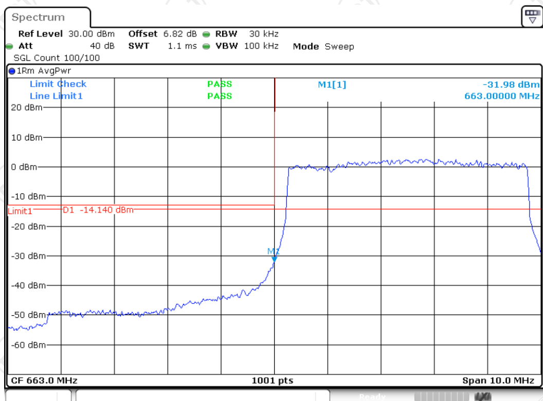
Band71 QPSK BW=5MHz Channel=133147 RB Size=25 Position=#0
