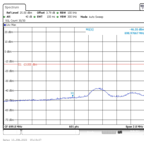
Band12-5MHz-16QAM-23035-1RB#24
