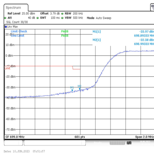
Band12-10MHz-QPSK-23060-50RB#0
