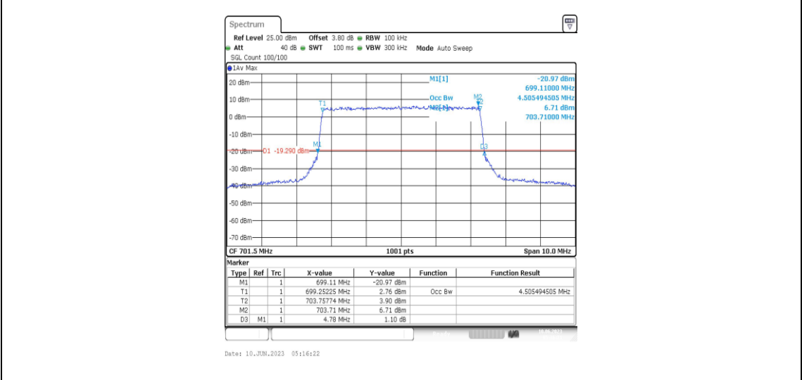
Band12-5MHz-16QAM-23035-25RB#0-4.505
