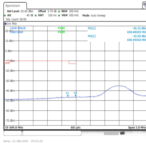
Band12-10MHz-QPSK-23060-1RB#49
