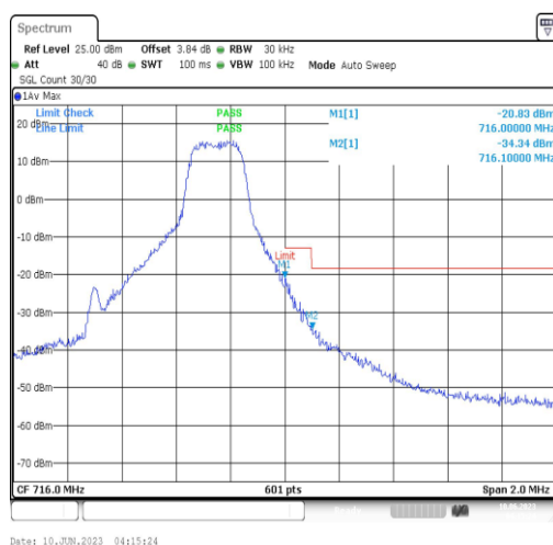
Band12-1.4MHz-16QAM-23173-1RB#5
