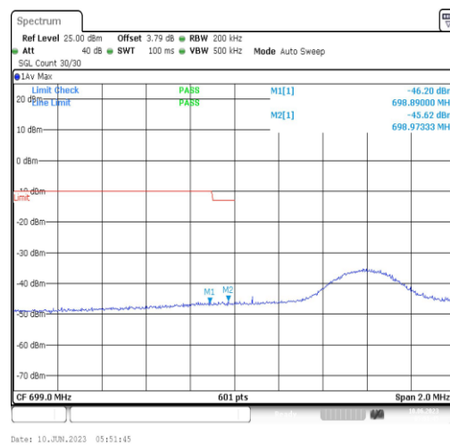
Band12-10MHz-16QAM-23060-1RB#49
