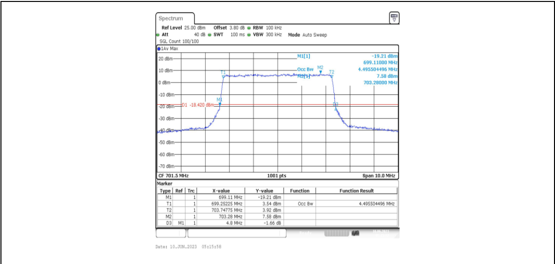
Band12-5MHz-QPSK-23035-25RB#0-4.496
