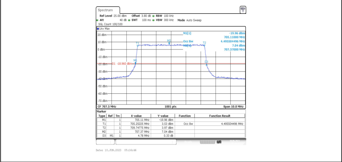
Band12-5MHz-QPSK-23095-25RB#0-4.496
