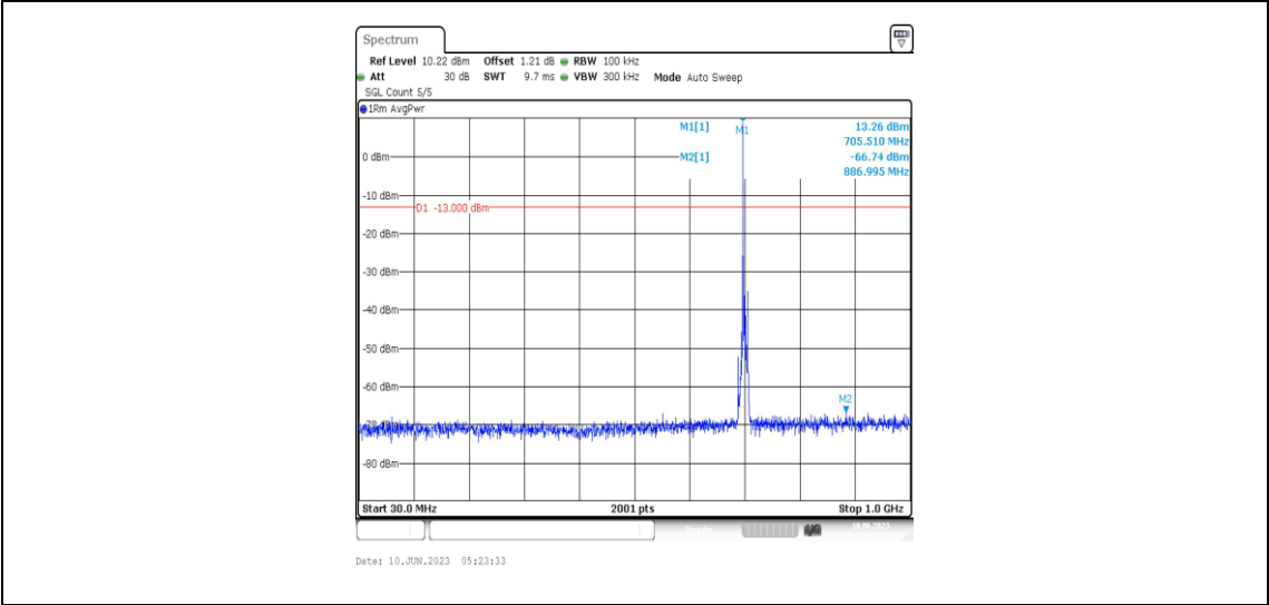
Band12-5MHz-QPSK-23095-1RB#0-Range3:30~1000MHz
