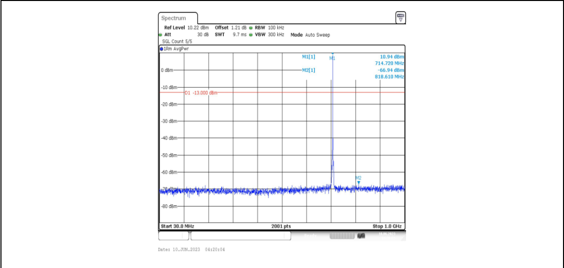
Band12-1.4MHz-QPSK-23173-1RB#0-Range3:30~1000MHz
