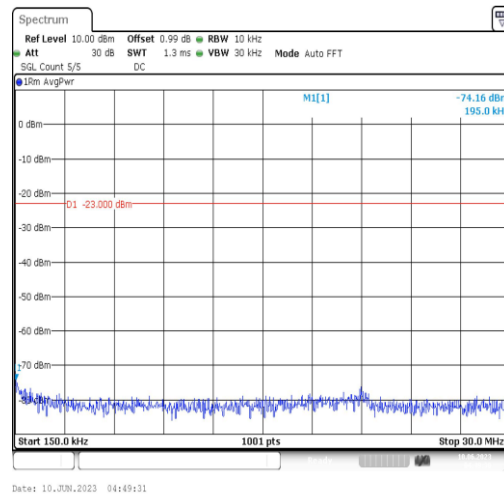
Band12-3MHz-16QAM-23025-1RB#0-Range2:0.15~30MHz
