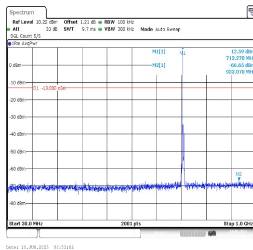
Band12-3MHz-16QAM-23165-1RB#0-Range3:30~1000MHz
