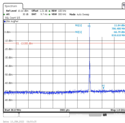
Band12-3MHz-QPSK-23095-1RB#0-Range3:30~1000MHz
