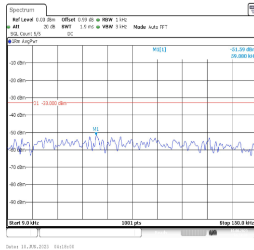
Band12-1.4MHz-QPSK-23095-1RB#0-Range1:0.009~0.15MHz
