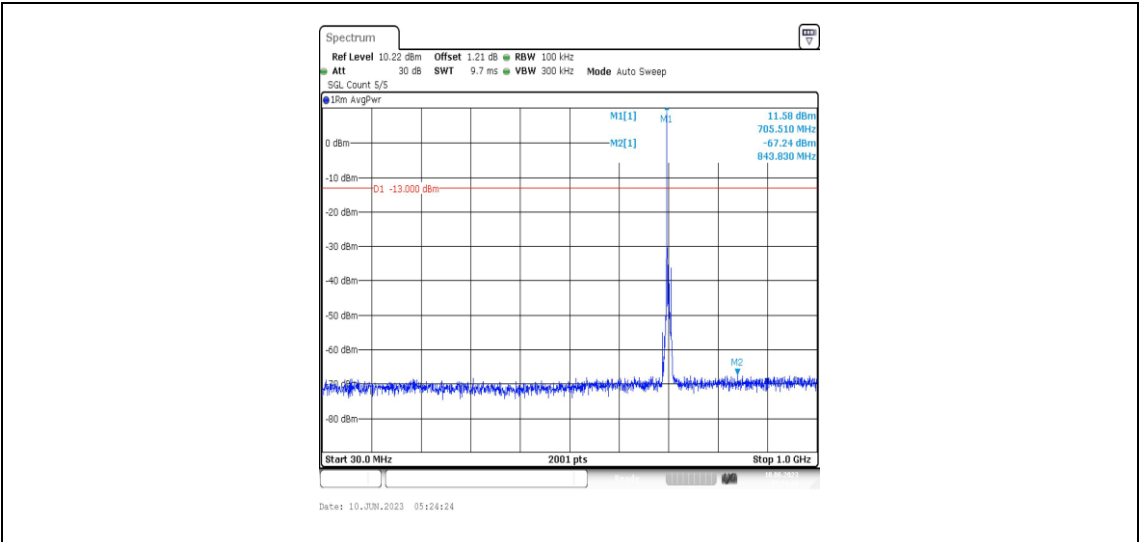
Band12-5MHz-16QAM-23095-1RB#0-Range3:30~1000MHz
