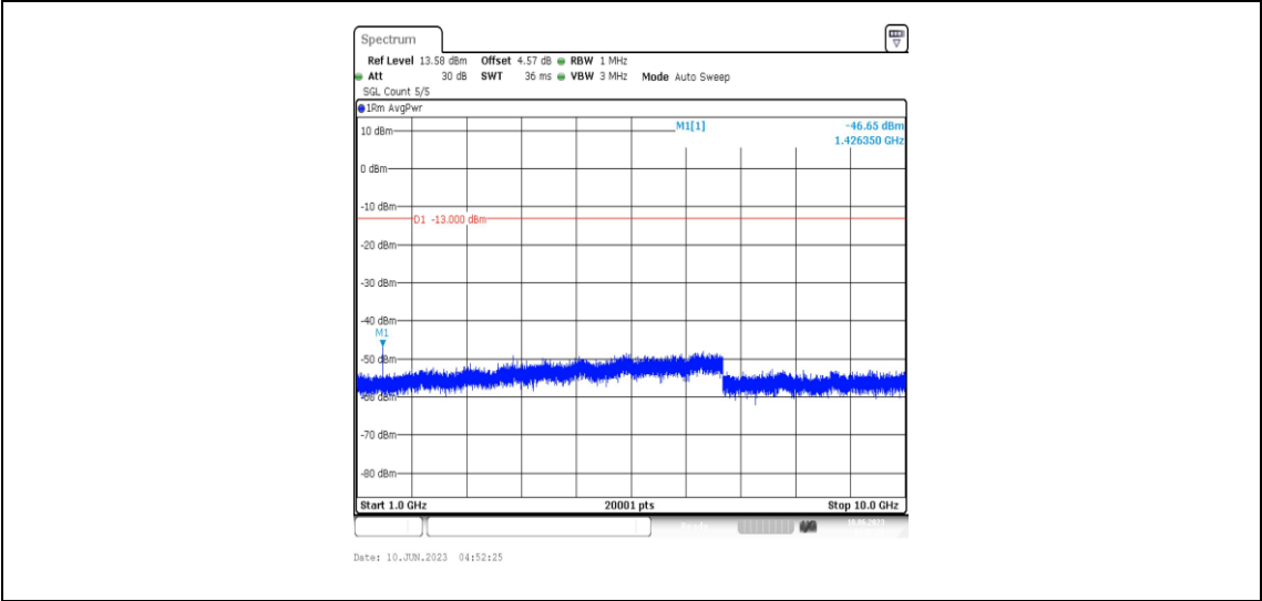
Band12-3MHz-QPSK-23165-1RB#0-Range4:1000~10000MHz
