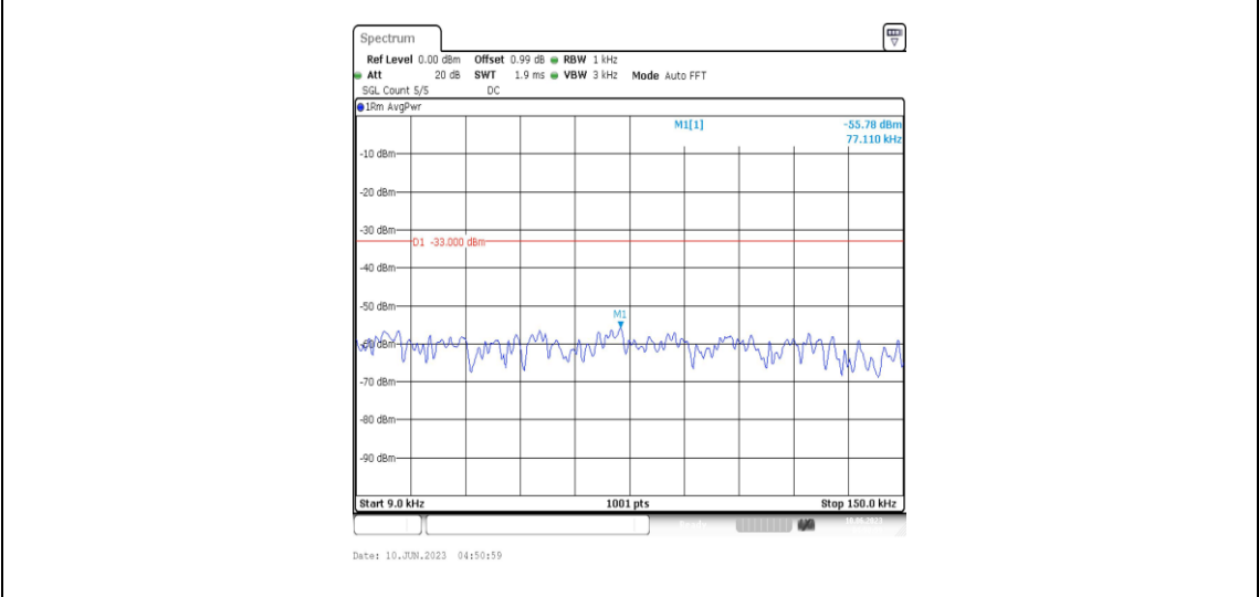
Band12-3MHz-16QAM-23095-1RB#0-Range1:0.009~0.15MHz
