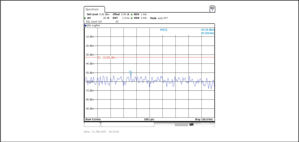
Band12-1.4MHz-QPSK-23173-1RB#0-Range1:0.009~0.15MHz
