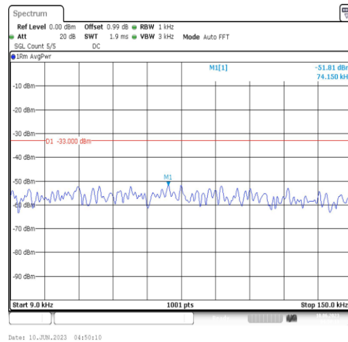
Band12-3MHz-QPSK-23095-1RB#0-Range1:0.009~0.15MHz
