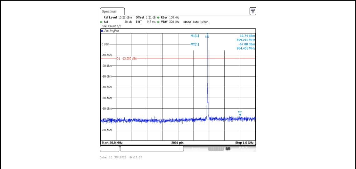
Band12-1.4MHz-16QAM-23017-1RB#0-Range3:30~1000MHz
