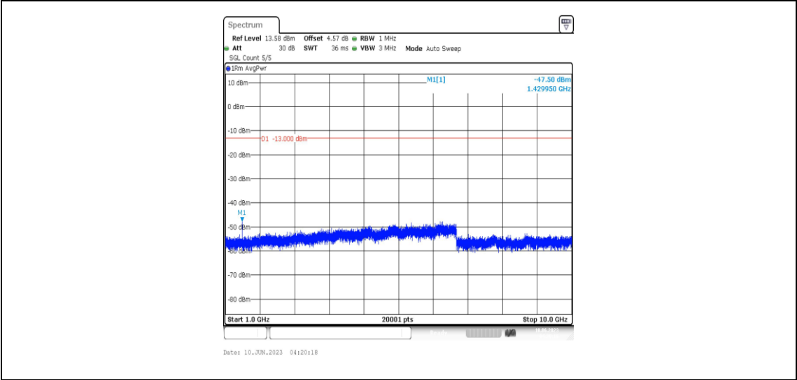
Band12-1.4MHz-QPSK-23173-1RB#0-Range4:1000~10000MHz
