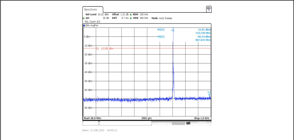
Band12-3MHz-QPSK-23165-1RB#0-Range3:30~1000MHz
