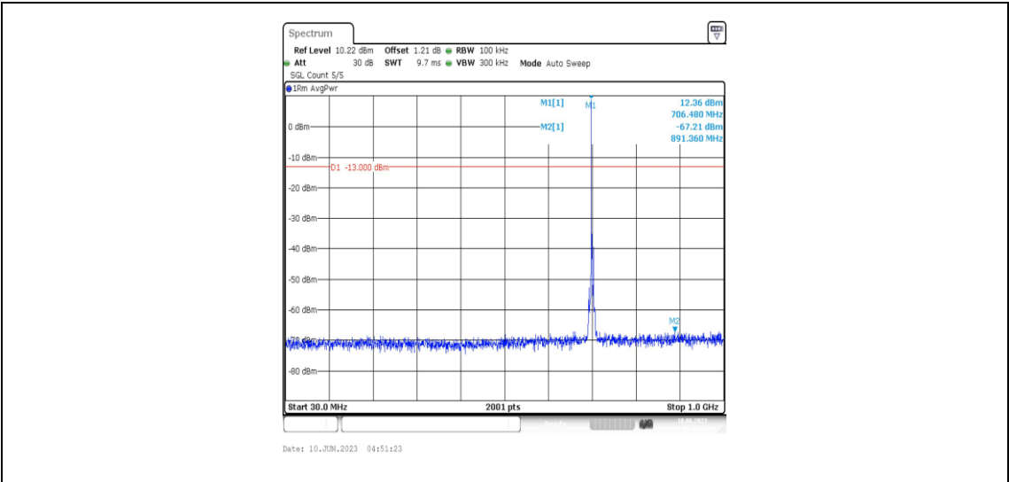
Band12-3MHz-16QAM-23095-1RB#0-Range3:30~1000MHz
