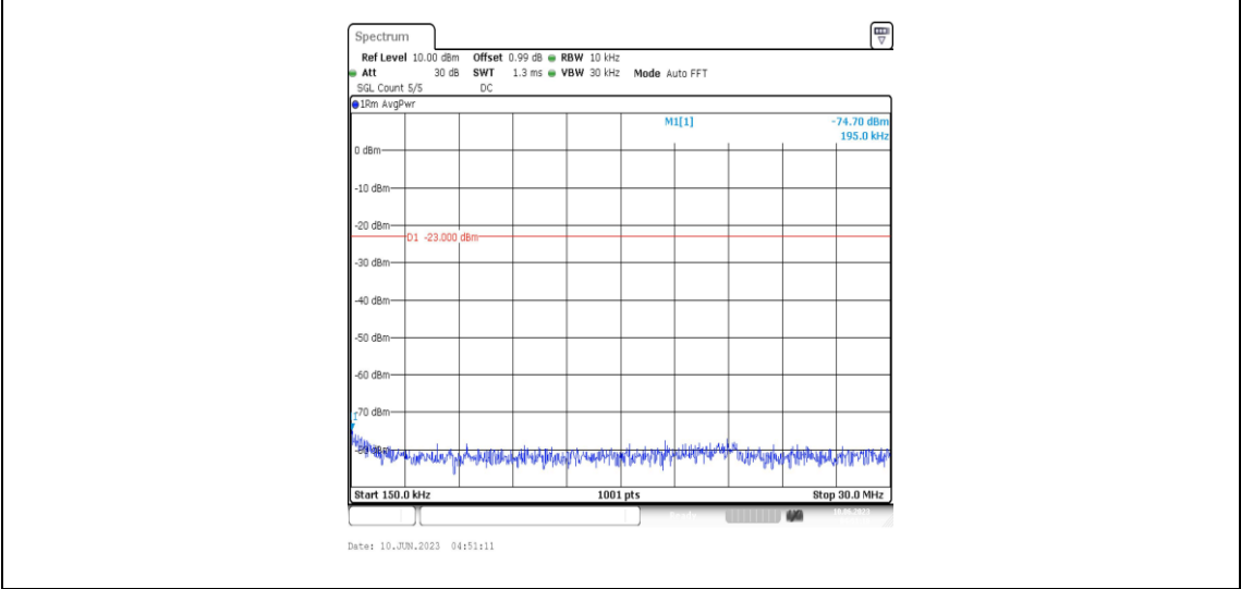
Band12-3MHz-16QAM-23095-1RB#0-Range2:0.15~30MHz
