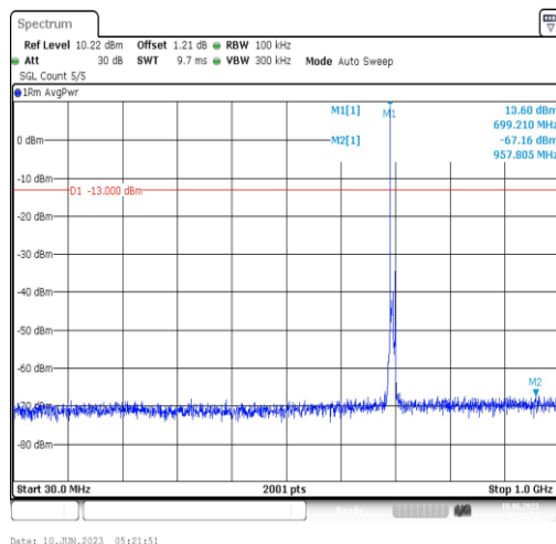
Band12-5MHz-QPSK-23035-1RB#0-Range3:30~1000MHz
