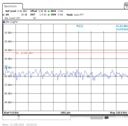
Band12-5MHz-16QAM-23035-1RB#0-Range1:0.009~0.15MHz
