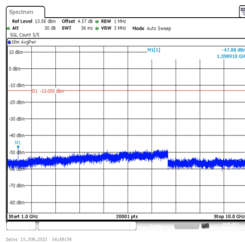
Band12-3MHz-16QAM-23025-1RB#0-Range4:1000~10000MHz
