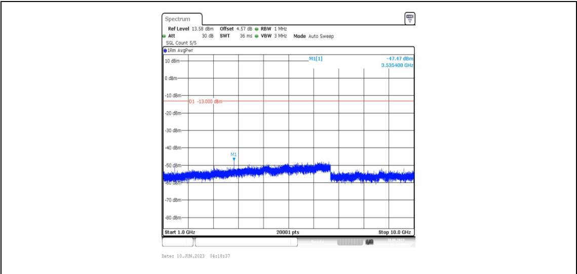
Band12-1.4MHz-QPSK-23095-1RB#0-Range4:1000~10000MHz
