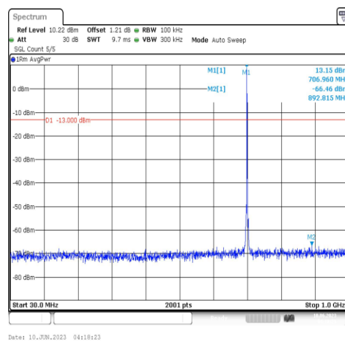
Band12-1.4MHz-QPSK-23095-1RB#0-Range3:30~1000MHz
