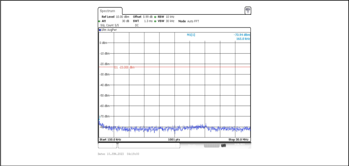
Band12-1.4MHz-16QAM-23095-1RB#0-Range2:0.15~30MHz
