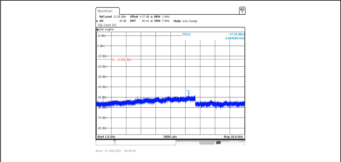
Band12-3MHz-QPSK-23025-1RB#0-Range4:1000~10000MHz
