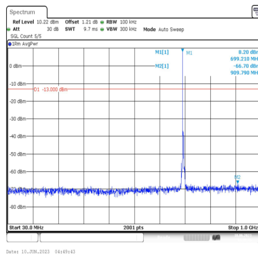
Band12-3MHz-16QAM-23025-1RB#0-Range3:30~1000MHz
