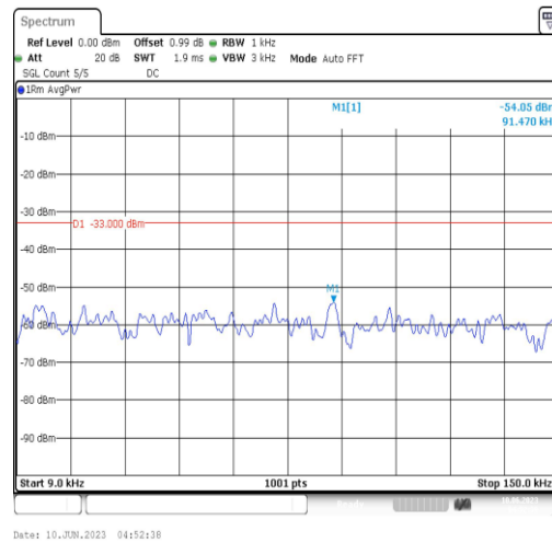
Band12-3MHz-16QAM-23165-1RB#0-Range1:0.009~0.15MHz
