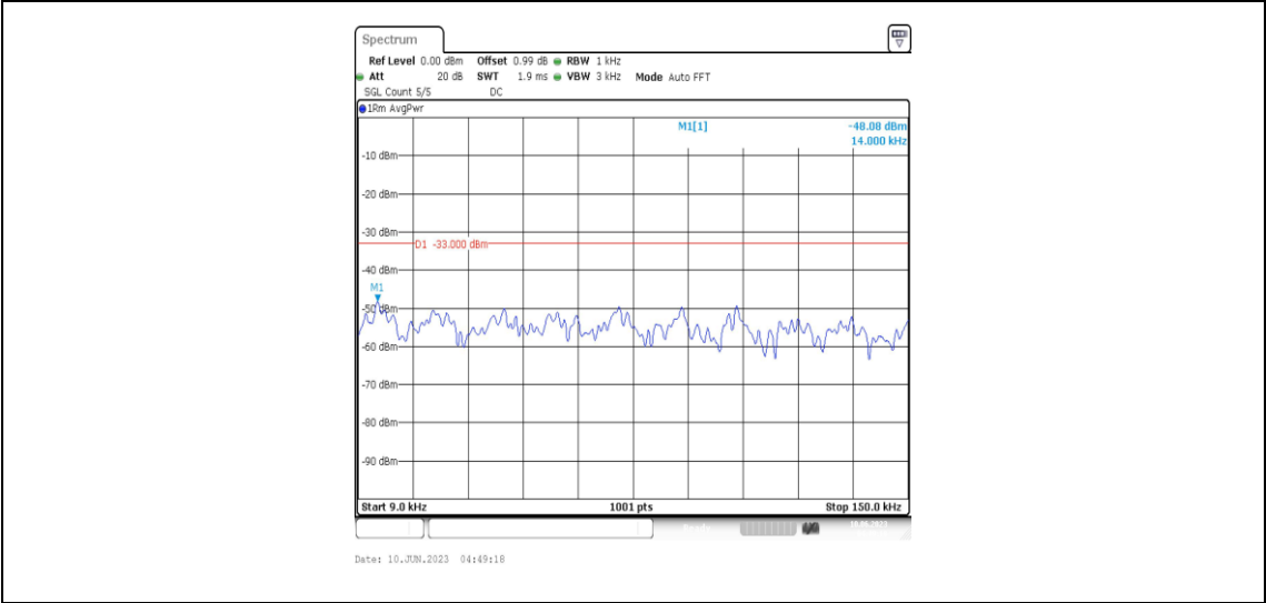
Band12-3MHz-16QAM-23025-1RB#0-Range1:0.009~0.15MHz
