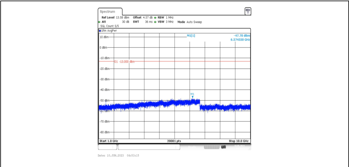
Band12-3MHz-16QAM-23165-1RB#0-Range4:1000~10000MHz
