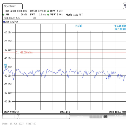
Band12-1.4MHz-16QAM-23017-1RB#0-Range1:0.009~0.15MHz
