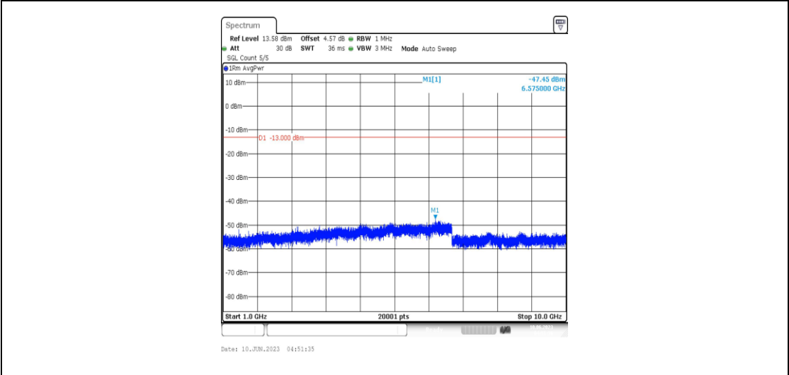
Band12-3MHz-16QAM-23095-1RB#0-Range4:1000~10000MHz
