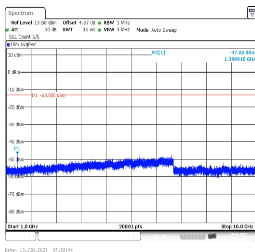
Band12-5MHz-QPSK-23035-1RB#0-Range4:1000~10000MHz
