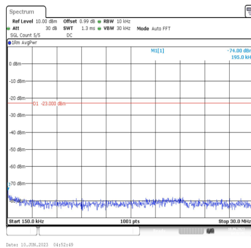
Band12-3MHz-16QAM-23165-1RB#0-Range2:0.15~30MHz
