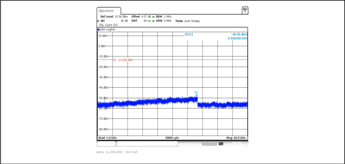
Band12-1.4MHz-16QAM-23017-1RB#0-Range4:1000~10000MHz
