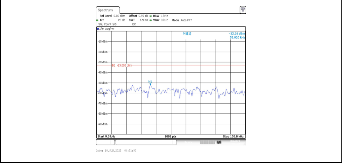
Band12-3MHz-QPSK-23165-1RB#0-Range1:0.009~0.15MHz
