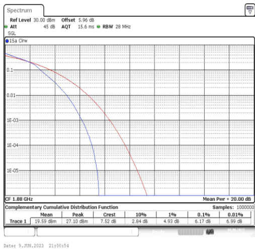
Band2-5MHz-16QAM-18900-25RB#0
