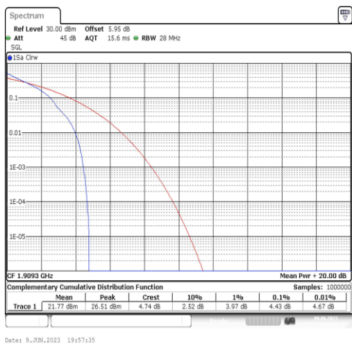
Band2-1.4MHz-QPSK-19193-1RB#0
