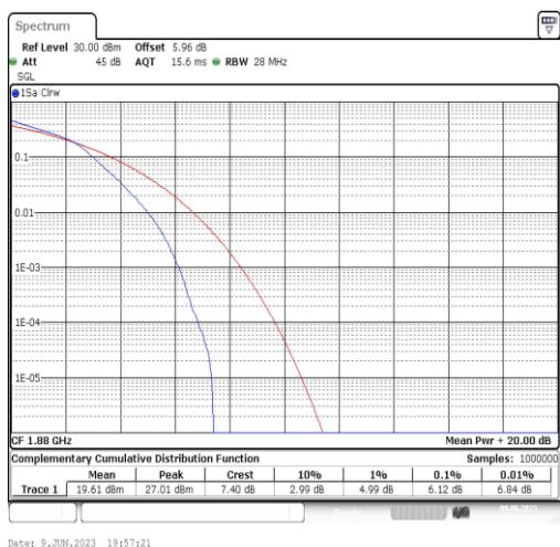
Band2-1.4MHz-16QAM-18900-6RB#0
