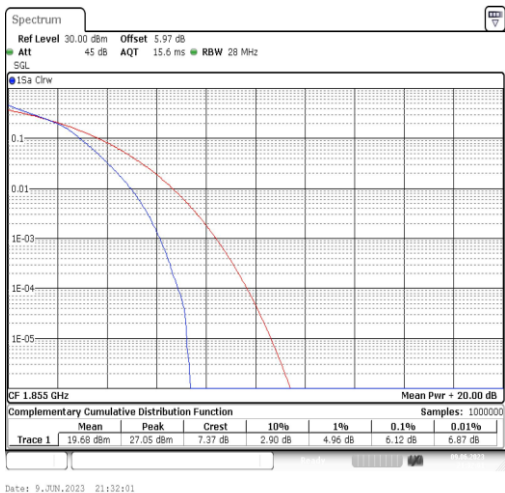
Band2-10MHz-16QAM-18650-50RB#0
