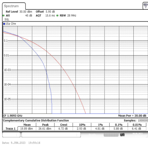
Band2-1.4MHz-16QAM-19193-6RB#0
