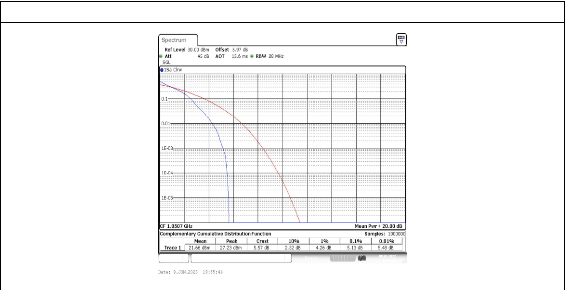
Band2-1.4MHz-QPSK-18607-1RB#0
