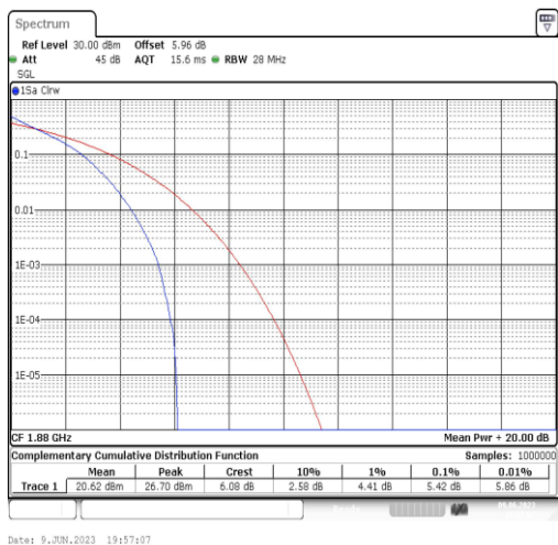
Band2-1.4MHz-QPSK-18900-6RB#0
