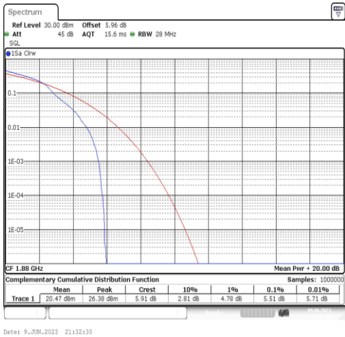
Band2-10MHz-16QAM-18900-1RB#0
