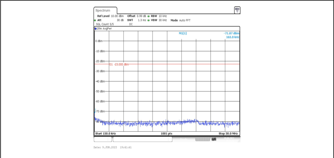
Band2-1.4MHz-16QAM-18607-1RB#0-Range2:0.15~30MHz
