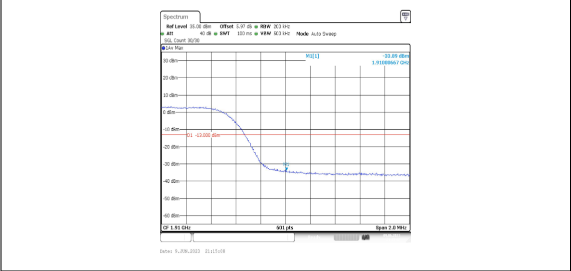
Band2-10MHz-16QAM-19150-50RB#0
