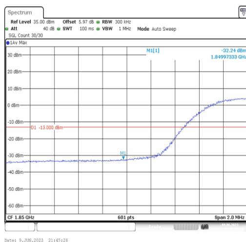
Band2-15MHz-QPSK-18675-75RB#0
