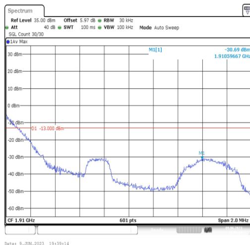
Band2-1.4MHz-QPSK-19193-1RB#0
