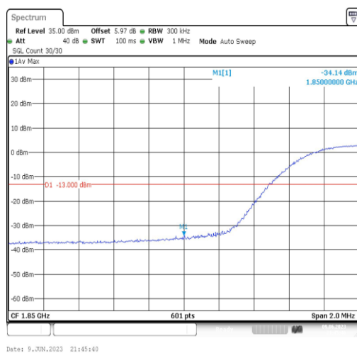
Band2-15MHz-16QAM-18675-75RB#0
