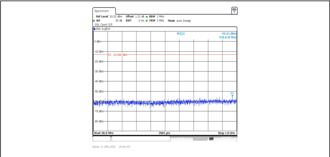
Band2-1.4MHz-16QAM-18607-1RB#0-Range3:30~1000MHz
