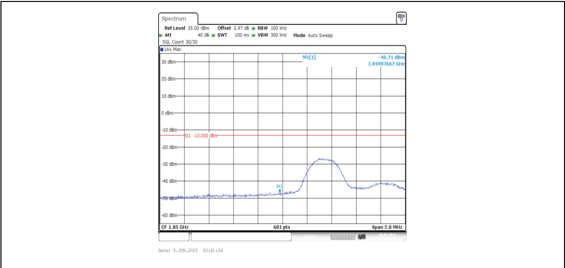
Band2-5MHz-16QAM-18625-1RB#24
