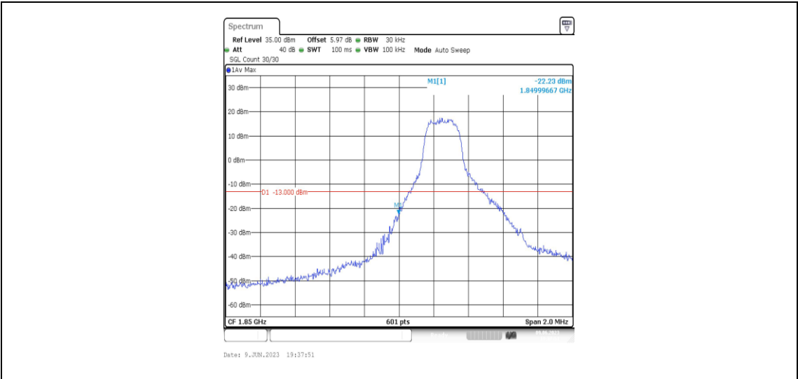
Band2-1.4MHz-QPSK-18607-1RB#0
