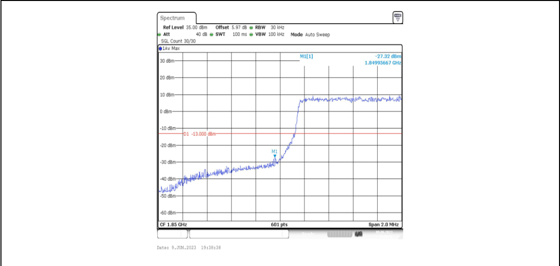
Band2-1.4MHz-QPSK-18607-6RB#0
