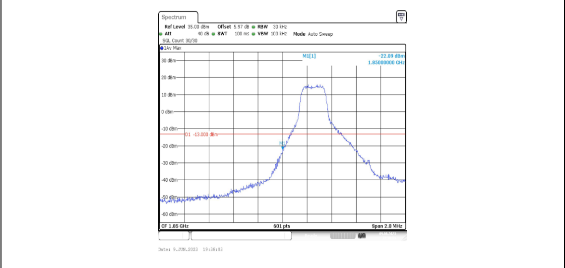
Band2-1.4MHz-16QAM-18607-1RB#0
