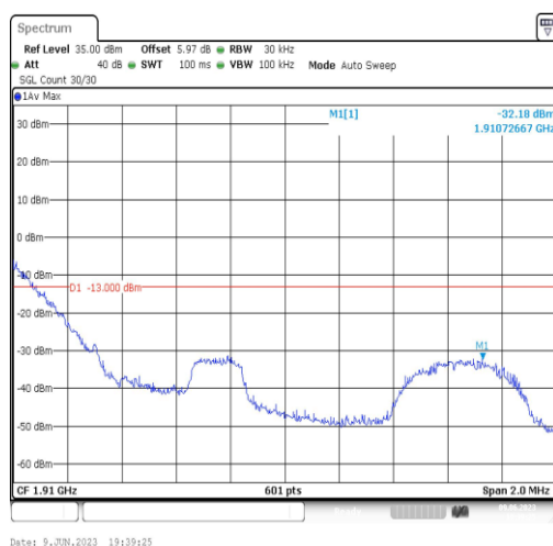
Band2-1.4MHz-16QAM-19193-1RB#0
