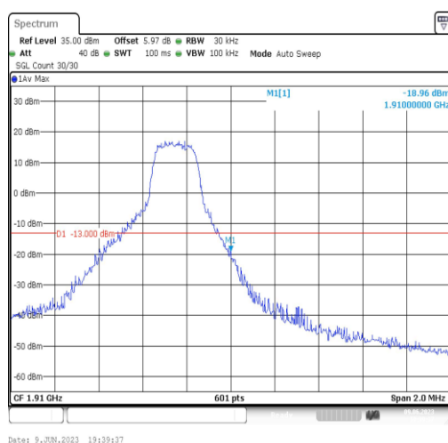
Band2-1.4MHz-QPSK-19193-1RB#5
