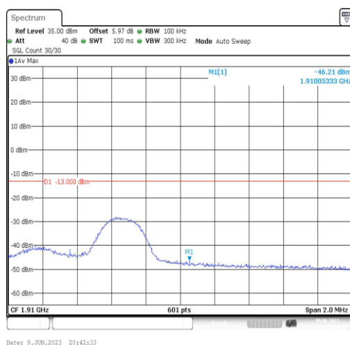
Band2-5MHz-16QAM-19175-1RB#0
