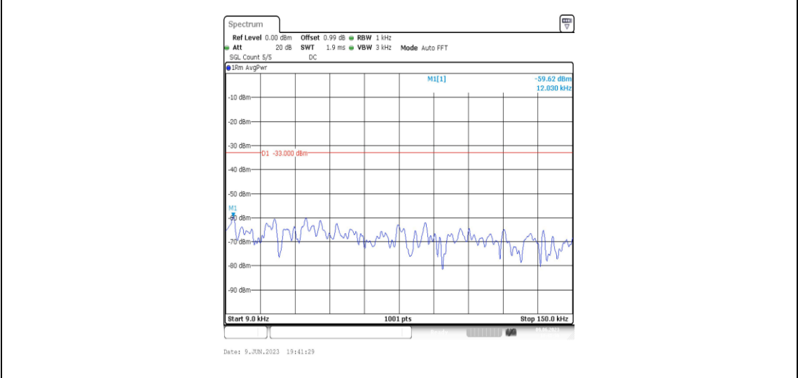
Band2-1.4MHz-16QAM-18607-1RB#0-Range1:0.009~0.15MHz
