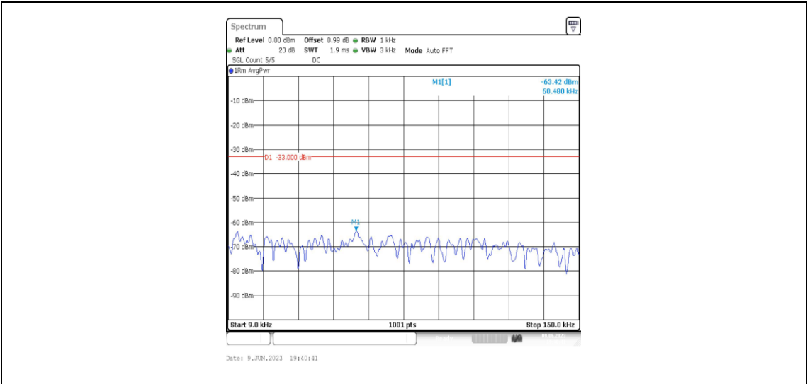
Band2-1.4MHz-QPSK-18607-1RB#0-Range1:0.009~0.15MHz
