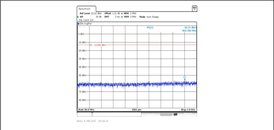
Band2-3MHz-16QAM-19185-1RB#0-Range3:30~1000MHz
