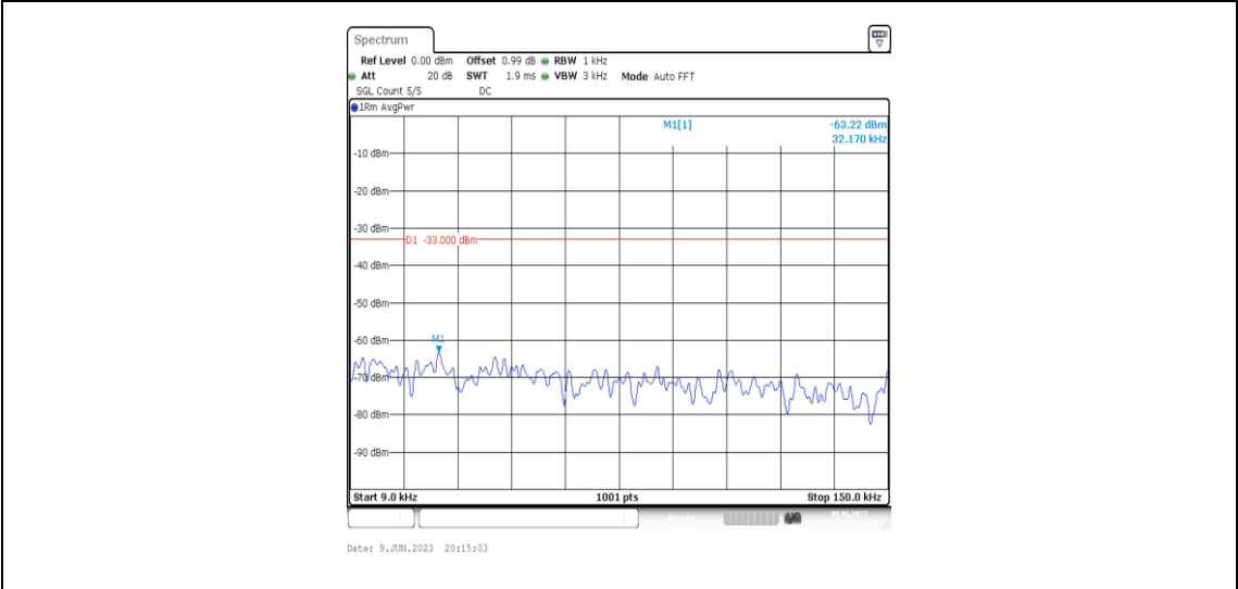
Band2-3MHz-QPSK-19185-1RB#0-Range1:0.009~0.15MHz
