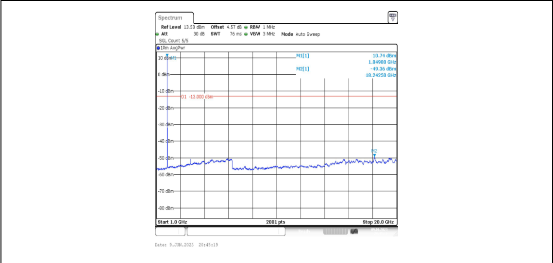
Band2-5MHz-16QAM-18625-1RB#0-Range4:1000~20000MHz
