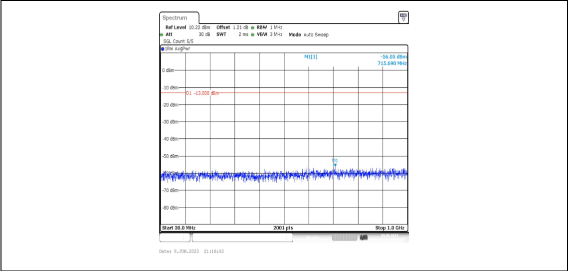
Band2-10MHz-QPSK-18650-1RB#0-Range3:30~1000MHz
