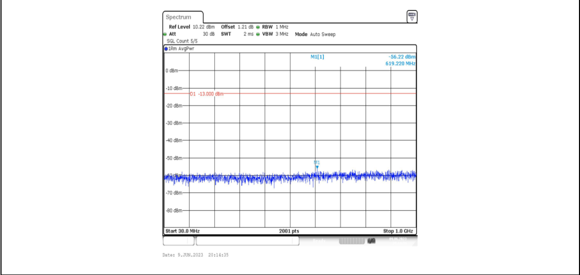
Band2-3MHz-16QAM-18900-1RB#0-Range3:30~1000MHz
