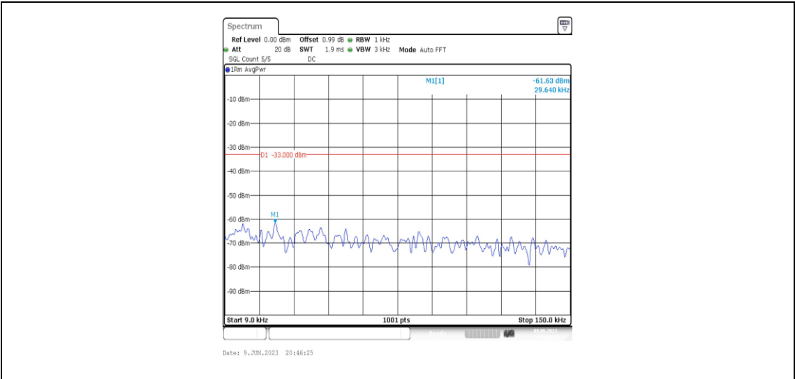
Band2-5MHz-16QAM-18900-1RB#0-Range1:0.009~0.15MHz
