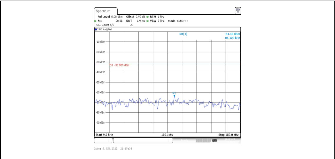
Band2-10MHz-QPSK-18650-1RB#0-Range1:0.009~0.15MHz
