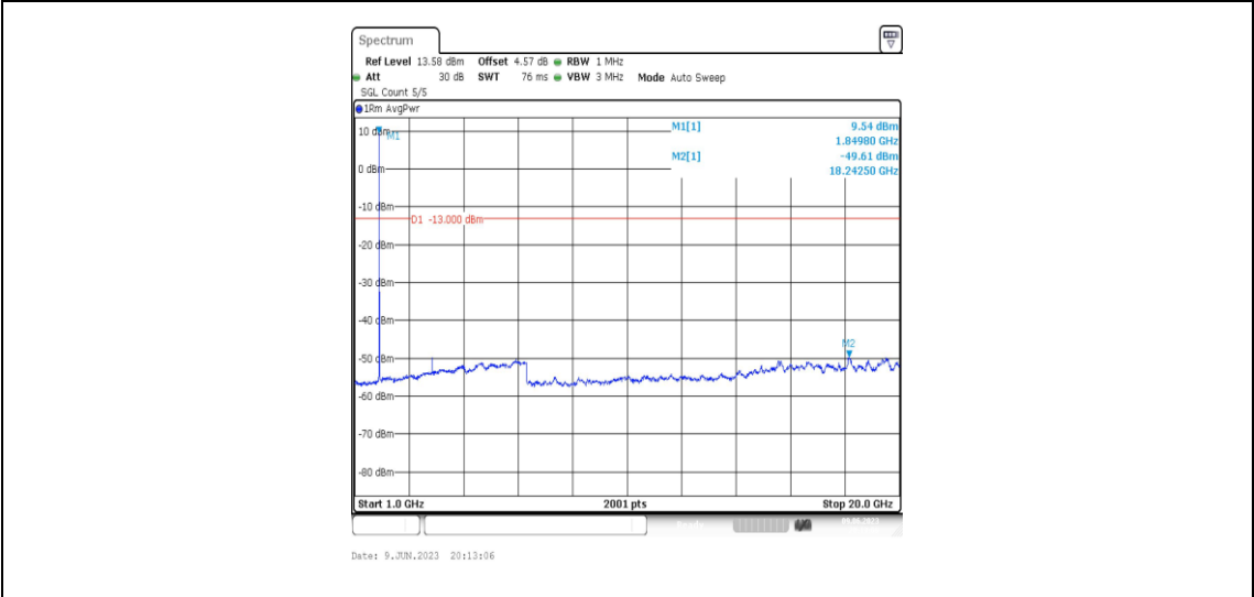
Band2-3MHz-16QAM-18615-1RB#0-Range4:1000~20000MHz
