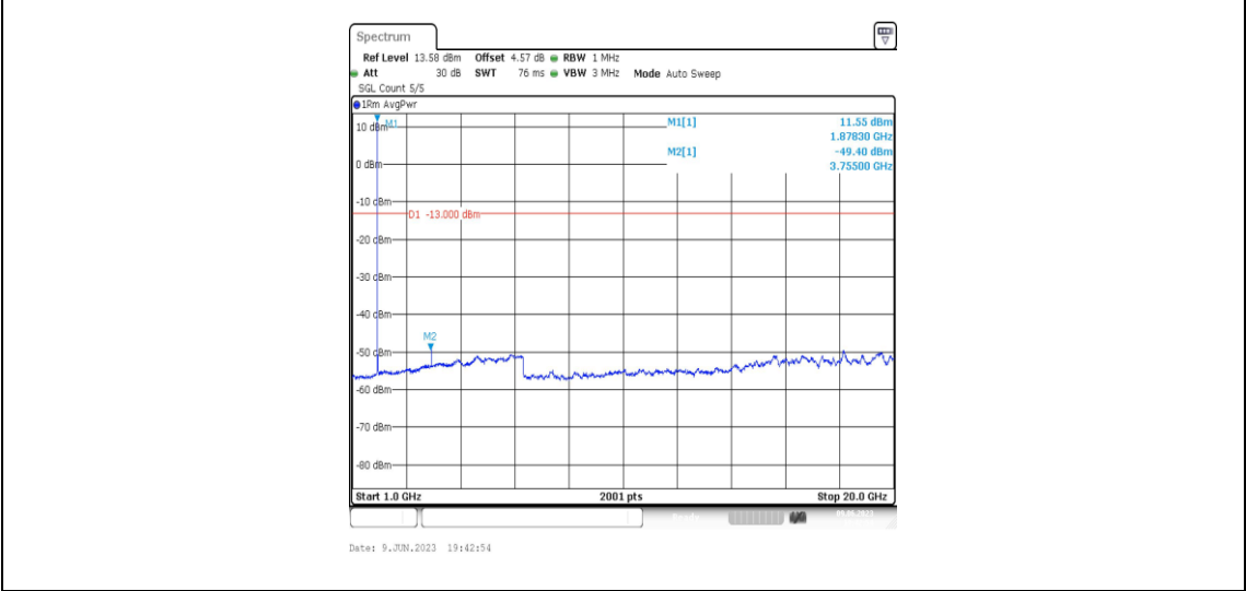
Band2-1.4MHz-QPSK-18900-1RB#0-Range4:1000~20000MHz
