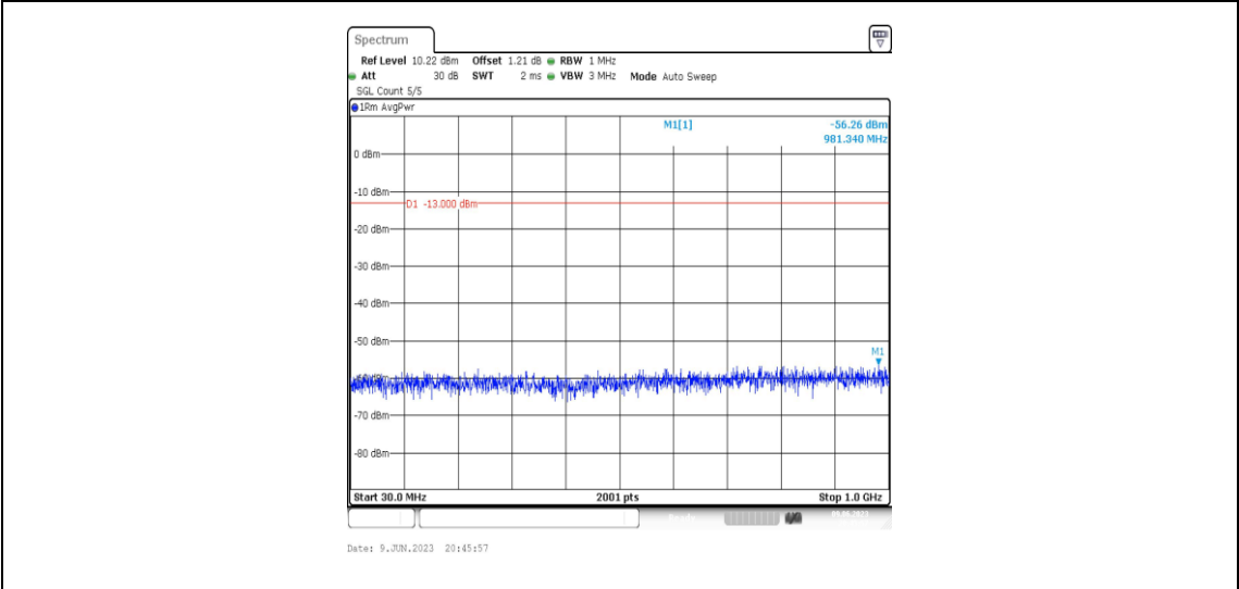
Band2-5MHz-QPSK-18900-1RB#0-Range3:30~1000MHz
