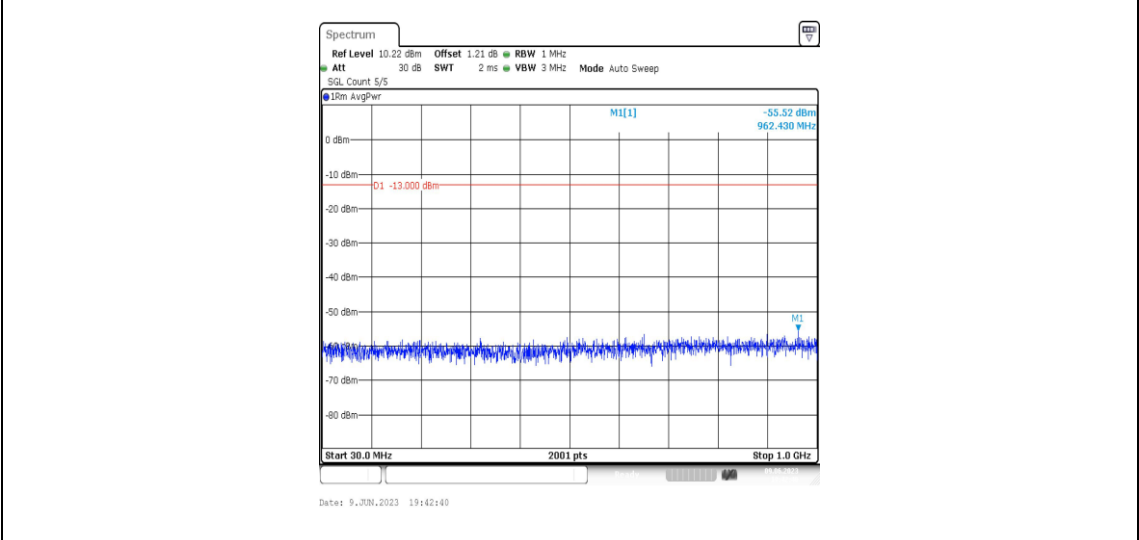
Band2-1.4MHz-QPSK-18900-1RB#0-Range3:30~1000MHz
