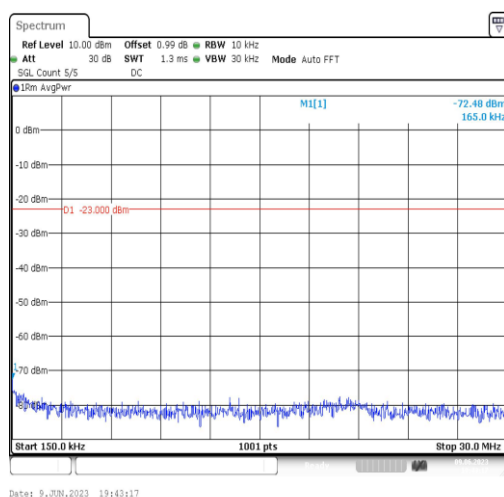
Band2-1.4MHz-16QAM-18900-1RB#0-Range2:0.15~30MHz
