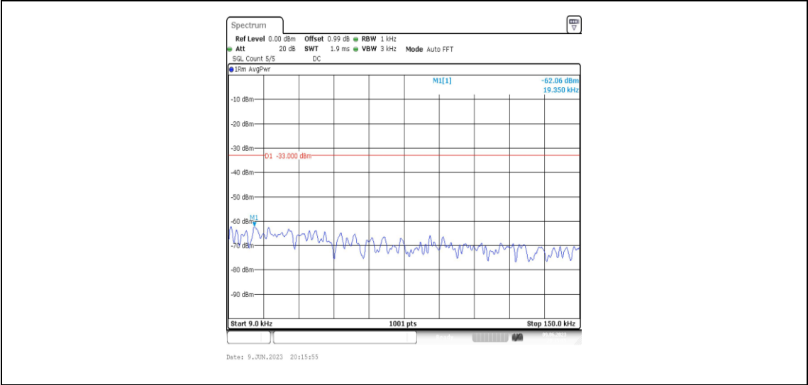
Band2-3MHz-16QAM-19185-1RB#0-Range1:0.009~0.15MHz
