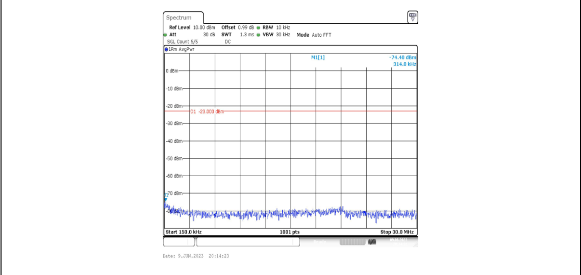
Band2-3MHz-16QAM-18900-1RB#0-Range2:0.15~30MHz
