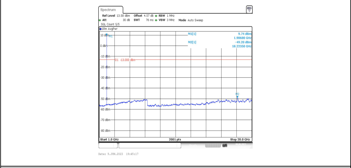
Band2-1.4MHz-16QAM-19193-1RB#0-Range4:1000~20000MHz
