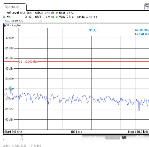
Band2-1.4MHz-16QAM-18900-1RB#0-Range1:0.009~0.15MHz
