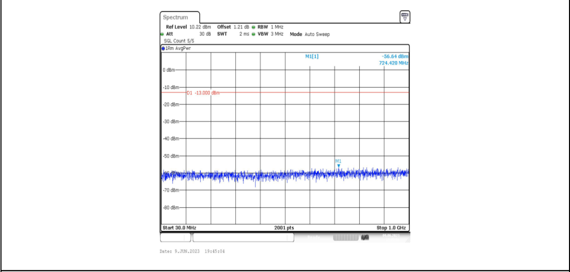
Band2-1.4MHz-16QAM-19193-1RB#0-Range3:30~1000MHz
