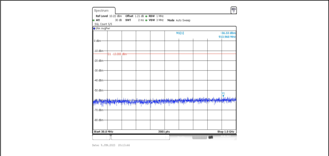
Band2-3MHz-QPSK-18900-1RB#0-Range3:30~1000MHz
