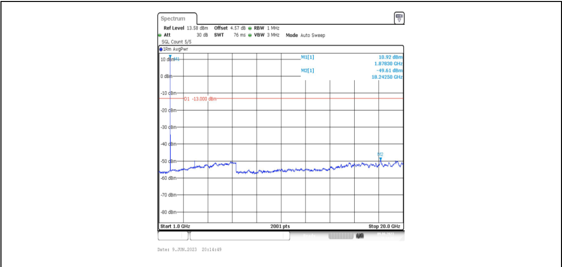
Band2-3MHz-16QAM-18900-1RB#0-Range4:1000~20000MHz
