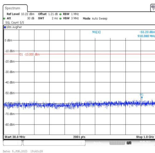
Band2-1.4MHz-16QAM-18900-1RB#0-Range3:30~1000MHz
