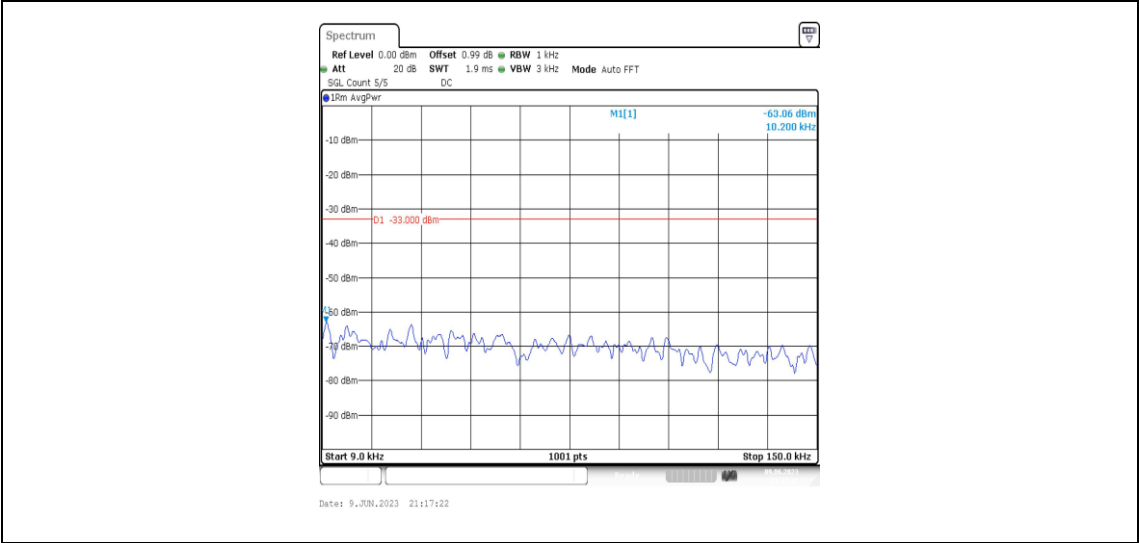
Band2-10MHz-QPSK-18900-1RB#0-Range1:0.009~0.15MHz
