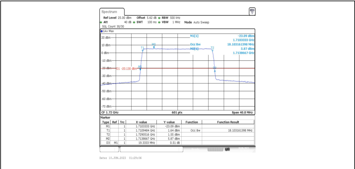
Band4-20MHz-QPSK-20050-100RB#0-18.103
