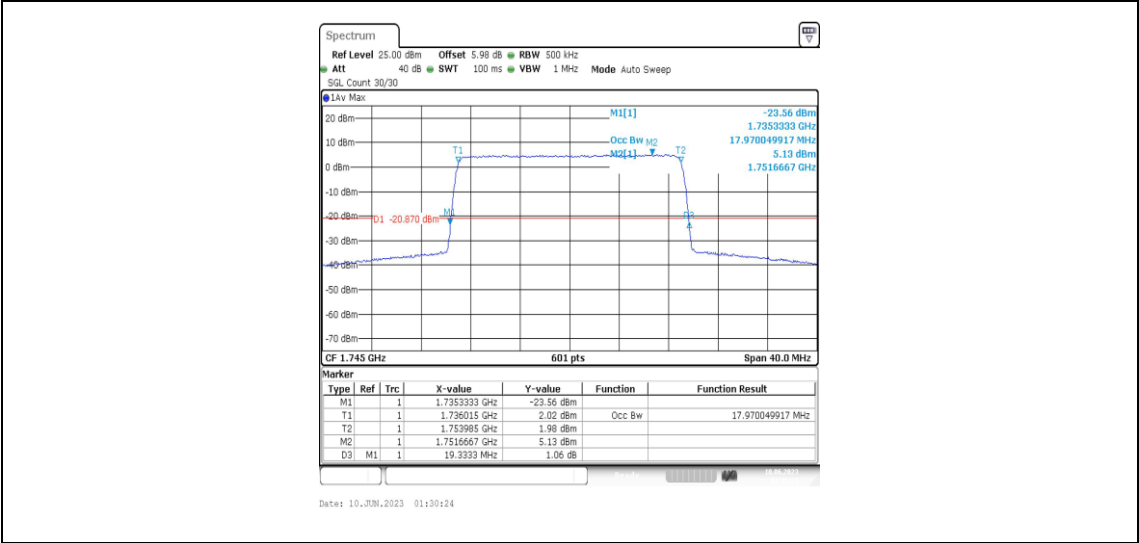
Band4-20MHz-16QAM-20300-100RB#0-17.97
