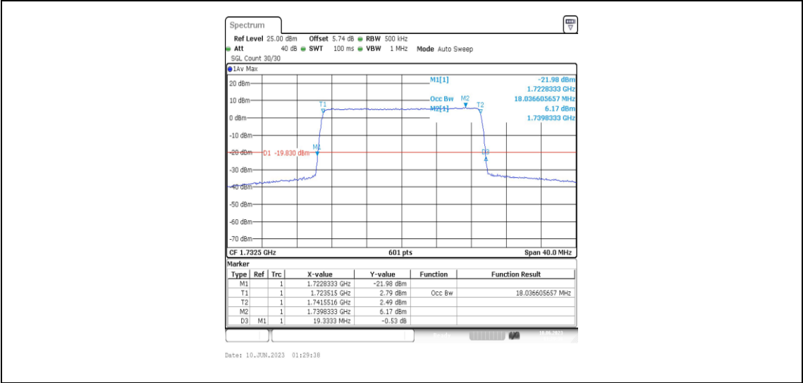
Band4-20MHz-QPSK-20175-100RB#0-18.037
