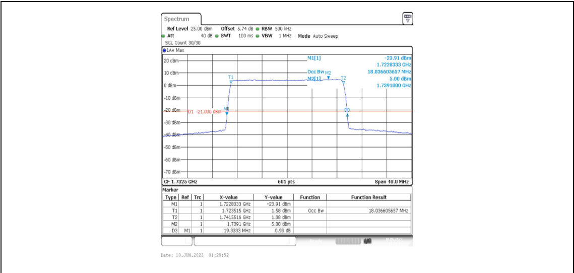
Band4-20MHz-16QAM-20175-100RB#0-18.037
