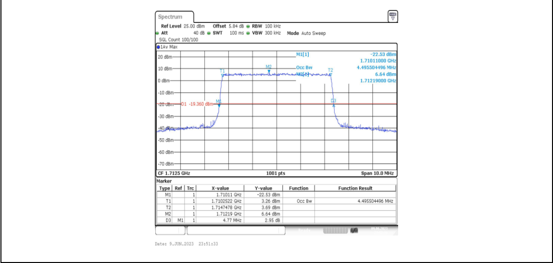
Band4-5MHz-16QAM-19975-25RB#0-4.496
