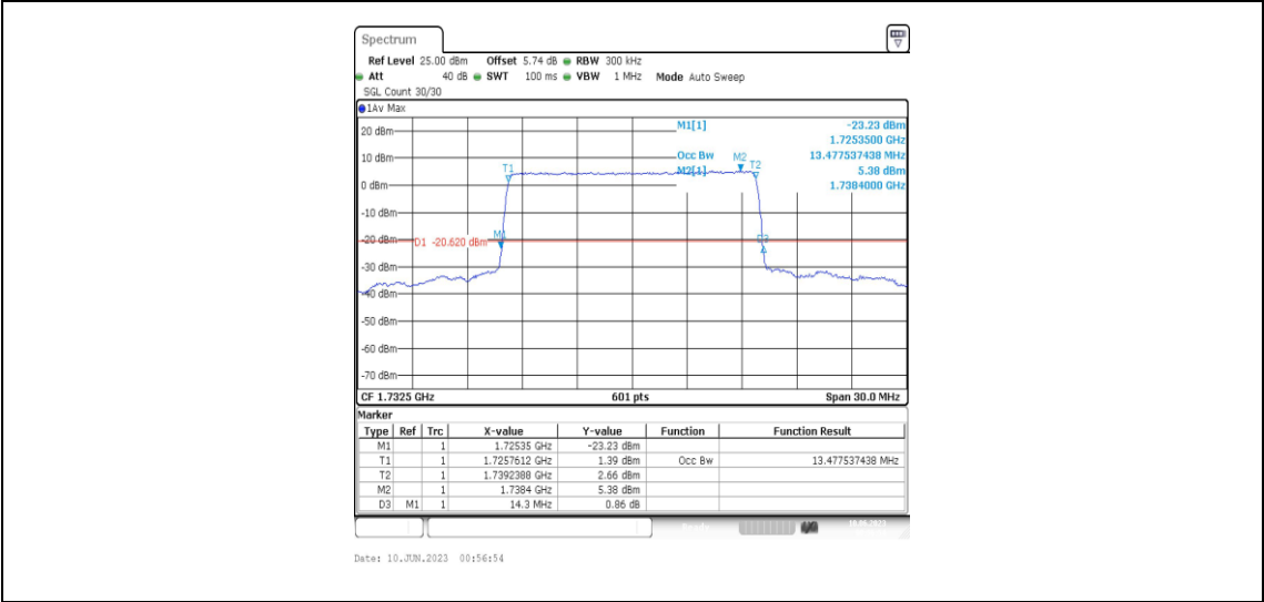
Band4-15MHz-QPSK-20175-75RB#0-13.478
