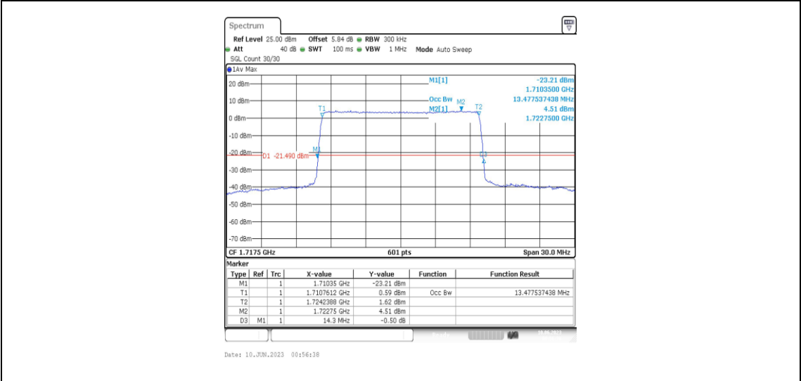
Band4-15MHz-16QAM-20025-75RB#0-13.478
