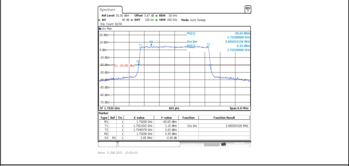
Band4-3MHz-16QAM-20385-15RB#0-2.686
