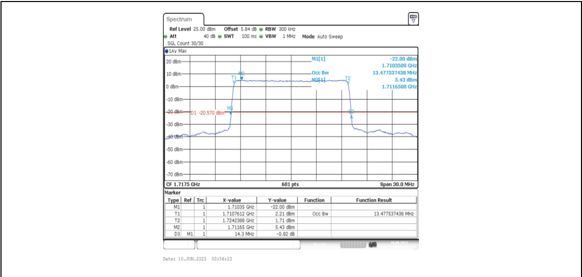
Band4-15MHz-QPSK-20025-75RB#0-13.478
