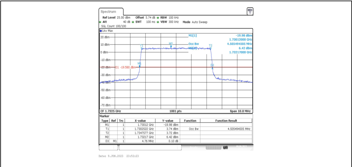
Band4-5MHz-16QAM-20175-25RB#0-4.505
