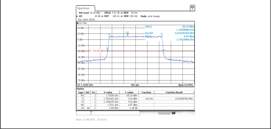
Band4-3MHz-QPSK-20385-15RB#0-2.676
