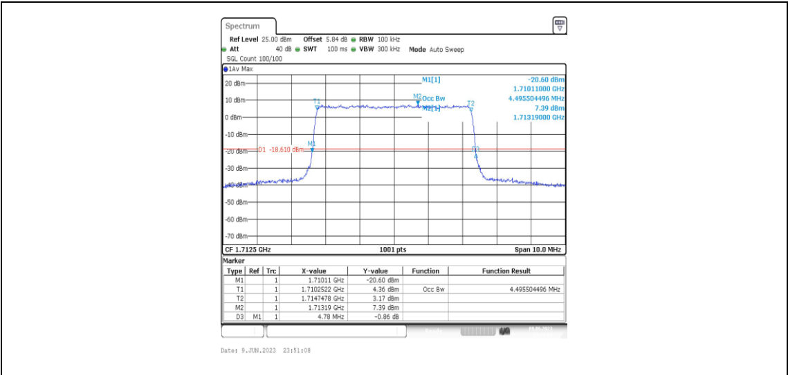
Band4-5MHz-QPSK-19975-25RB#0-4.496
