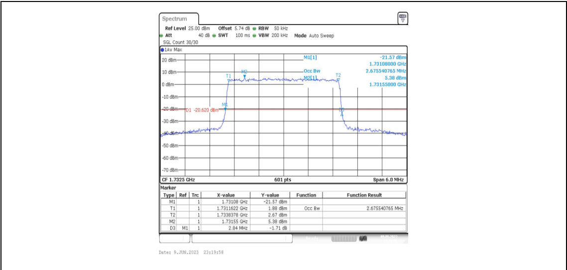
Band4-3MHz-16QAM-20175-15RB#0-2.676
