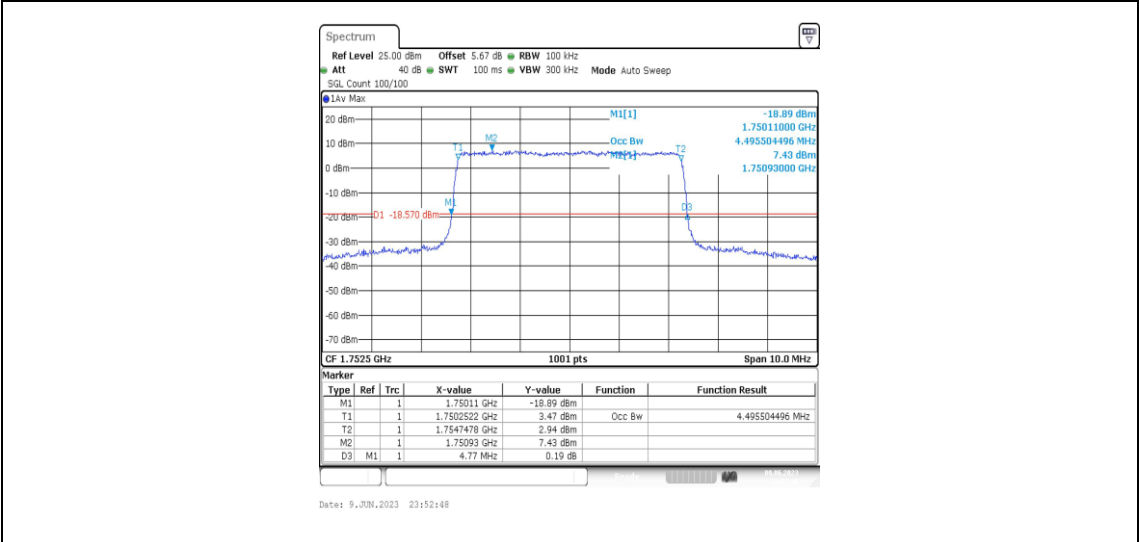
Band4-5MHz-QPSK-20375-25RB#0-4.496
