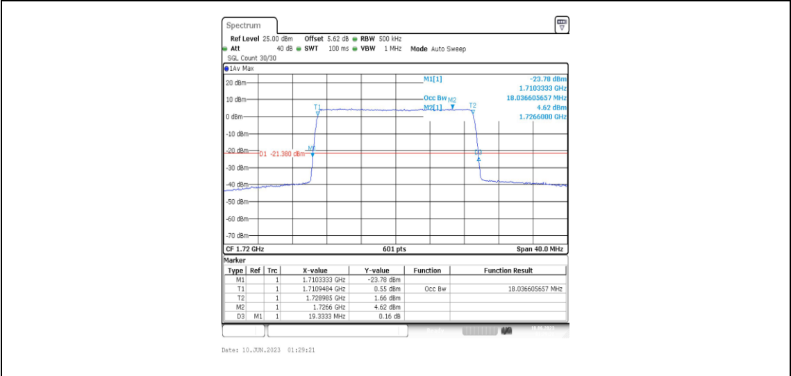
Band4-20MHz-16QAM-20050-100RB#0-18.037
