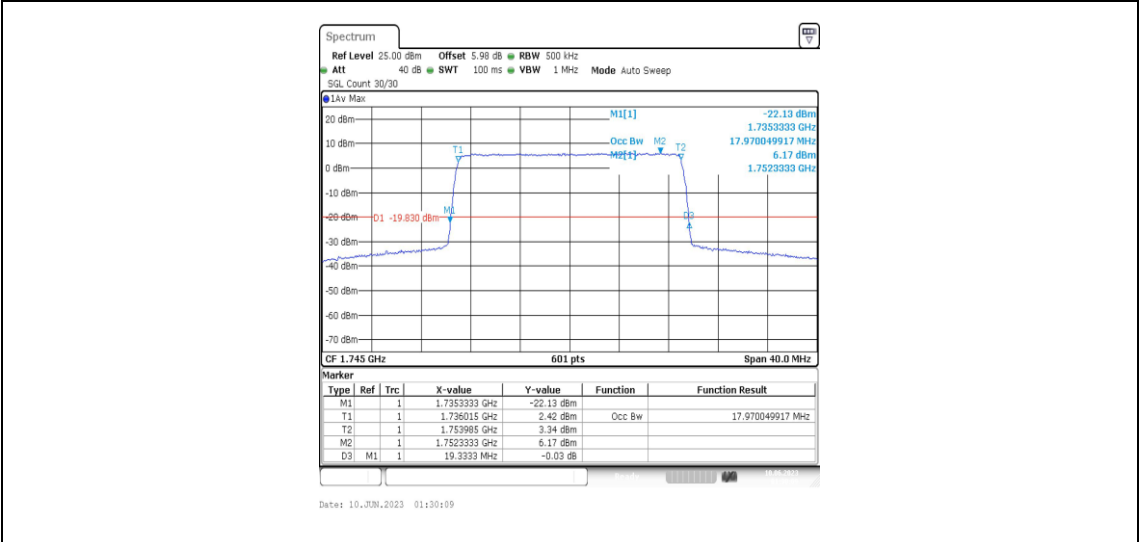
Band4-20MHz-QPSK-20300-100RB#0-17.97
