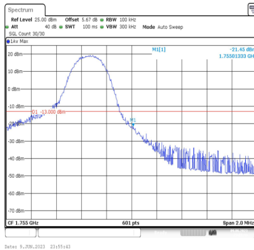
Band4-5MHz-16QAM-20375-1RB#24
