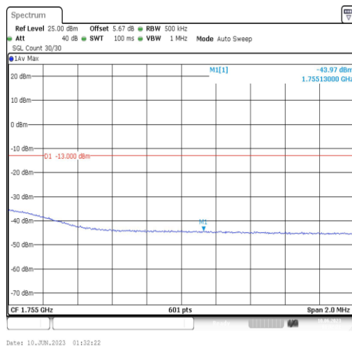
Band4-20MHz-QPSK-20300-1RB#0
