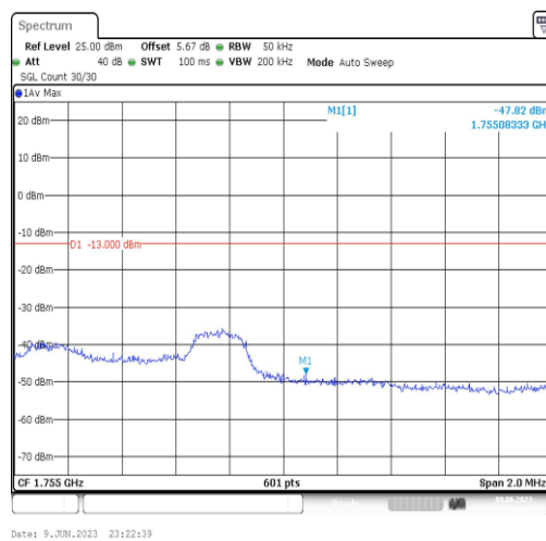
Band4-3MHz-16QAM-20385-1RB#0
