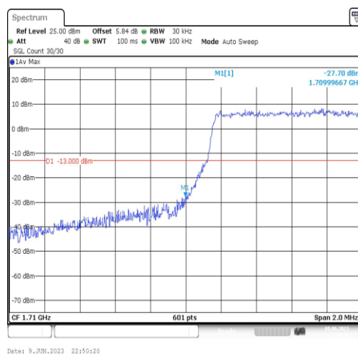
Band4-1.4MHz-16QAM-19957-6RB#0
