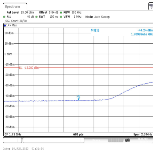
Band4-20MHz-16QAM-20050-1RB#99
