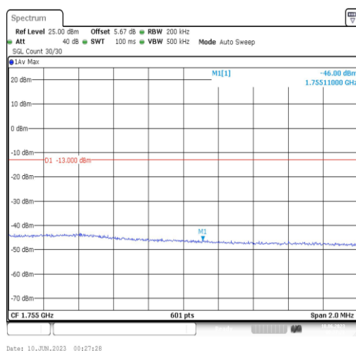
Band4-10MHz-16QAM-20350-1RB#0
