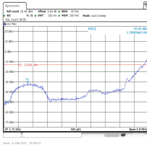
Band4-1.4MHz-16QAM-19957-1RB#5
