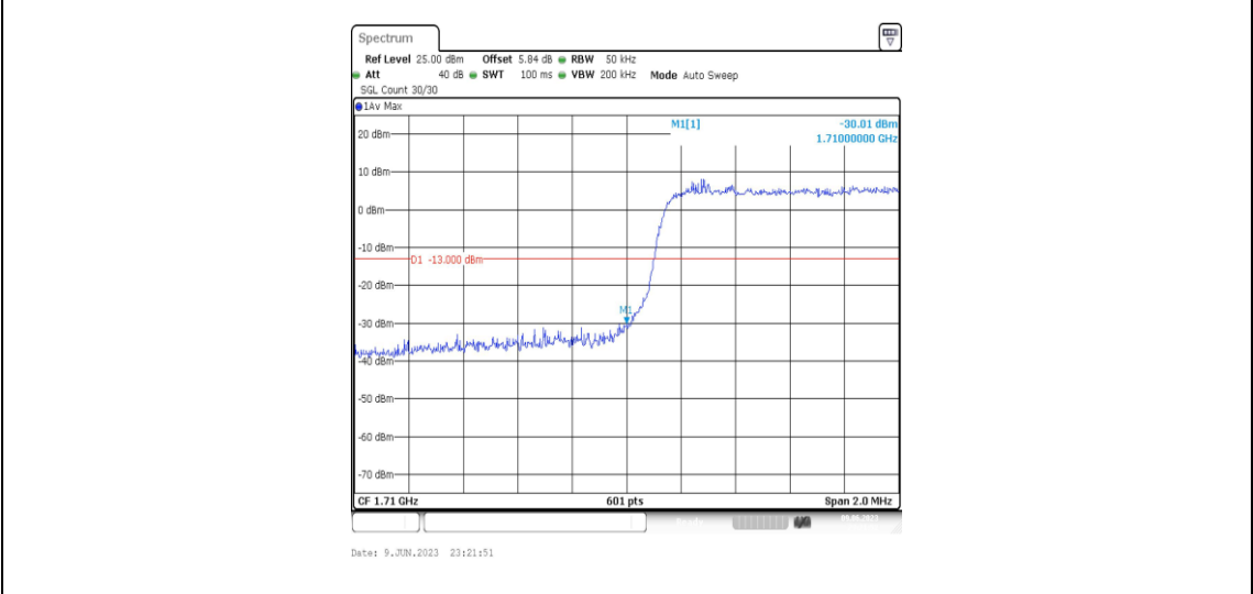
Band4-3MHz-QPSK-19965-15RB#0
