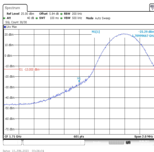
Band4-10MHz-16QAM-20000-1RB#0
