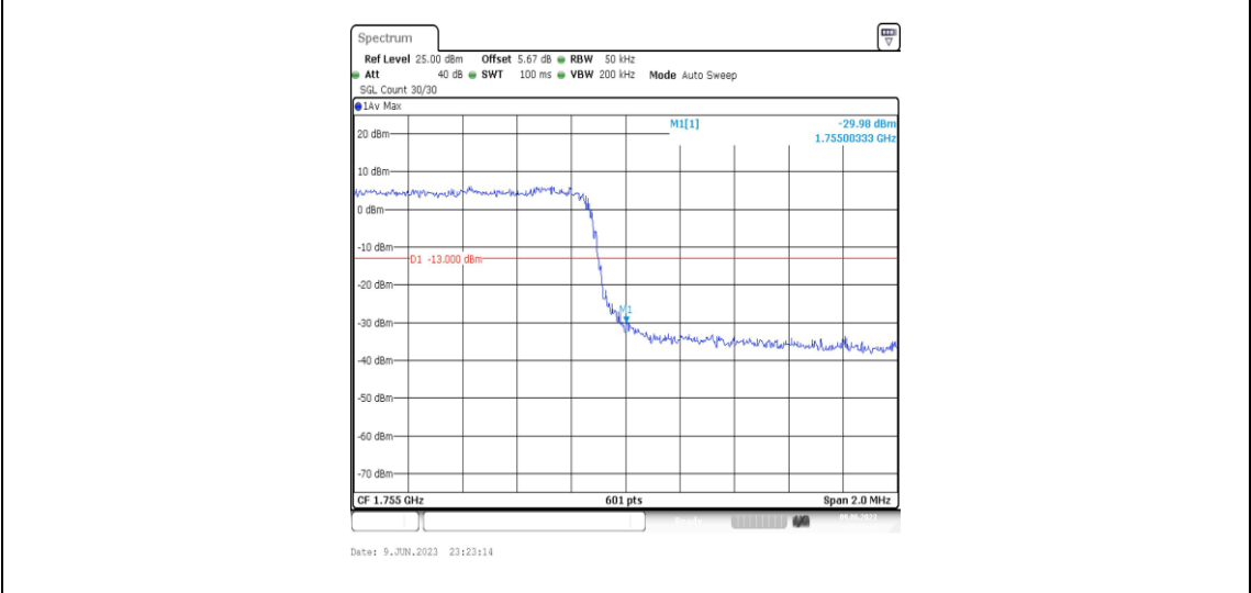
Band4-3MHz-QPSK-20385-15RB#0
