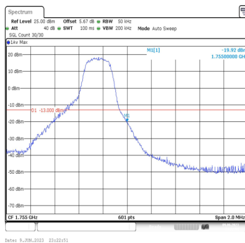
Band4-3MHz-QPSK-20385-1RB#14
