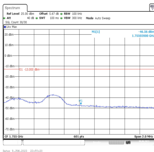
Band4-5MHz-16QAM-20375-1RB#0
