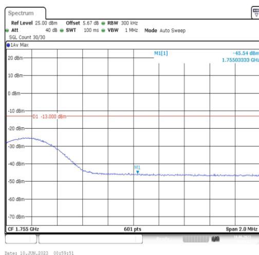
Band4-15MHz-16QAM-20325-1RB#0
