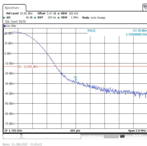
Band4-15MHz-QPSK-20325-1RB#74
