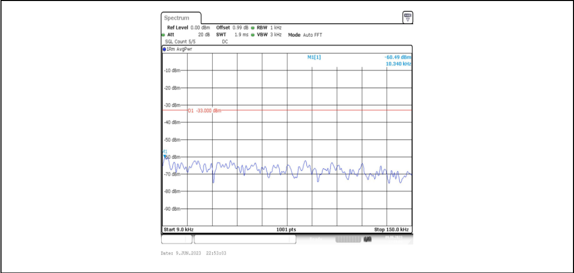
Band4-1.4MHz-16QAM-19957-1RB#0-Range1:0.009~0.15MHz
