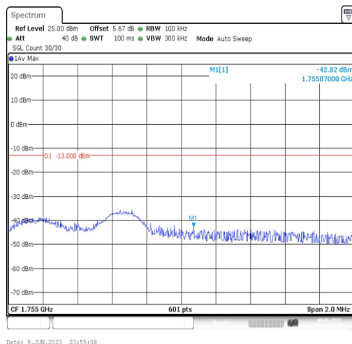
Band4-5MHz-QPSK-20375-1RB#0
