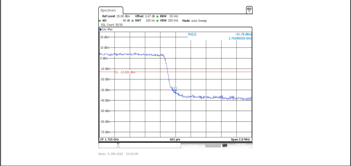
Band4-3MHz-16QAM-20385-15RB#0
