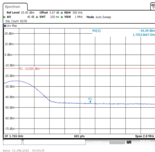
Band4-15MHz-QPSK-20325-1RB#0
