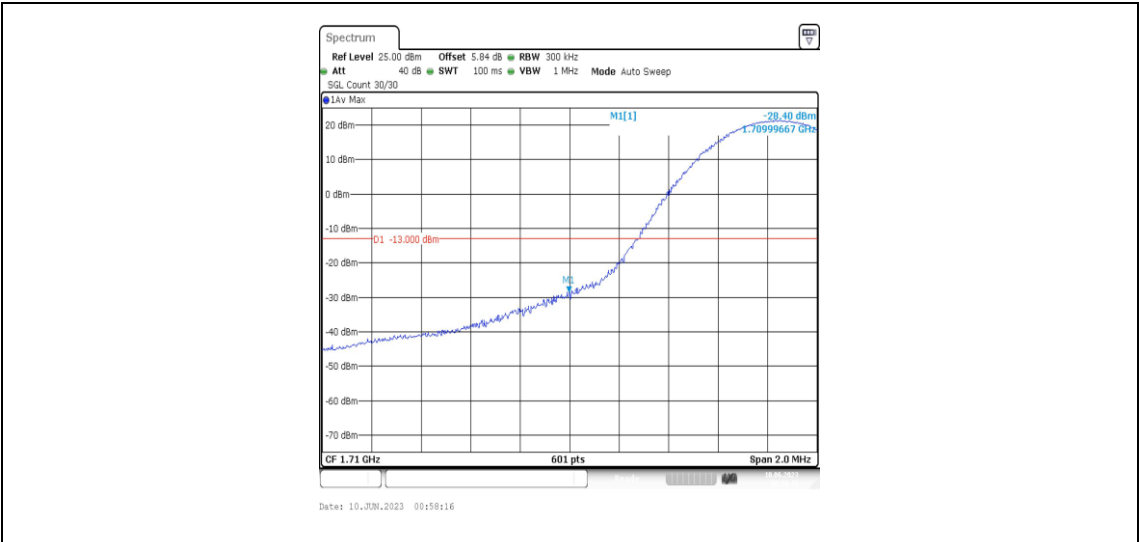
Band4-15MHz-QPSK-20025-1RB#0
