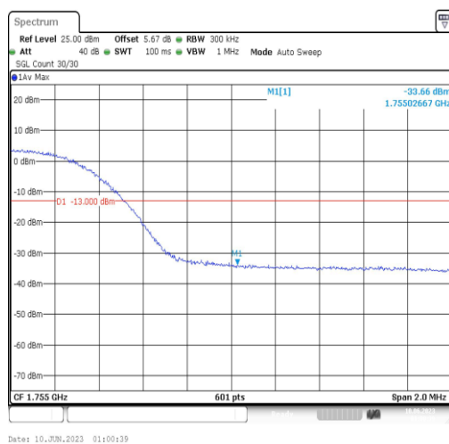
Band4-15MHz-16QAM-20325-75RB#0
