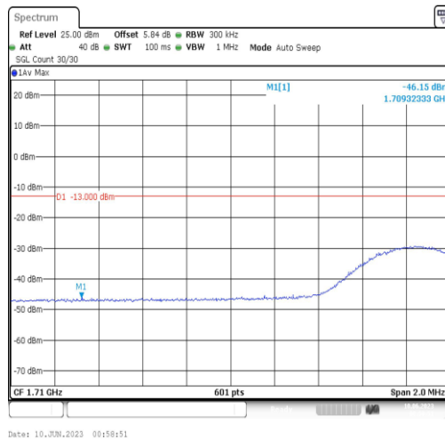
Band4-15MHz-16QAM-20025-1RB#74
