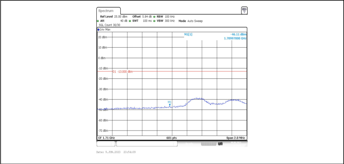
Band4-5MHz-QPSK-19975-1RB#24
