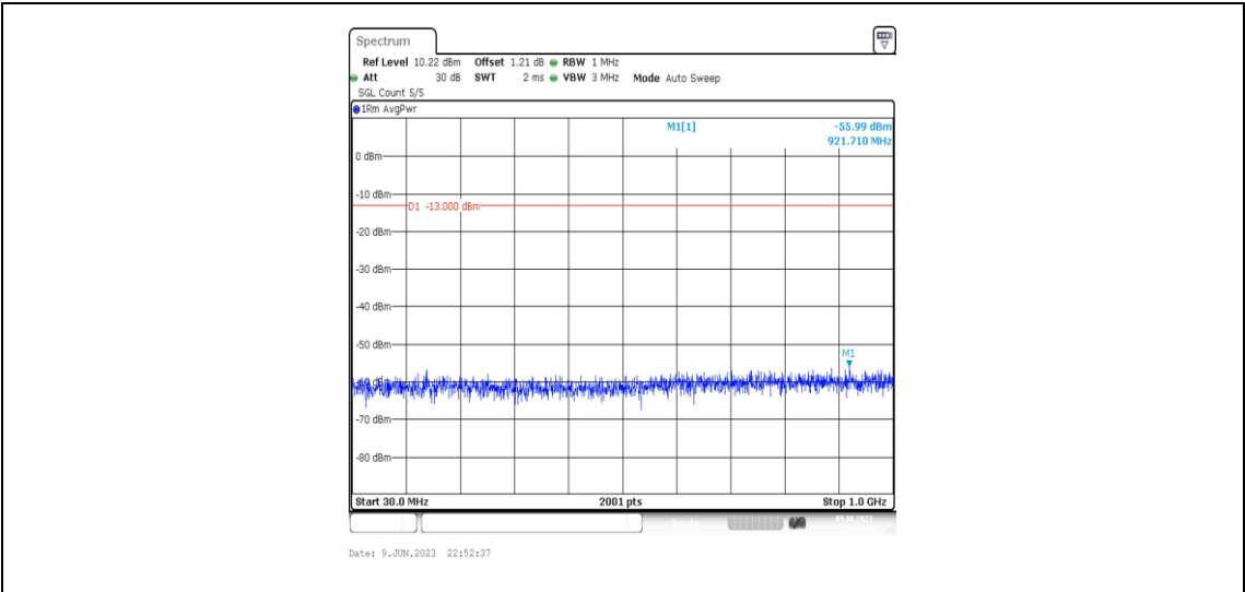
Band4-1.4MHz-QPSK-19957-1RB#0-Range3:30~1000MHz
