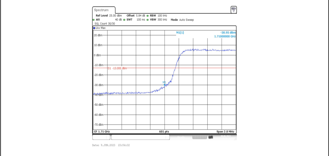
Band4-5MHz-QPSK-19975-25RB#0
