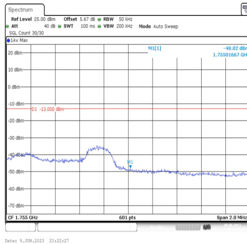
Band4-3MHz-QPSK-20385-1RB#0
