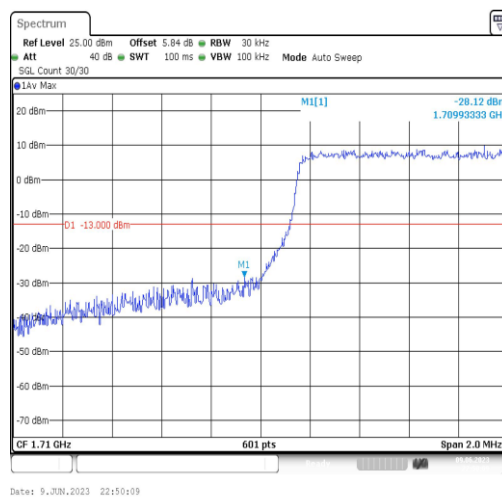
Band4-1.4MHz-QPSK-19957-6RB#0
