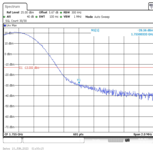
Band4-15MHz-16QAM-20325-1RB#74
