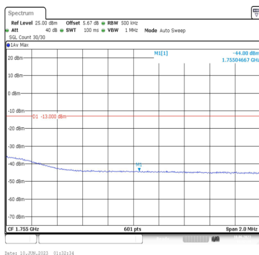
Band4-20MHz-16QAM-20300-1RB#0
