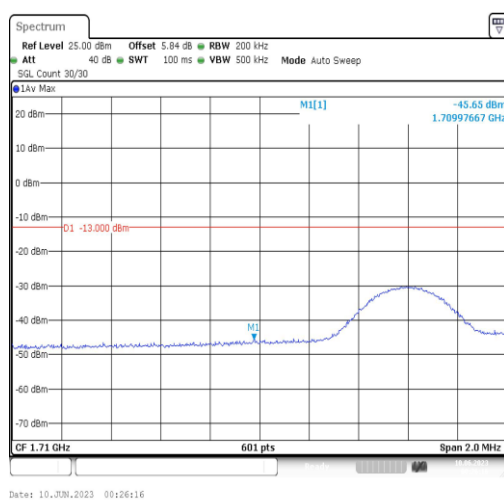
Band4-10MHz-QPSK-20000-1RB#49
