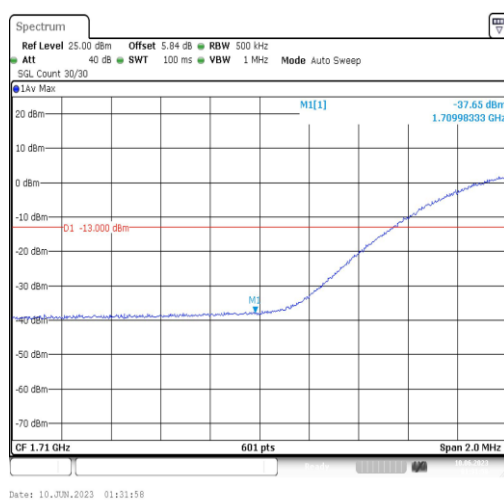
Band4-20MHz-16QAM-20050-100RB#0
