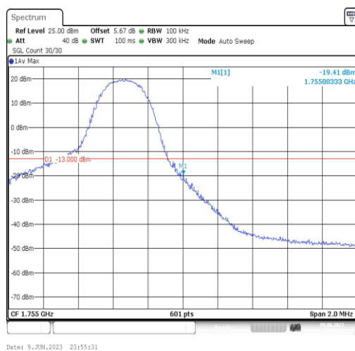
Band4-5MHz-QPSK-20375-1RB#24
