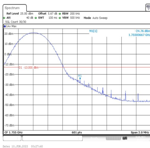
Band4-10MHz-QPSK-20350-1RB#49
