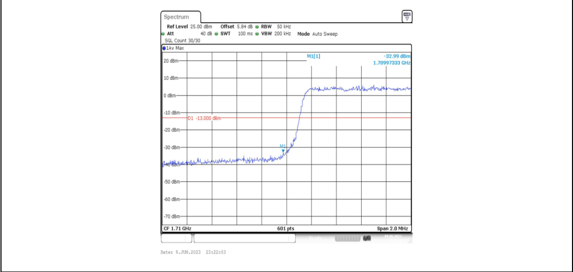
Band4-3MHz-16QAM-19965-15RB#0
