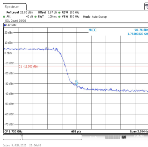
Band4-5MHz-16QAM-20375-25RB#0
