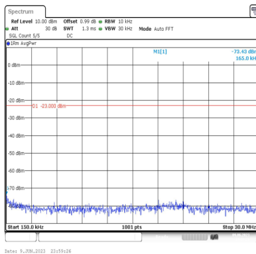
Band4-5MHz-16QAM-20175-1RB#0-Range2:0.15~30MHz
