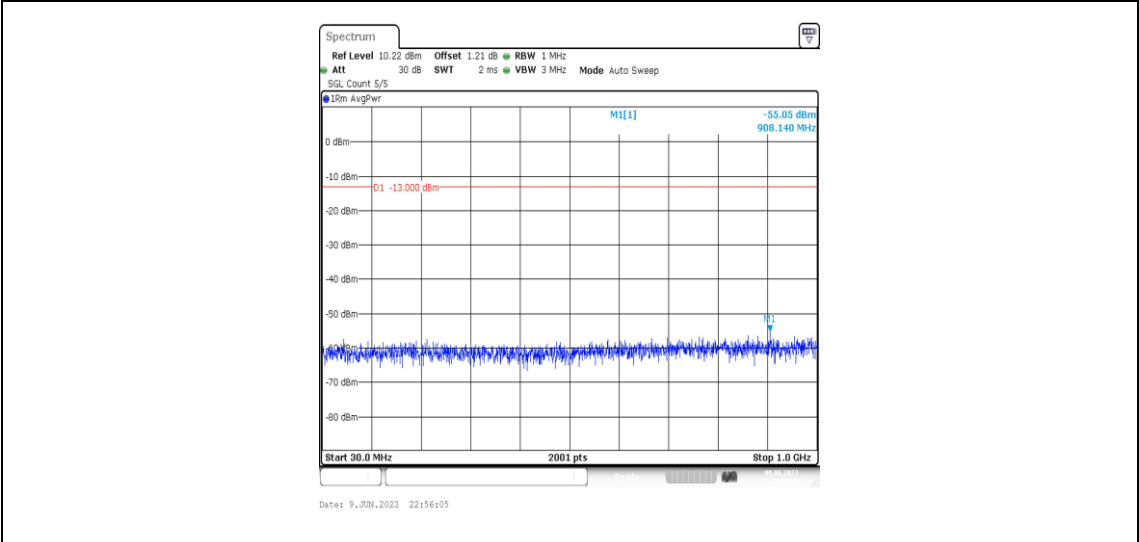
Band4-1.4MHz-QPSK-20393-1RB#0-Range3:30~1000MHz
