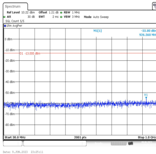
Band4-3MHz-16QAM-19965-1RB#0-Range3:30~1000MHz
