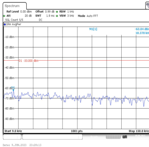
Band4-3MHz-16QAM-20385-1RB#0-Range1:0.009~0.15MHz
