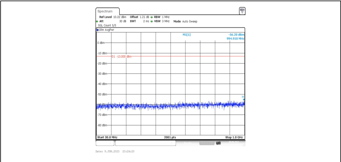
Band4-3MHz-QPSK-19965-1RB#0-Range3:30~1000MHz
