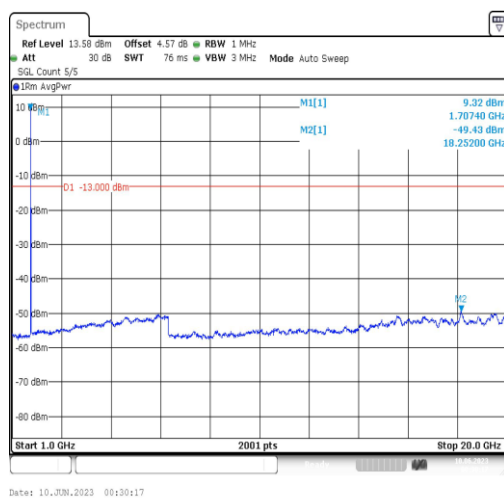
Band4-10MHz-16QAM-20000-1RB#0-Range4:1000~20000MHz
