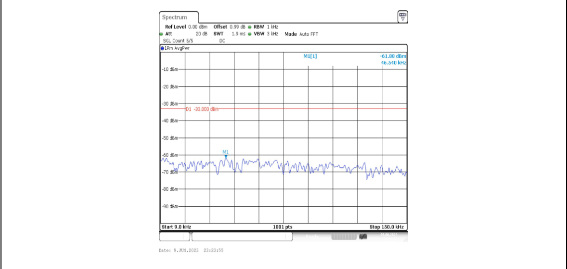
Band4-3MHz-QPSK-19965-1RB#0-Range1:0.009~0.15MHz
