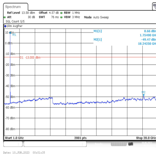
Band4-5MHz-16QAM-20375-1RB#0-Range4:1000~20000MHz
