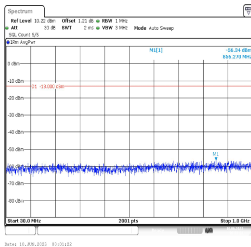
Band4-5MHz-16QAM-20375-1RB#0-Range3:30~1000MHz
