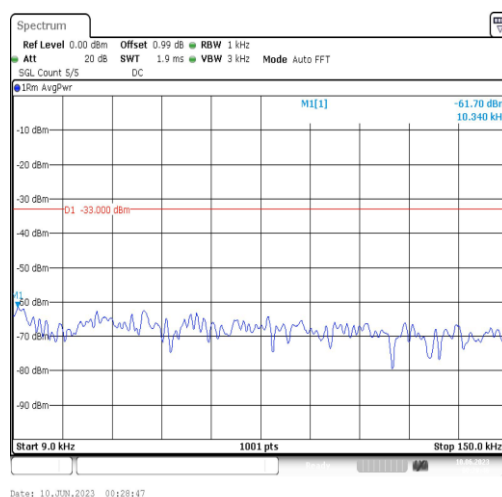
Band4-10MHz-QPSK-20000-1RB#0-Range1:0.009~0.15MHz
