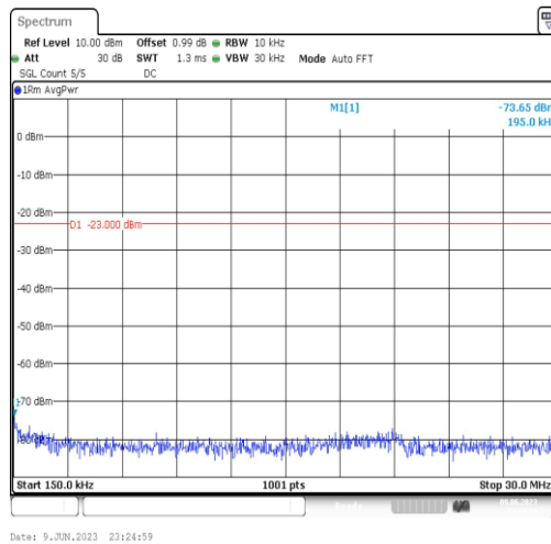
Band4-3MHz-16QAM-19965-1RB#0-Range2:0.15~30MHz
