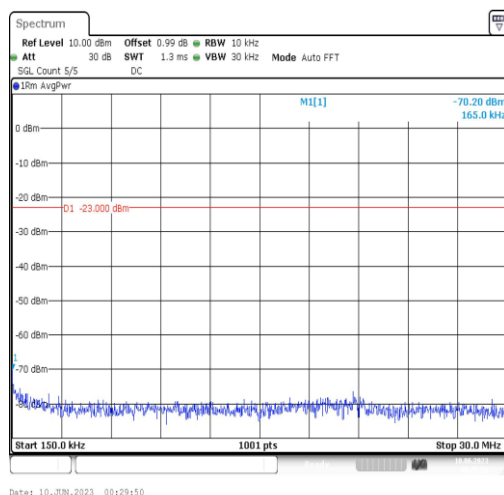
Band4-10MHz-16QAM-20000-1RB#0-Range2:0.15~30MHz
