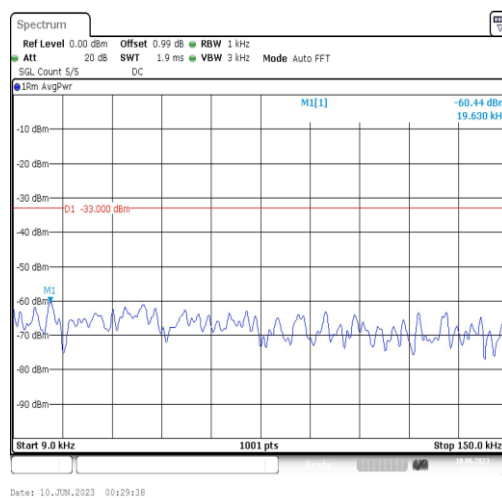
Band4-10MHz-16QAM-20000-1RB#0-Range1:0.009~0.15MHz
