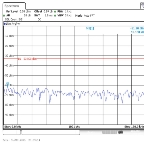
Band4-5MHz-16QAM-20175-1RB#0-Range1:0.009~0.15MHz
