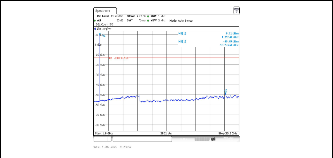
Band4-5MHz-16QAM-20175-1RB#0-Range4:1000~20000MHz
