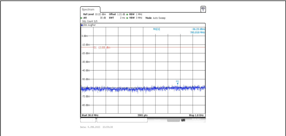
Band4-5MHz-16QAM-20175-1RB#0-Range3:30~1000MHz
