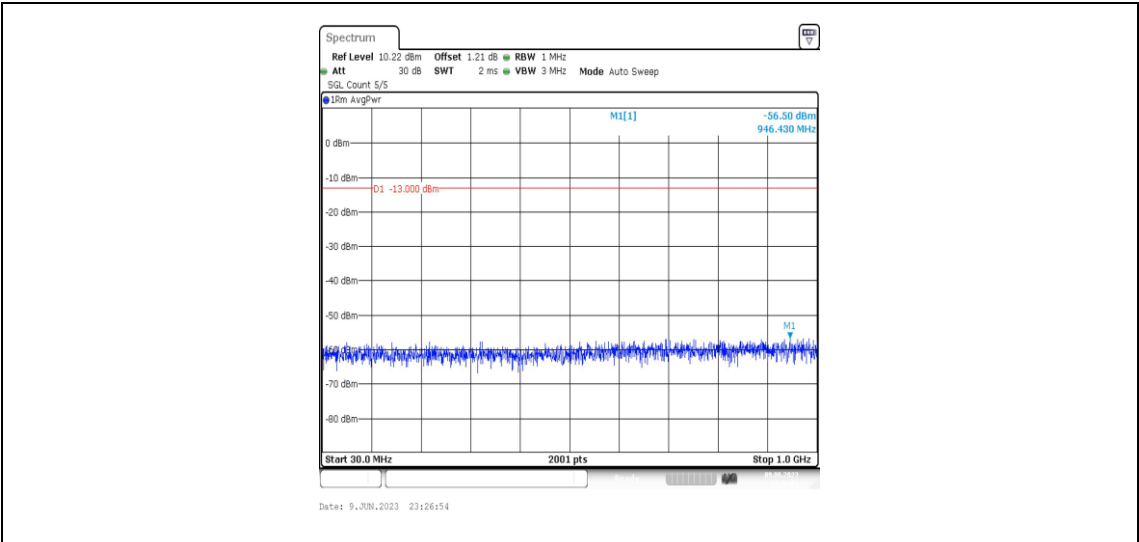
Band4-3MHz-16QAM-20175-1RB#0-Range3:30~1000MHz
