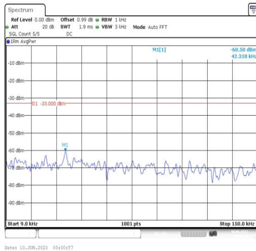
Band4-5MHz-16QAM-20375-1RB#0-Range1:0.009~0.15MHz
