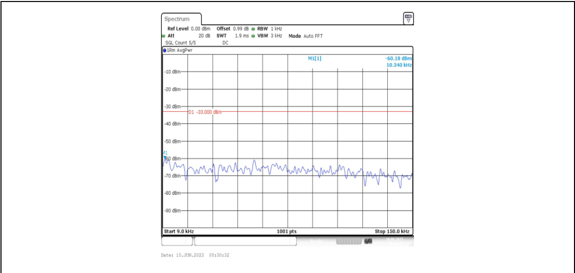
Band4-10MHz-QPSK-20175-1RB#0-Range1:0.009~0.15MHz
