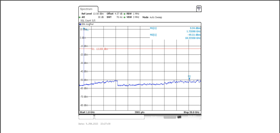
Band4-3MHz-16QAM-20175-1RB#0-Range4:1000~20000MHz
