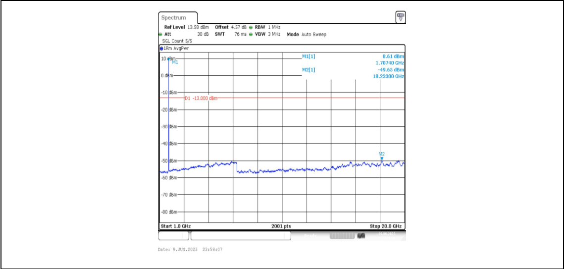
Band4-5MHz-16QAM-19975-1RB#0-Range4:1000~20000MHz
