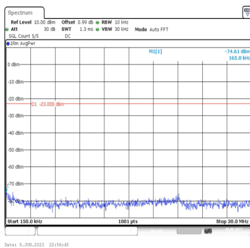
Band4-1.4MHz-16QAM-20393-1RB#0-Range2:0.15~30MHz
