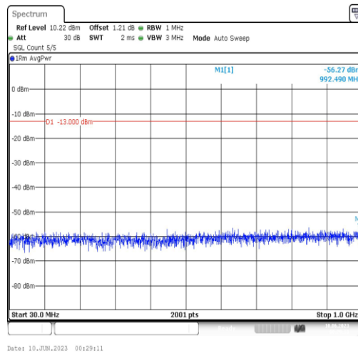
Band4-10MHz-QPSK-20000-1RB#0-Range3:30~1000MHz
