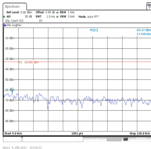
Band4-1.4MHz-16QAM-20393-1RB#0-Range1:0.009~0.15MHz
