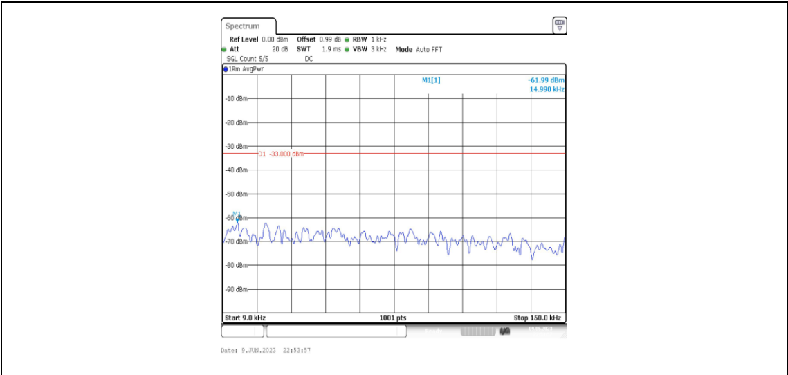
Band4-1.4MHz-QPSK-20175-1RB#0-Range1:0.009~0.15MHz
