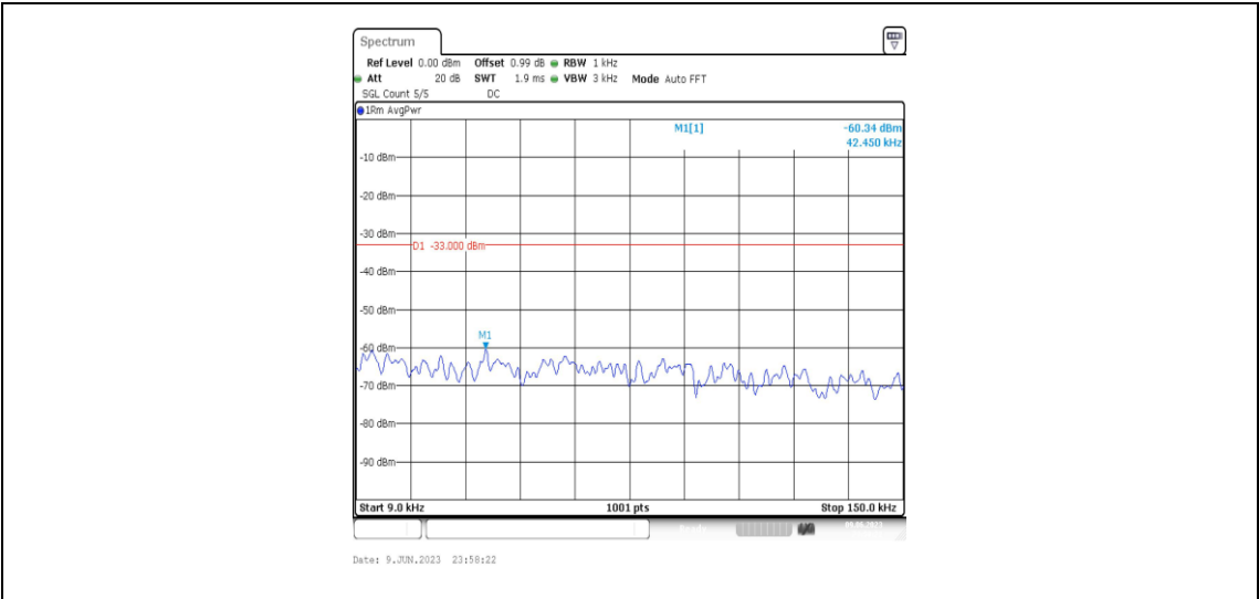
Band4-5MHz-QPSK-20175-1RB#0-Range1:0.009~0.15MHz
