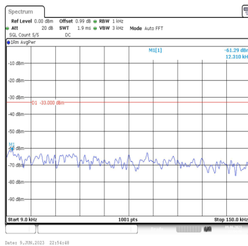
Band4-1.4MHz-16QAM-20175-1RB#0-Range1:0.009~0.15MHz
