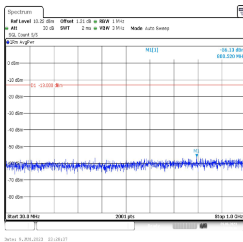
Band4-3MHz-16QAM-20385-1RB#0-Range3:30~1000MHz
