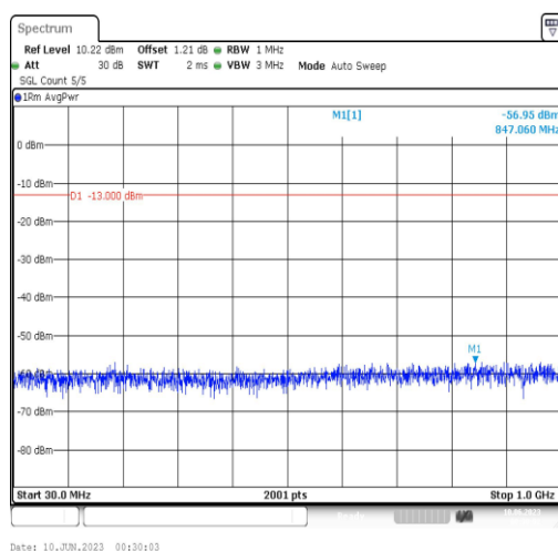
Band4-10MHz-16QAM-20000-1RB#0-Range3:30~1000MHz
