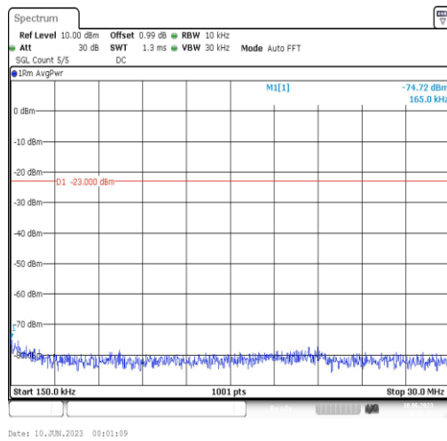
Band4-5MHz-16QAM-20375-1RB#0-Range2:0.15~30MHz
