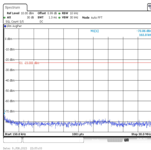
Band4-1.4MHz-16QAM-20175-1RB#0-Range2:0.15~30MHz
