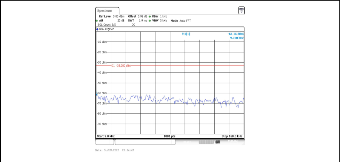
Band4-3MHz-16QAM-19965-1RB#0-Range1:0.009~0.15MHz
