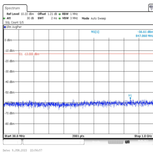
Band4-1.4MHz-16QAM-20393-1RB#0-Range3:30~1000MHz
