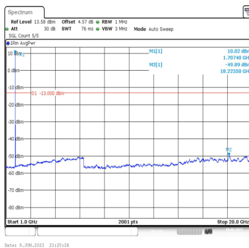
Band4-3MHz-16QAM-19965-1RB#0-Range4:1000~20000MHz
