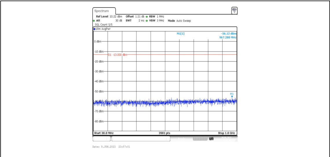
Band4-5MHz-QPSK-19975-1RB#0-Range3:30~1000MHz
