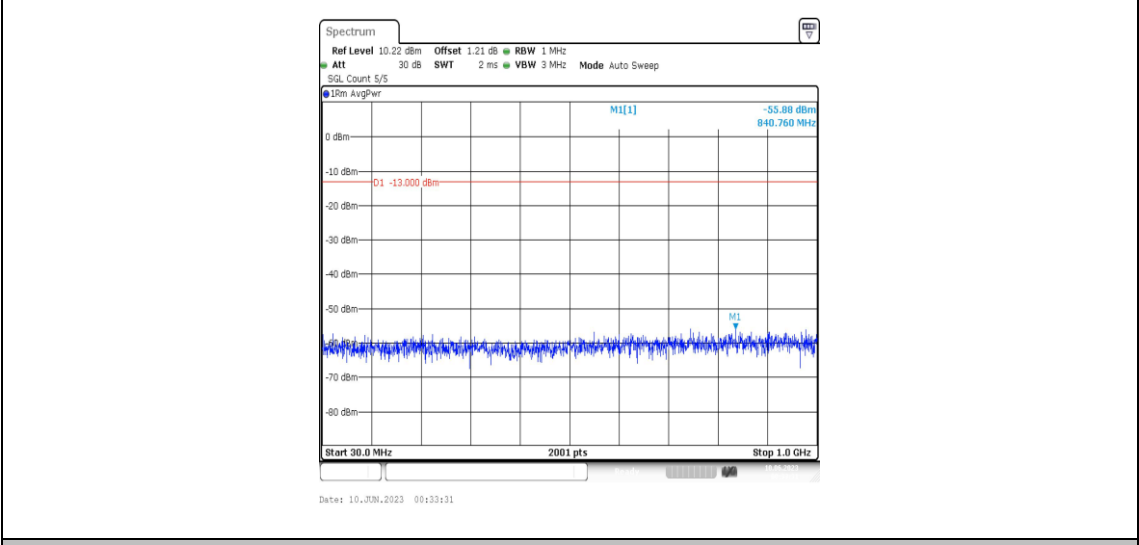
Band4-10MHz-16QAM-20350-1RB#0-Range3:30~1000MHz
