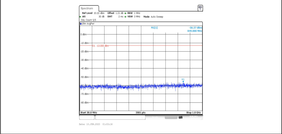
Band4-15MHz-QPSK-20175-1RB#0-Range3:30~1000MHz
