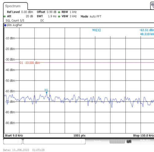
Band4-15MHz-16QAM-20325-1RB#0-Range1:0.009~0.15MHz
