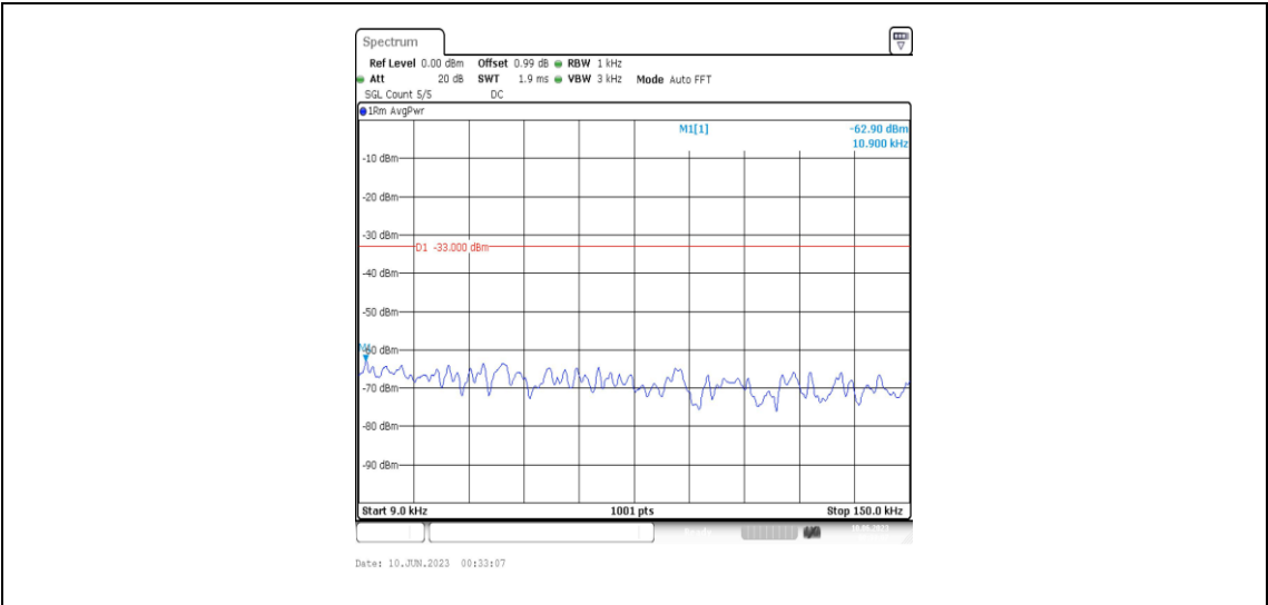
Band4-10MHz-16QAM-20350-1RB#0-Range1:0.009~0.15MHz
