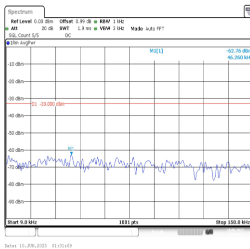
Band4-15MHz-QPSK-20025-1RB#0-Range1:0.009~0.15MHz
