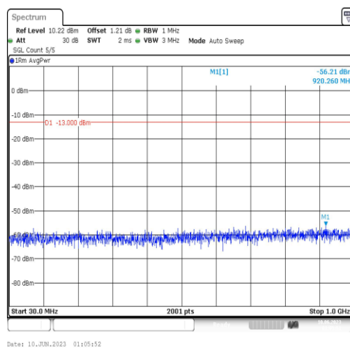
Band4-15MHz-16QAM-20325-1RB#0-Range3:30~1000MHz
