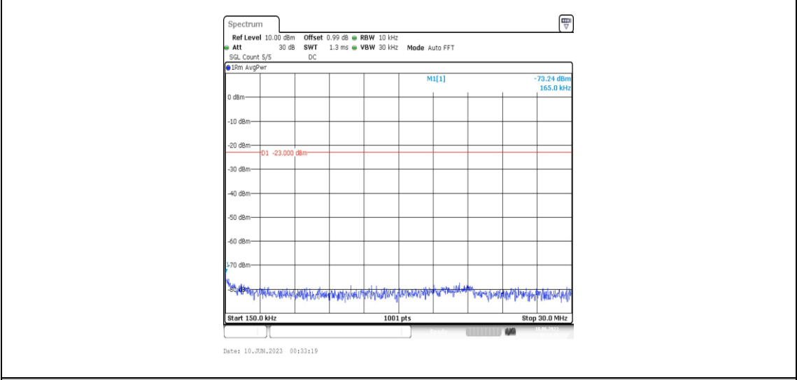
Band4-10MHz-16QAM-20350-1RB#0-Range2:0.15~30MHz
