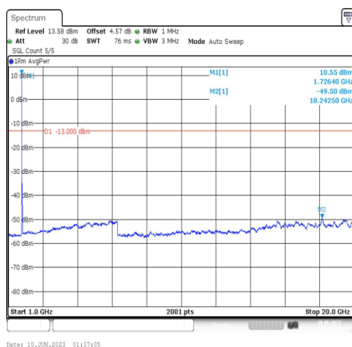
Band4-20MHz-16QAM-20175-1RB#0-Range4:1000~20000MHz
