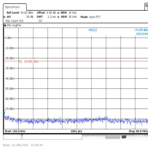
Band4-15MHz-16QAM-20325-1RB#0-Range2:0.15~30MHz
