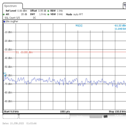
Band4-15MHz-16QAM-20175-1RB#0-Range1:0.009~0.15MHz
