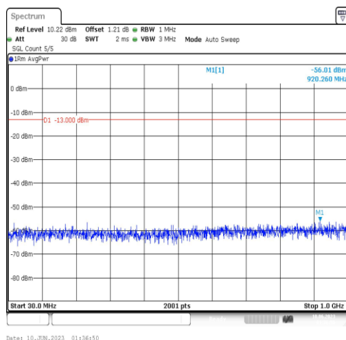
Band4-20MHz-16QAM-20175-1RB#0-Range3:30~1000MHz
