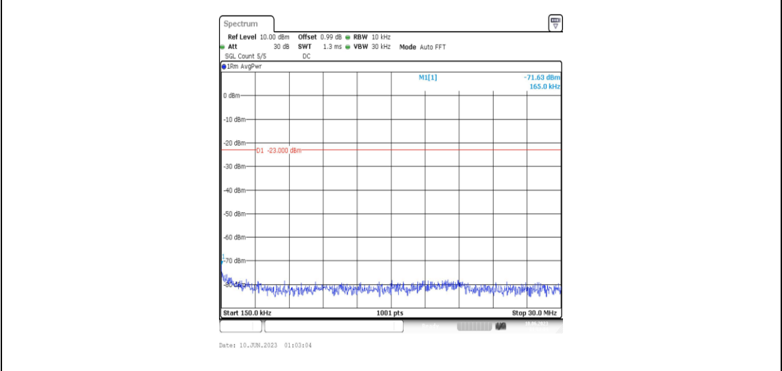
Band4-15MHz-QPSK-20175-1RB#0-Range2:0.15~30MHz
