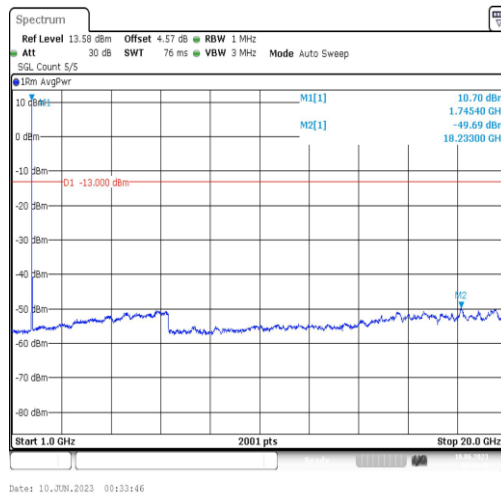
Band4-10MHz-16QAM-20350-1RB#0-Range4:1000~20000MHz
