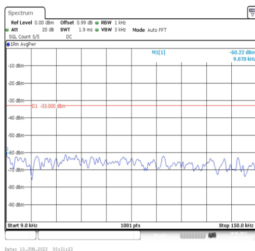
Band4-10MHz-16QAM-20175-1RB#0-Range1:0.009~0.15MHz
