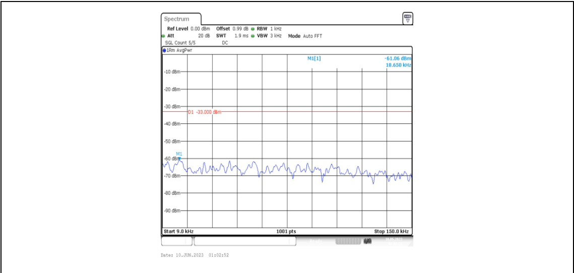
Band4-15MHz-QPSK-20175-1RB#0-Range1:0.009~0.15MHz
