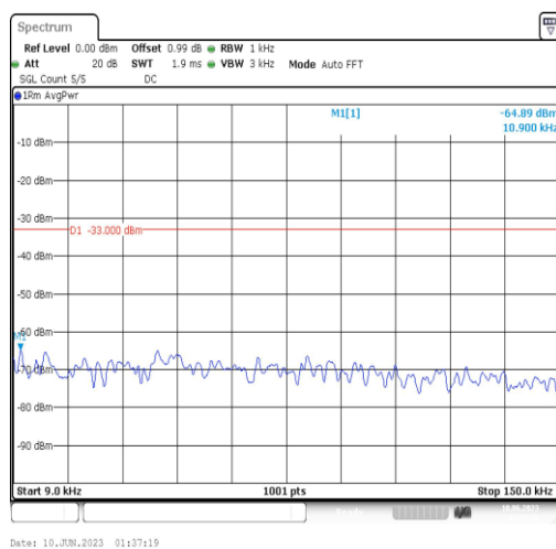
Band4-20MHz-QPSK-20300-1RB#0-Range1:0.009~0.15MHz
