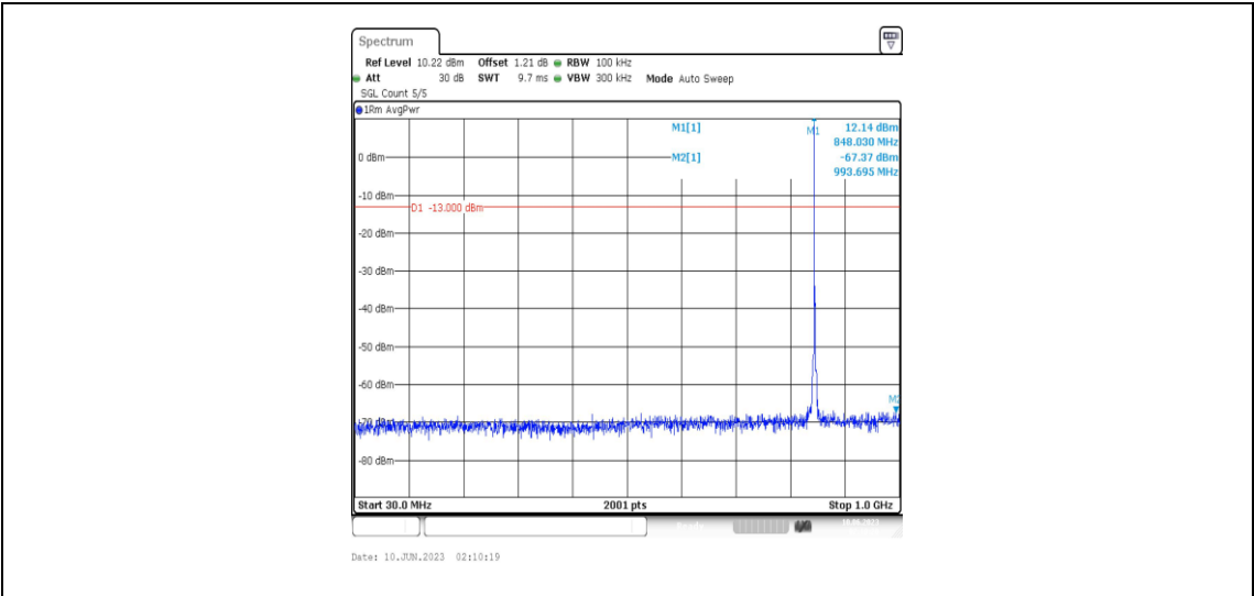
Band5-1.4MHz-QPSK-20643-1RB#0-Range3:30~1000MHz
