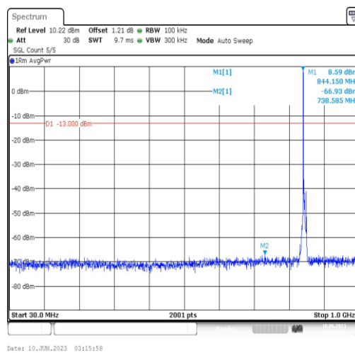
Band5-5MHz-16QAM-20625-1RB#0-Range3:30~1000MHz
