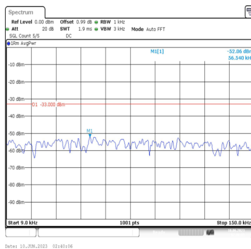
Band5-3MHz-QPSK-20525-1RB#0-Range1:0.009~0.15MHz
