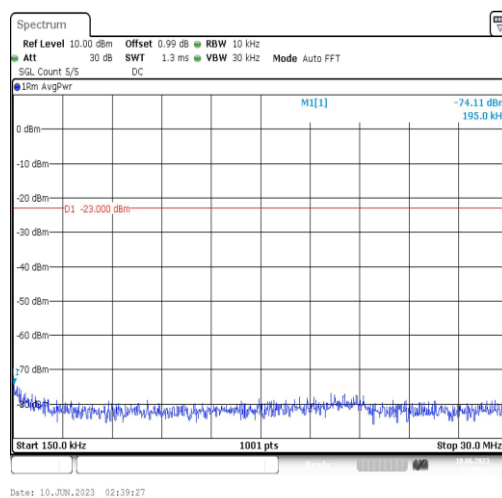
Band5-3MHz-16QAM-20415-1RB#0-Range2:0.15~30MHz
