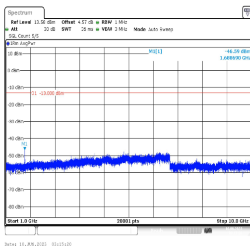
Band5-5MHz-QPSK-20625-1RB#0-Range4:1000~10000MHz
