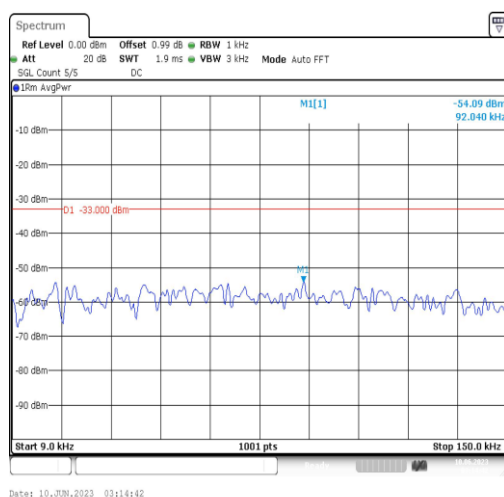
Band5-5MHz-QPSK-20625-1RB#0-Range1:0.009~0.15MHz
