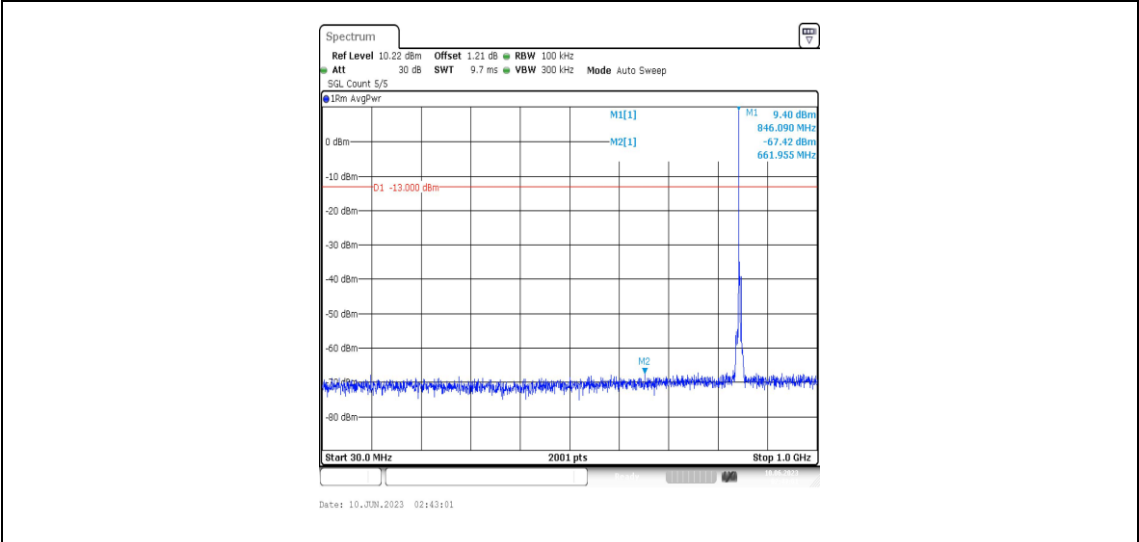
Band5-3MHz-16QAM-20635-1RB#0-Range3:30~1000MHz
