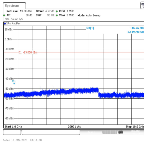
Band5-5MHz-QPSK-20425-1RB#0-Range4:1000~10000MHz
