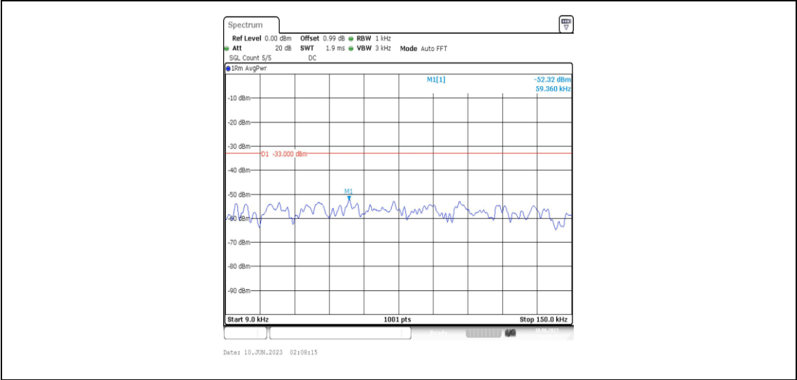
Band5-1.4MHz-QPSK-20525-1RB#0-Range1:0.009~0.15MHz
