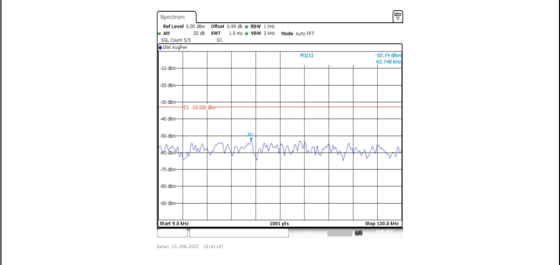
Band5-3MHz-QPSK-20635-1RB#0-Range1:0.009~0.15MHz
