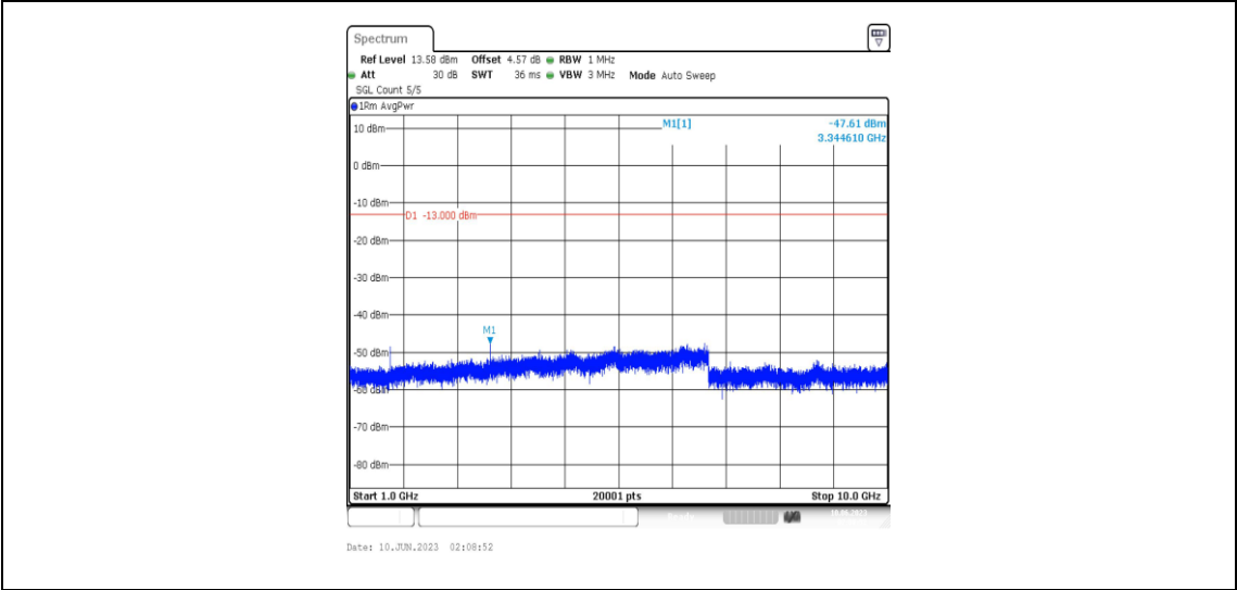
Band5-1.4MHz-QPSK-20525-1RB#0-Range4:1000~10000MHz
