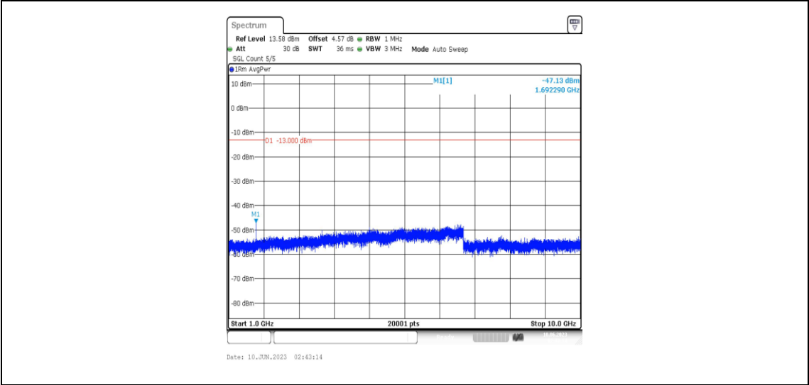
Band5-3MHz-16QAM-20635-1RB#0-Range4:1000~10000MHz
