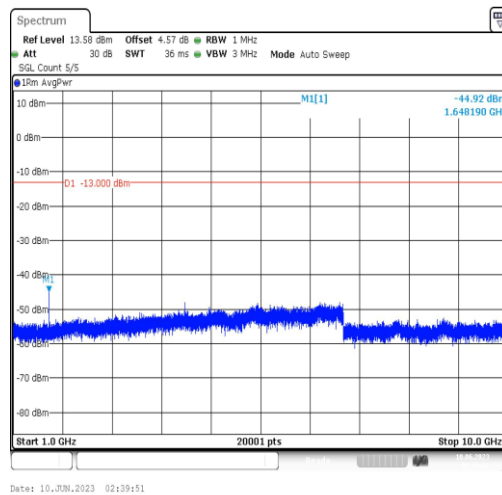
Band5-3MHz-16QAM-20415-1RB#0-Range4:1000~10000MHz
