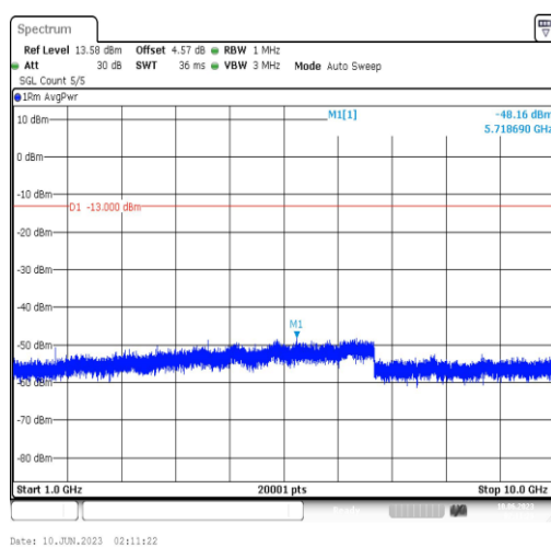
Band5-1.4MHz-16QAM-20643-1RB#0-Range4:1000~10000MHz
