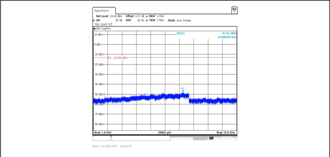
Band5-3MHz-QPSK-20635-1RB#0-Range4:1000~10000MHz
