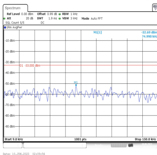
Band5-1.4MHz-QPSK-20643-1RB#0-Range1:0.009~0.15MHz
