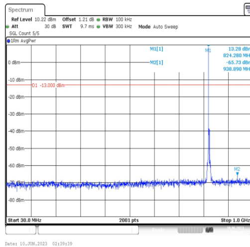
Band5-3MHz-16QAM-20415-1RB#0-Range3:30~1000MHz
