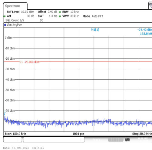
Band5-5MHz-16QAM-20625-1RB#0-Range2:0.15~30MHz
