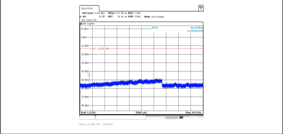
Band5-3MHz-QPSK-20525-1RB#0-Range4:1000~10000MHz
