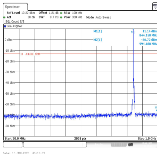
Band5-5MHz-QPSK-20625-1RB#0-Range3:30~1000MHz
