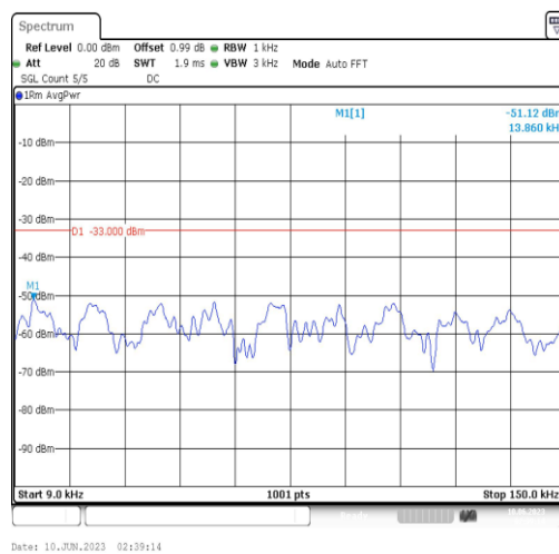
Band5-3MHz-16QAM-20415-1RB#0-Range1:0.009~0.15MHz
