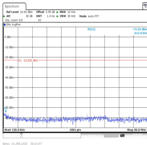
Band5-1.4MHz-16QAM-20643-1RB#0-Range2:0.15~30MHz
