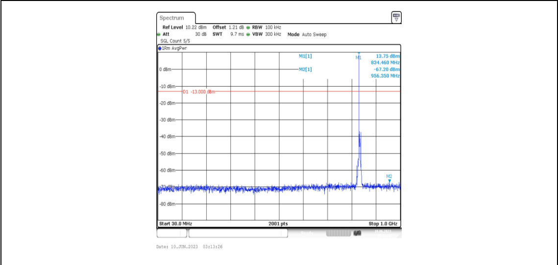
Band5-5MHz-QPSK-20525-1RB#0-Range3:30~1000MHz
