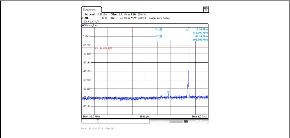
Band5-3MHz-QPSK-20635-1RB#0-Range3:30~1000MHz
