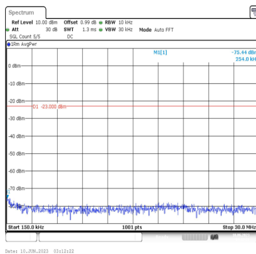
Band5-5MHz-16QAM-20425-1RB#0-Range2:0.15~30MHz
