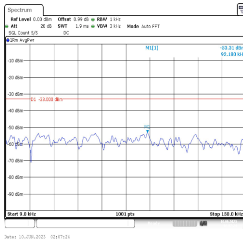
Band5-1.4MHz-16QAM-20407-1RB#0-Range1:0.009~0.15MHz
