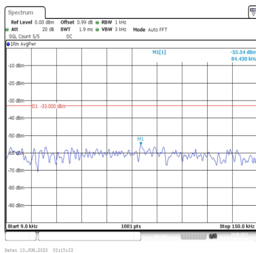
Band5-5MHz-16QAM-20625-1RB#0-Range1:0.009~0.15MHz
