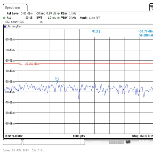
Band5-5MHz-QPSK-20525-1RB#0-Range1:0.009~0.15MHz
