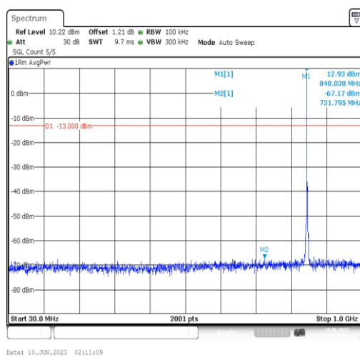
Band5-1.4MHz-16QAM-20643-1RB#0-Range3:30~1000MHz
