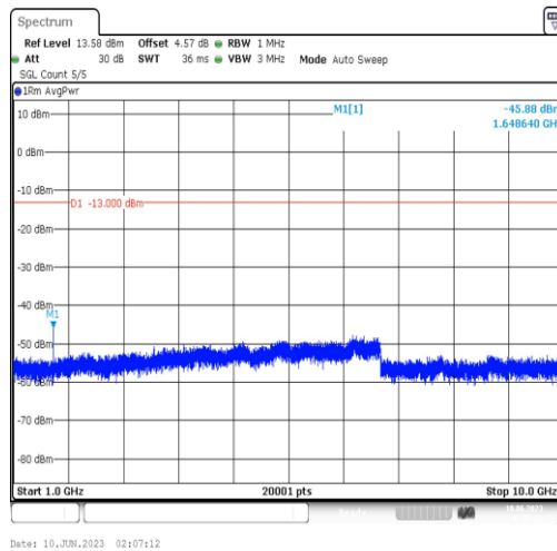
Band5-1.4MHz-QPSK-20407-1RB#0-Range4:1000~10000MHz
