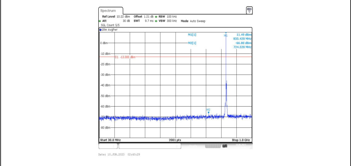
Band5-3MHz-QPSK-20525-1RB#0-Range3:30~1000MHz
