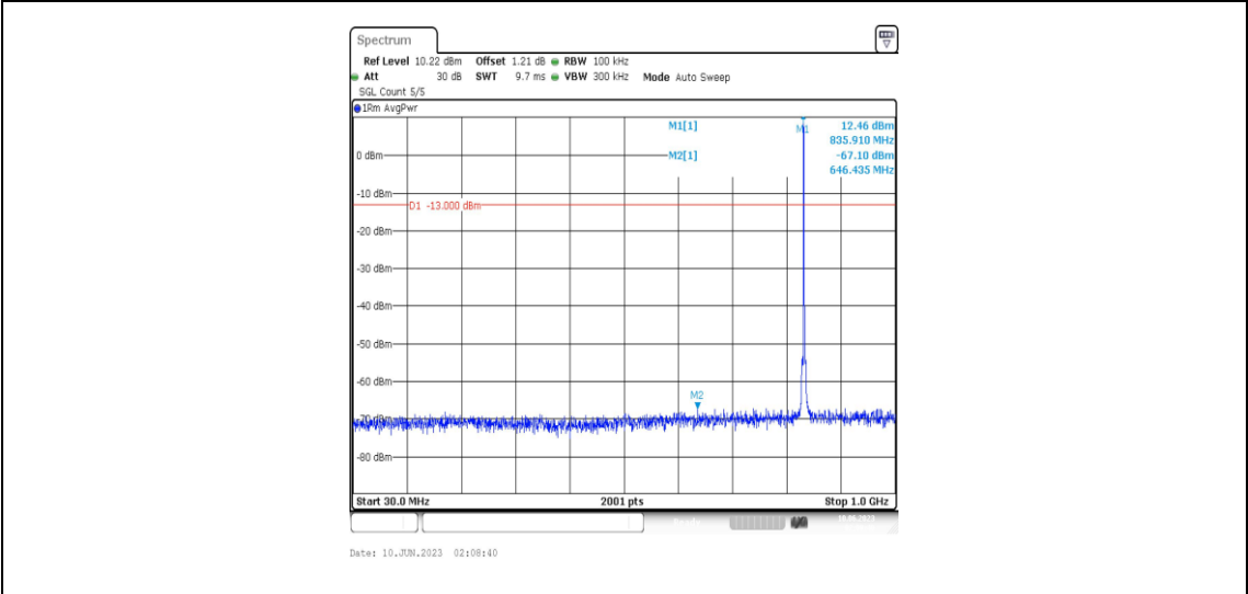
Band5-1.4MHz-QPSK-20525-1RB#0-Range3:30~1000MHz
