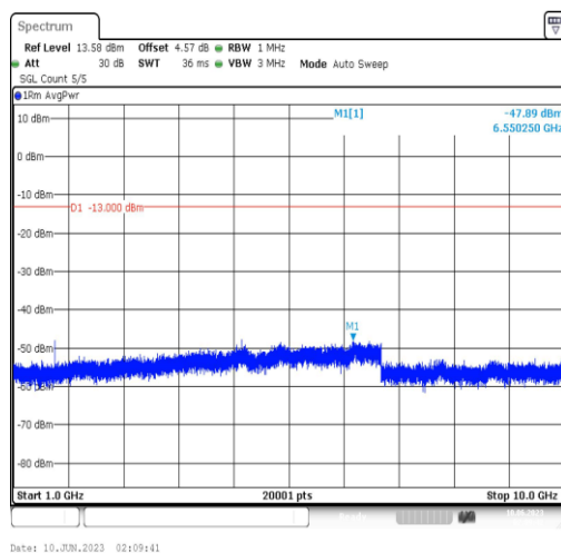
Band5-1.4MHz-16QAM-20525-1RB#0-Range4:1000~10000MHz
