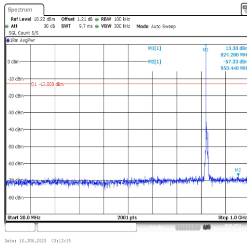
Band5-5MHz-16QAM-20425-1RB#0-Range3:30~1000MHz
