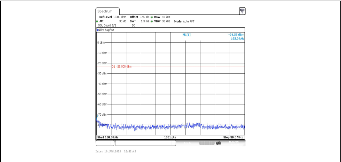
Band5-3MHz-16QAM-20635-1RB#0-Range2:0.15~30MHz
