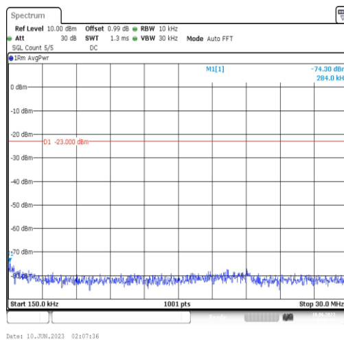
Band5-1.4MHz-16QAM-20407-1RB#0-Range2:0.15~30MHz
