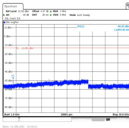
Band5-5MHz-16QAM-20625-1RB#0-Range4:1000~10000MHz
