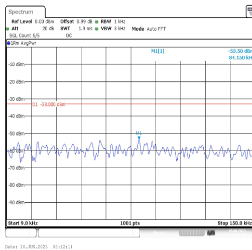
Band5-5MHz-16QAM-20425-1RB#0-Range1:0.009~0.15MHz
