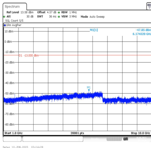
Band5-5MHz-16QAM-20525-1RB#0-Range4:1000~10000MHz
