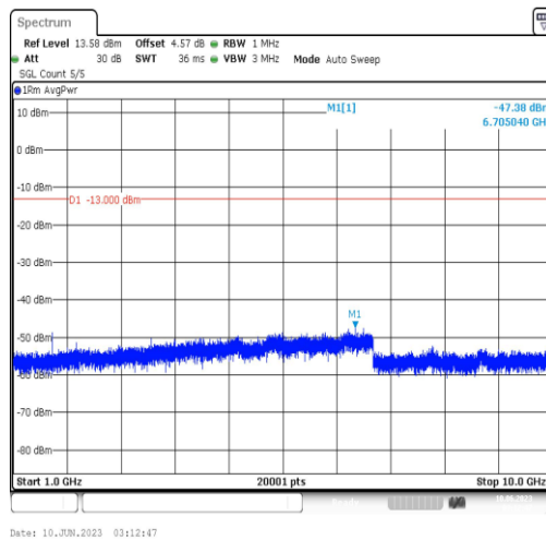
Band5-5MHz-16QAM-20425-1RB#0-Range4:1000~10000MHz
