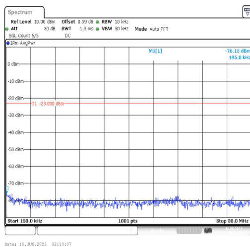
Band5-1.4MHz-QPSK-20643-1RB#0-Range2:0.15~30MHz
