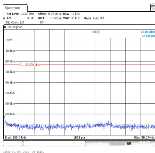
Band5-10MHz-16QAM-20525-1RB#0-Range2:0.15~30MHz
