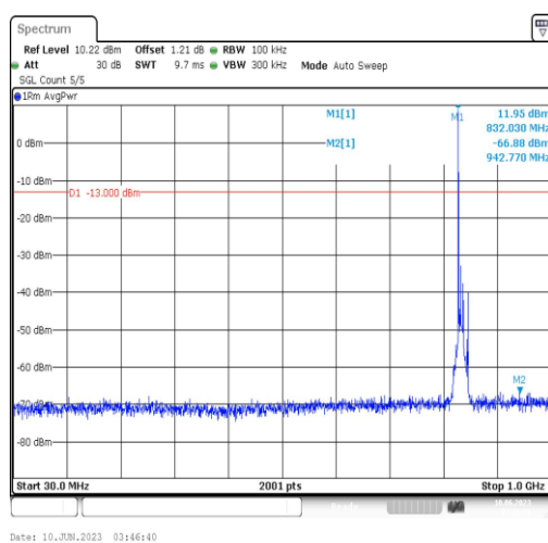
Band5-10MHz-16QAM-20525-1RB#0-Range3:30~1000MHz
