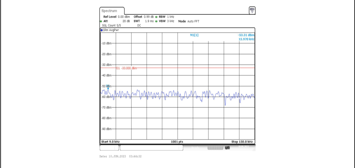
Band5-10MHz-16QAM-20450-1RB#0-Range1:0.009~0.15MHz
