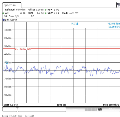
Band5-10MHz-16QAM-20525-1RB#0-Range1:0.009~0.15MHz
