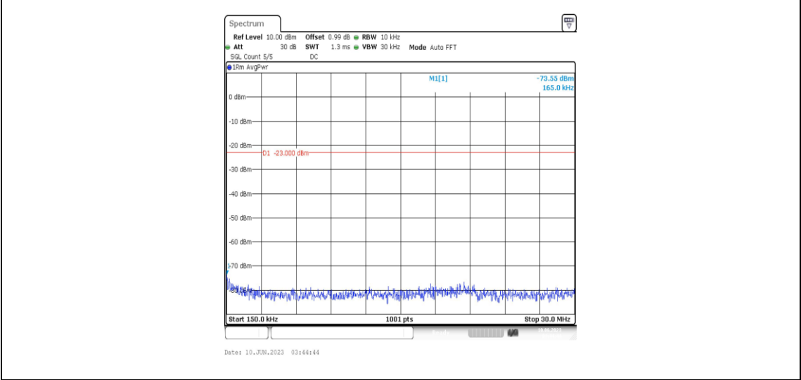
Band5-10MHz-16QAM-20450-1RB#0-Range2:0.15~30MHz
