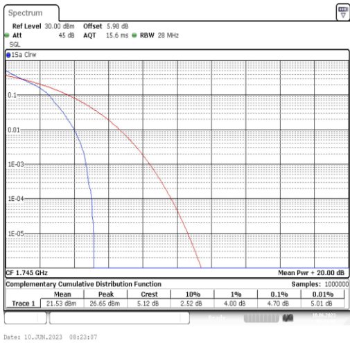
Band66-10MHz-QPSK-132322-1RB#0
