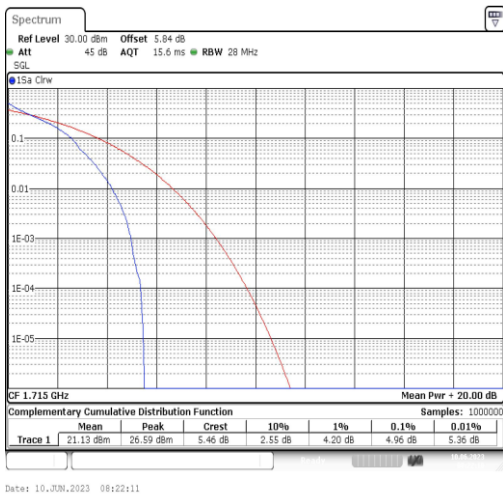
Band66-10MHz-QPSK-132022-1RB#0
