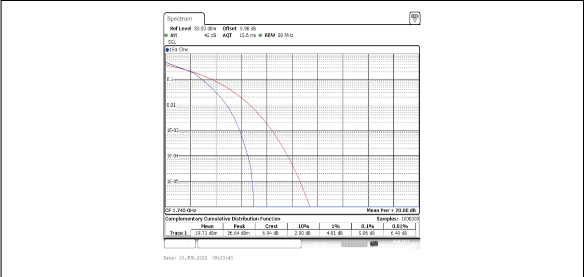
Band66-10MHz-16QAM-132322-50RB#0
