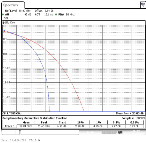
Band66-3MHz-16QAM-132657-15RB#0
