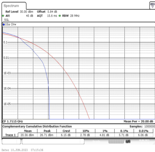
Band66-3MHz-16QAM-131987-1RB#0
