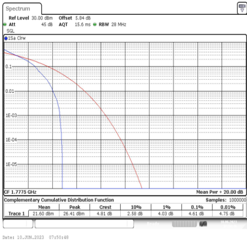
Band66-5MHz-QPSK-132647-1RB#0
