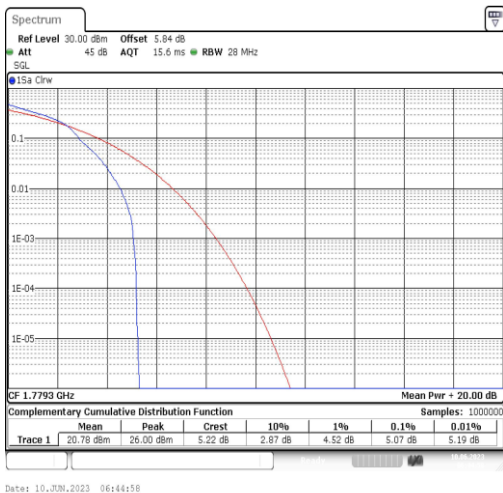
Band66-1.4MHz-16QAM-132665-1RB#0
