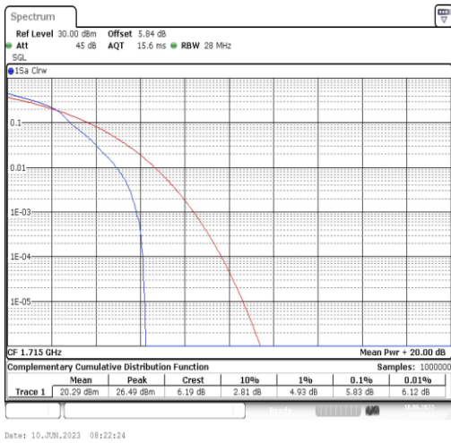
Band66-10MHz-16QAM-132022-1RB#0
