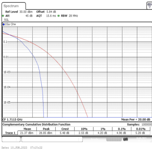
Band66-3MHz-QPSK-131987-1RB#0
