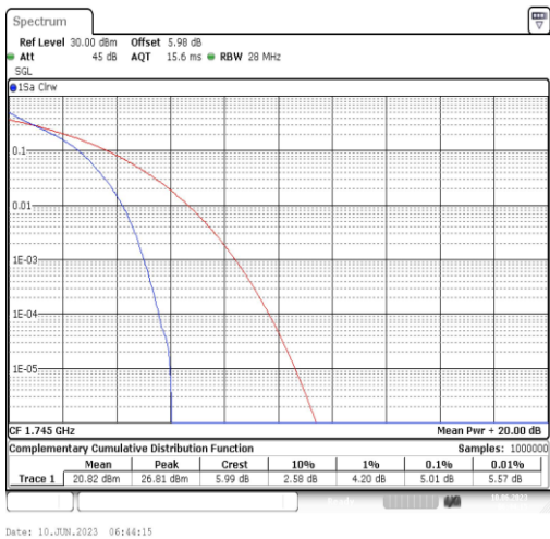
Band66-1.4MHz-QPSK-132322-6RB#0
