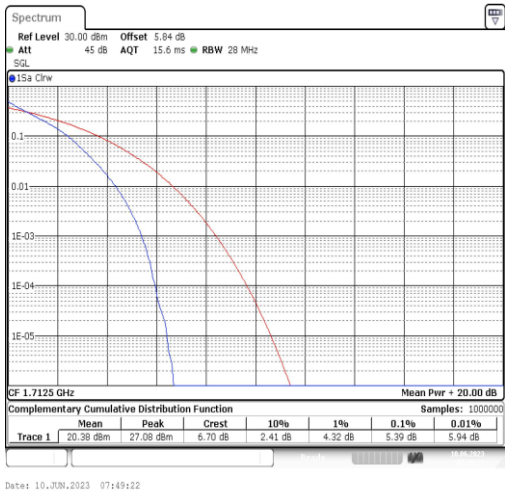
Band66-5MHz-QPSK-131997-25RB#0
