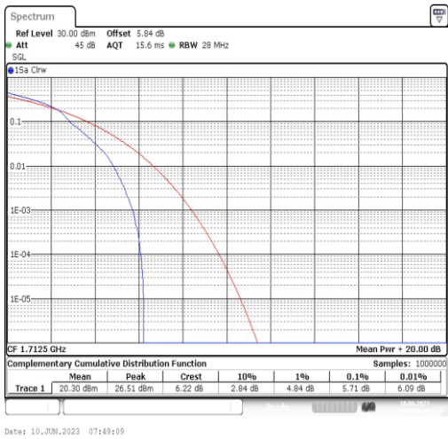
Band66-5MHz-16QAM-131997-1RB#0
