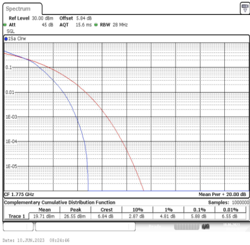
Band66-10MHz-16QAM-132622-50RB#0
