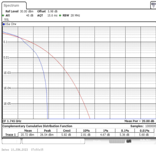
Band66-5MHz-16QAM-132322-1RB#0
