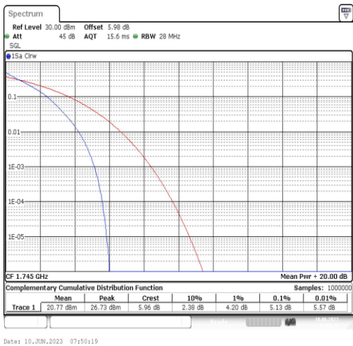
Band66-5MHz-QPSK-132322-25RB#0
