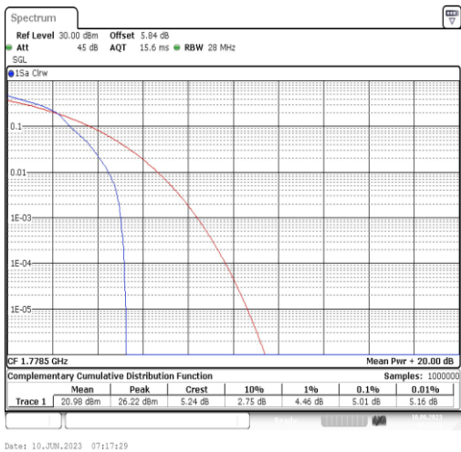
Band66-3MHz-16QAM-132657-1RB#0
