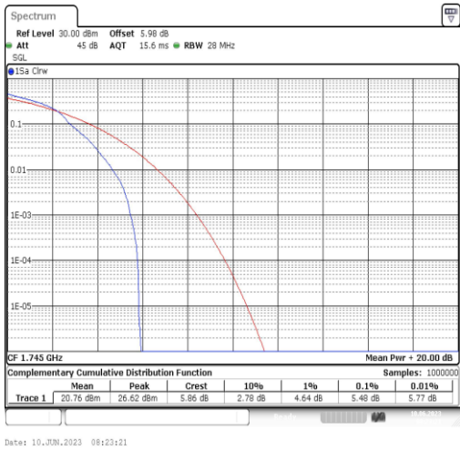
Band66-10MHz-16QAM-132322-1RB#0
