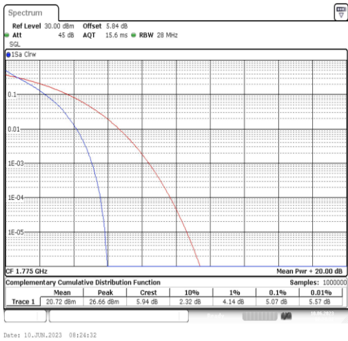
Band66-10MHz-QPSK-132622-50RB#0
