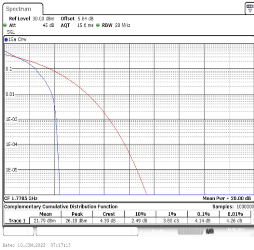
Band66-3MHz-QPSK-132657-1RB#0
