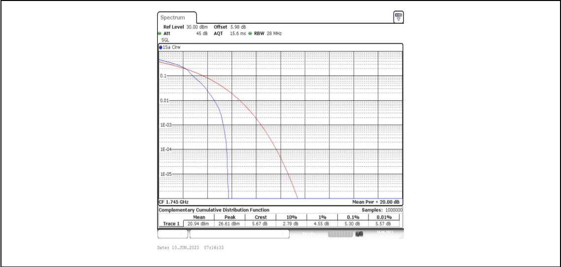
Band66-3MHz-16QAM-132322-1RB#0
