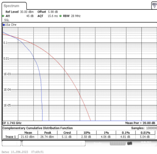
Band66-5MHz-QPSK-132322-1RB#0
