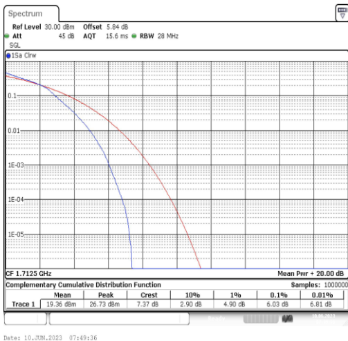
Band66-5MHz-16QAM-131997-25RB#0
