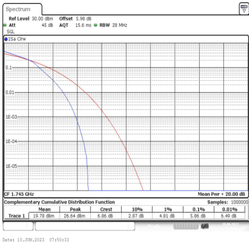
Band66-5MHz-16QAM-132322-25RB#0
