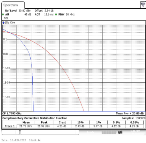
Band66-1.4MHz-QPSK-132665-1RB#0
