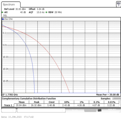
Band66-3MHz-QPSK-132657-15RB#0
