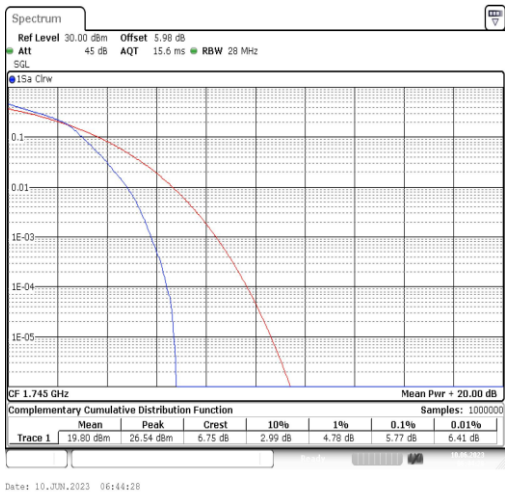
Band66-1.4MHz-16QAM-132322-6RB#0
