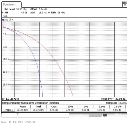
Band66-3MHz-QPSK-131987-15RB#0
