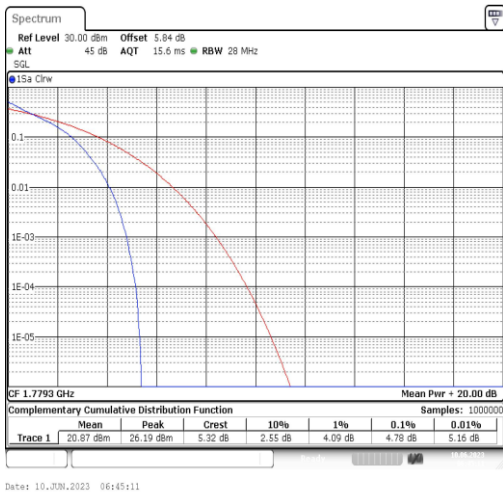
Band66-1.4MHz-QPSK-132665-6RB#0
