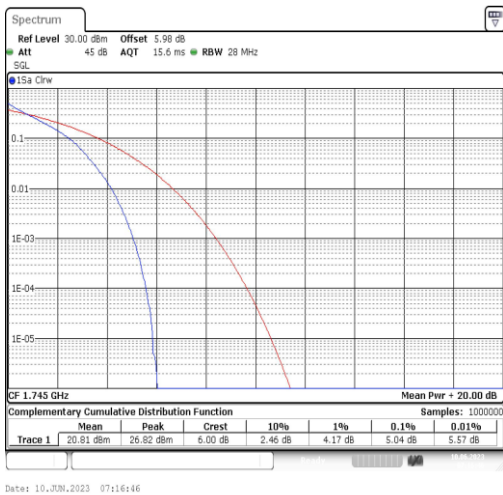
Band66-3MHz-QPSK-132322-15RB#0
