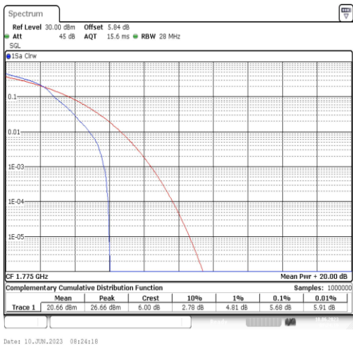
Band66-10MHz-16QAM-132622-1RB#0
