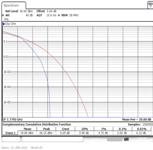
Band66-1.4MHz-16QAM-132665-6RB#0
