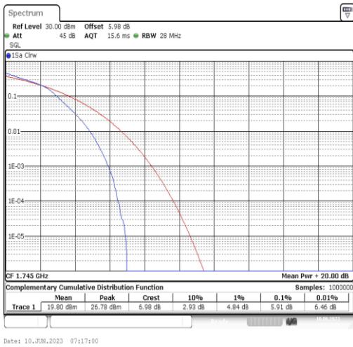
Band66-3MHz-16QAM-132322-15RB#0
