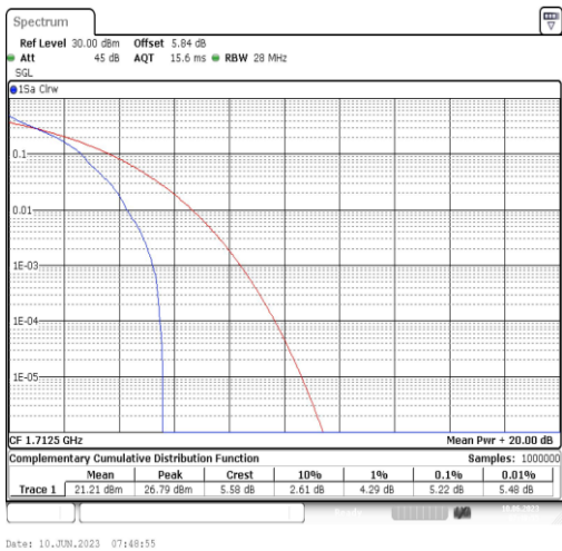
Band66-5MHz-QPSK-131997-1RB#0
