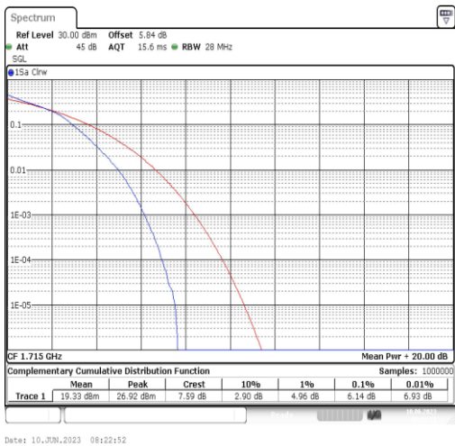
Band66-10MHz-16QAM-132022-50RB#0
