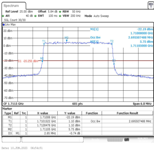
Band66-3MHz-16QAM-131987-15RB#0-2.696
