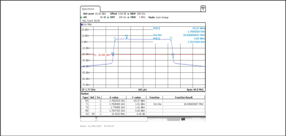
Band66-20MHz-16QAM-132572-100RB#0-18.037
