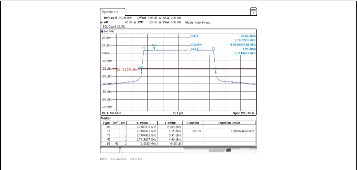
Band66-10MHz-16QAM-132322-50RB#0-8.985
