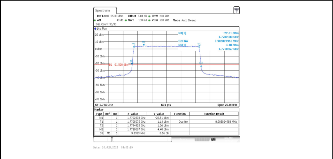
Band66-10MHz-16QAM-132622-50RB#0-8.985
