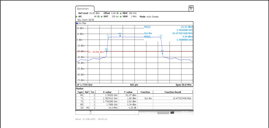
Band66-15MHz-QPSK-132597-75RB#0-13.478
