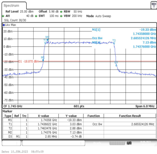
Band66-3MHz-QPSK-132322-15RB#0-2.686
