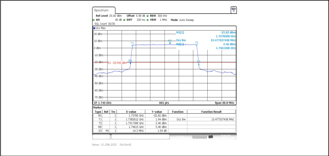
Band66-15MHz-QPSK-132322-75RB#0-13.478
