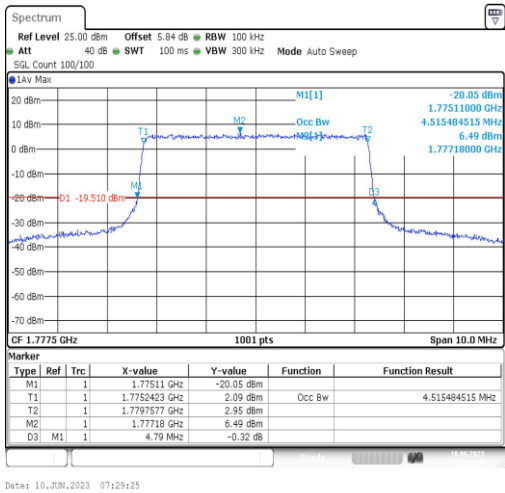
Band66-5MHz-16QAM-132647-25RB#0-4.515
