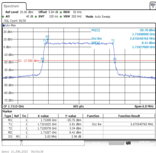
Band66-3MHz-QPSK-131987-15RB#0-2.676
