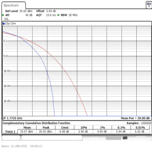
Band66-15MHz-16QAM-132597-75RB#0
