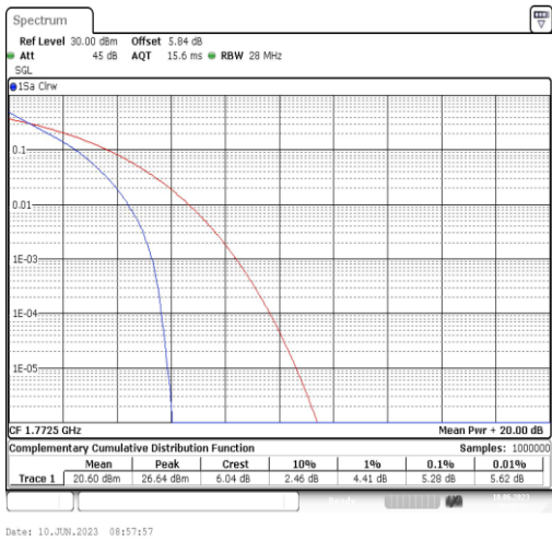
Band66-15MHz-QPSK-132597-75RB#0
