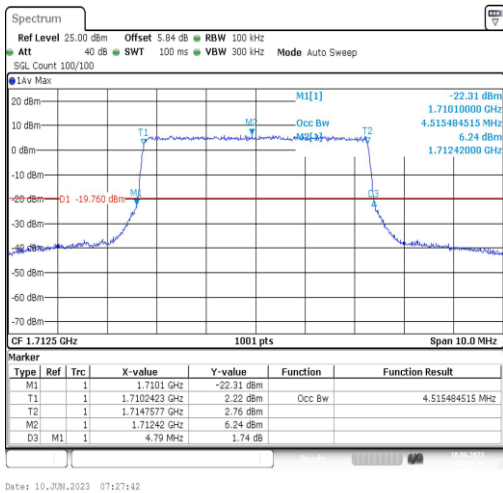
Band66-5MHz-16QAM-131997-25RB#0-4.515
