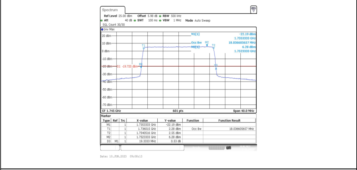
Band66-20MHz-QPSK-132322-100RB#0-18.037
