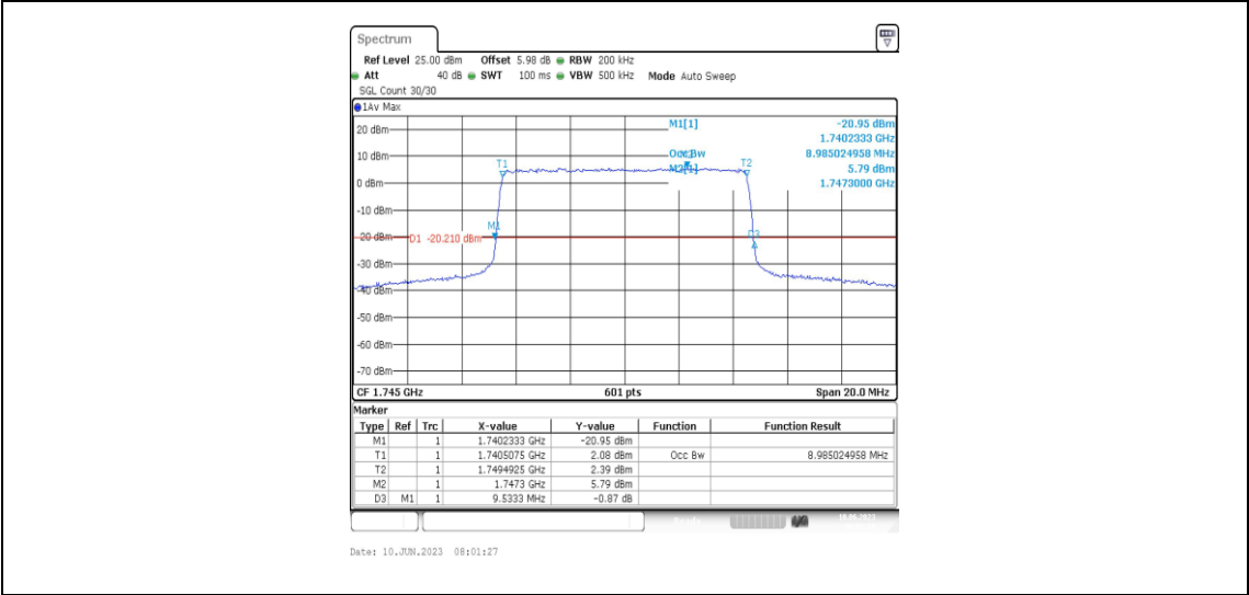
Band66-10MHz-QPSK-132322-50RB#0-8.985
