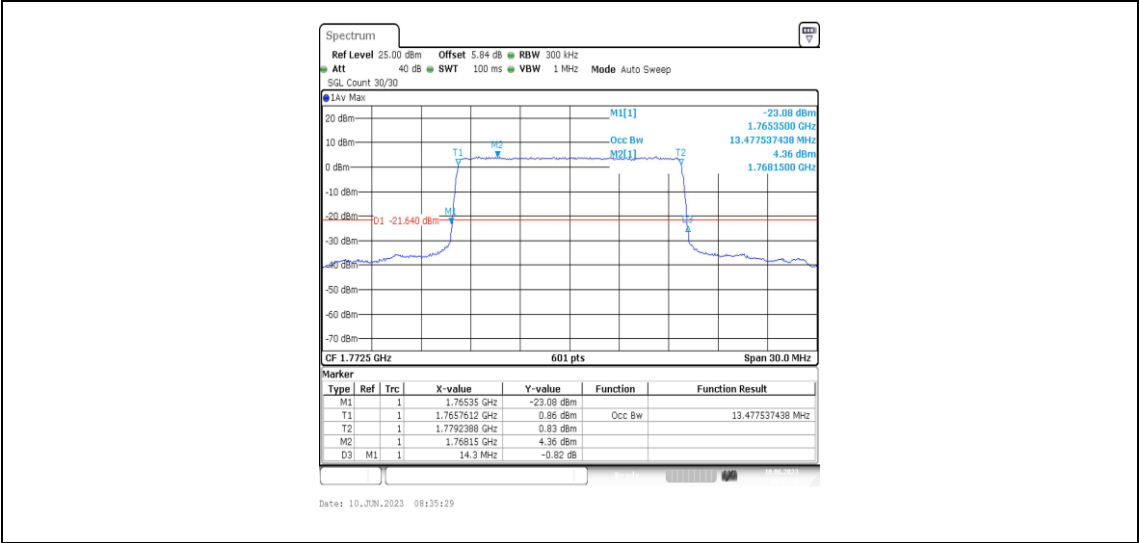
Band66-15MHz-16QAM-132597-75RB#0-13.478
