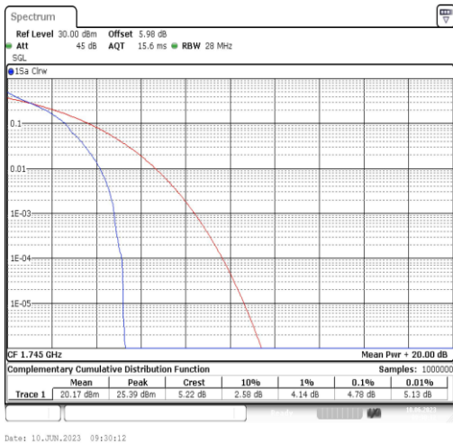
Band66-20MHz-QPSK-132322-1RB#0
