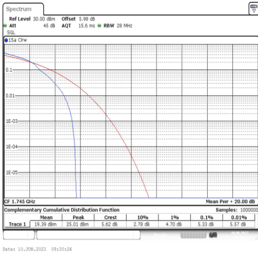
Band66-20MHz-16QAM-132322-1RB#0
