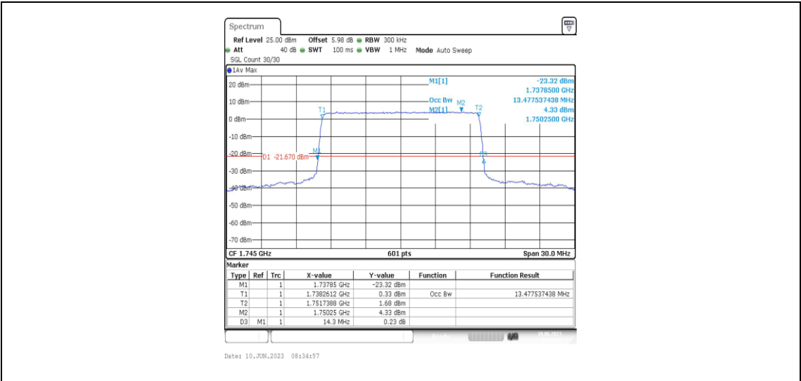
Band66-15MHz-16QAM-132322-75RB#0-13.478
