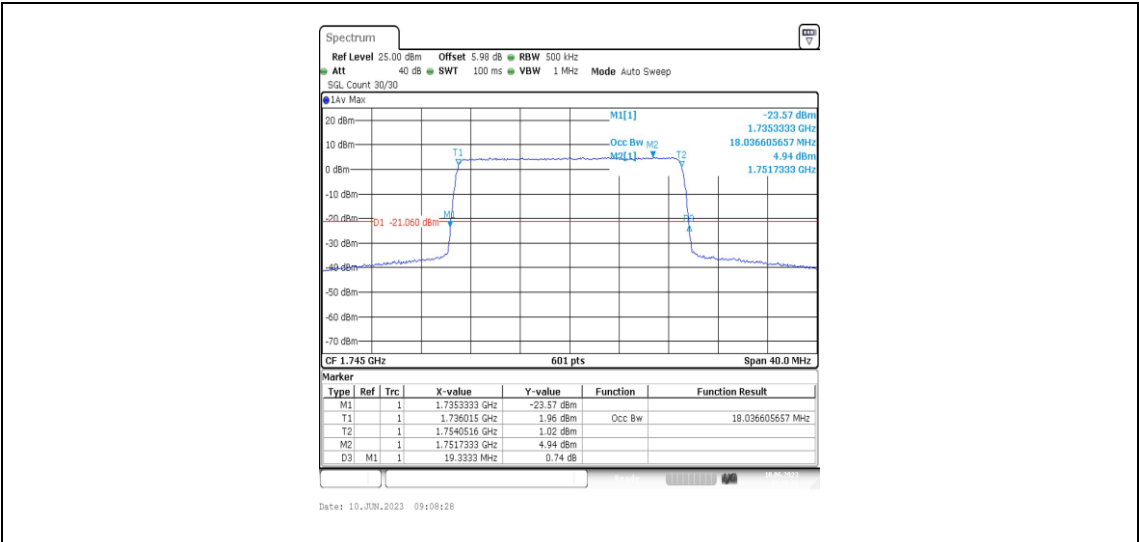
Band66-20MHz-16QAM-132322-100RB#0-18.037
