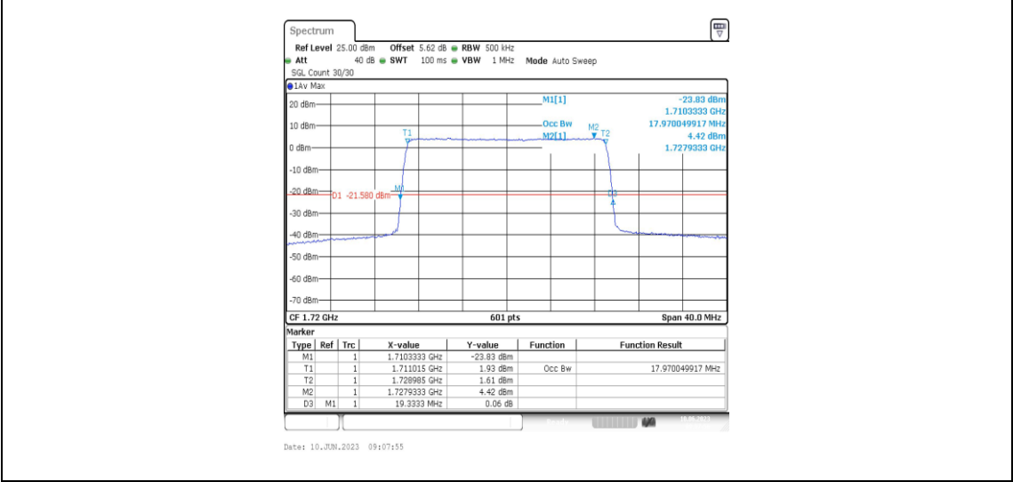
Band66-20MHz-16QAM-132072-100RB#0-17.97
