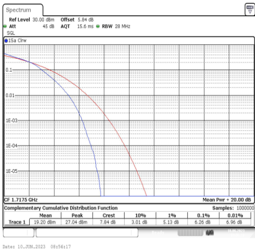
Band66-15MHz-16QAM-132047-75RB#0
