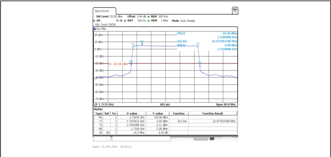
Band66-15MHz-QPSK-132047-75RB#0-13.478
