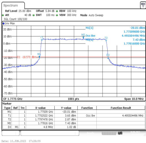
Band66-5MHz-QPSK-132647-25RB#0-4.496
