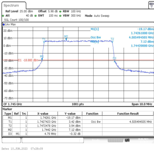
Band66-5MHz-QPSK-132322-25RB#0-4.505
