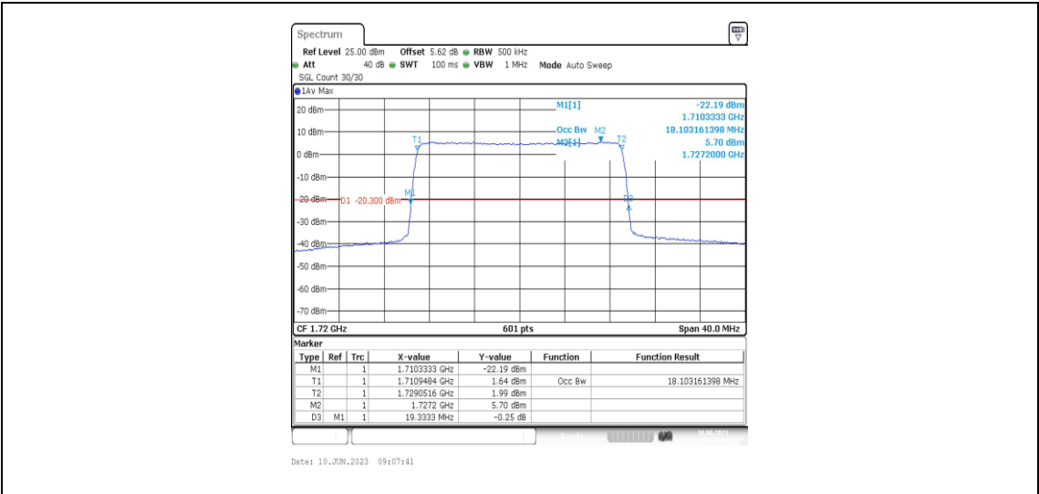
Band66-20MHz-QPSK-132072-100RB#0-18.103
