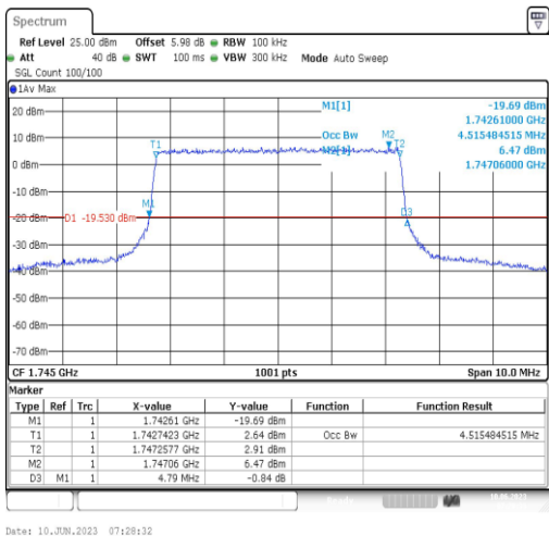
Band66-5MHz-16QAM-132322-25RB#0-4.515
