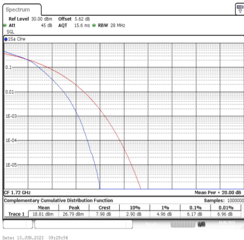
Band66-20MHz-16QAM-132072-100RB#0
