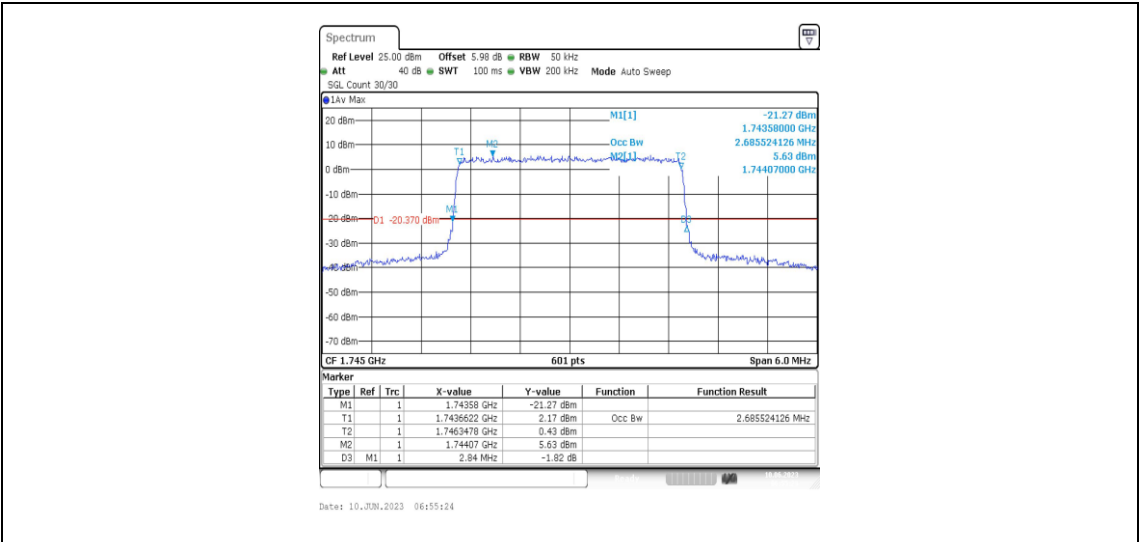
Band66-3MHz-16QAM-132322-15RB#0-2.686
