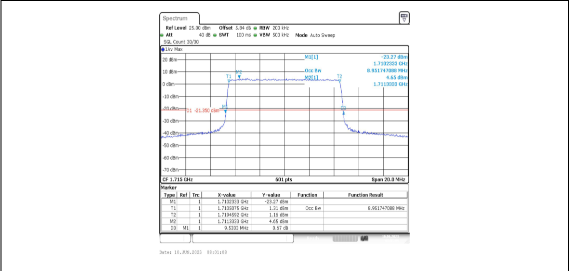
Band66-10MHz-16QAM-132022-50RB#0-8.952
