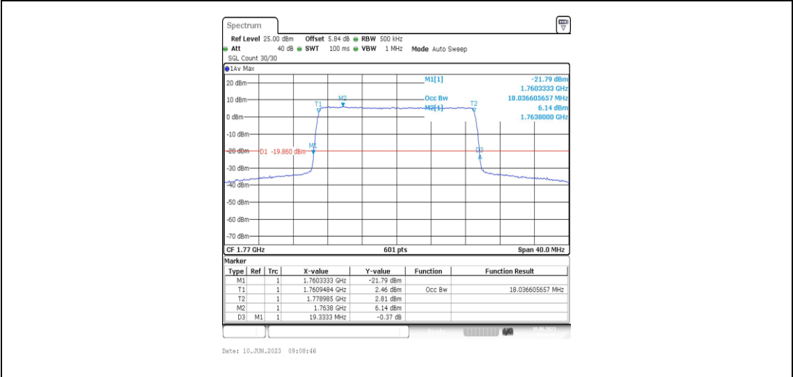
Band66-20MHz-QPSK-132572-100RB#0-18.037
