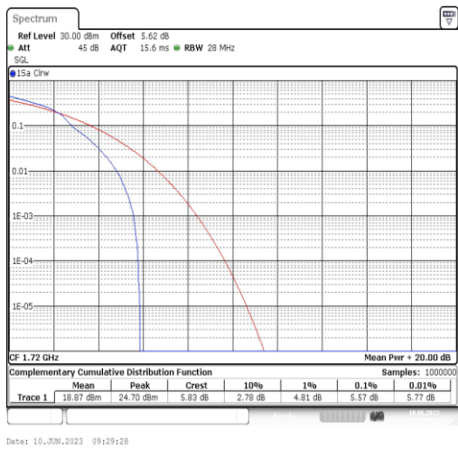
Band66-20MHz-16QAM-132072-1RB#0
