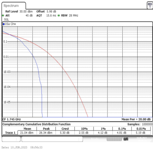
Band66-15MHz-QPSK-132322-1RB#0
