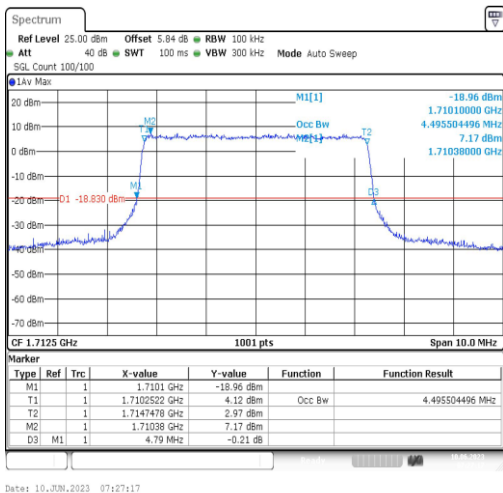
Band66-5MHz-QPSK-131997-25RB#0-4.496
