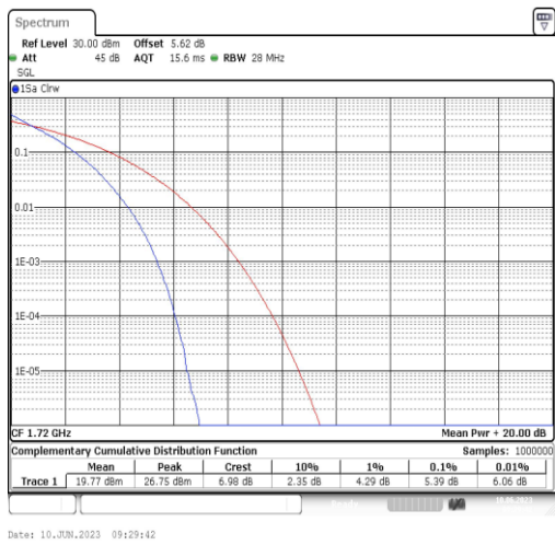
Band66-20MHz-QPSK-132072-100RB#0
