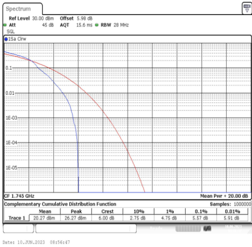
Band66-15MHz-16QAM-132322-1RB#0
