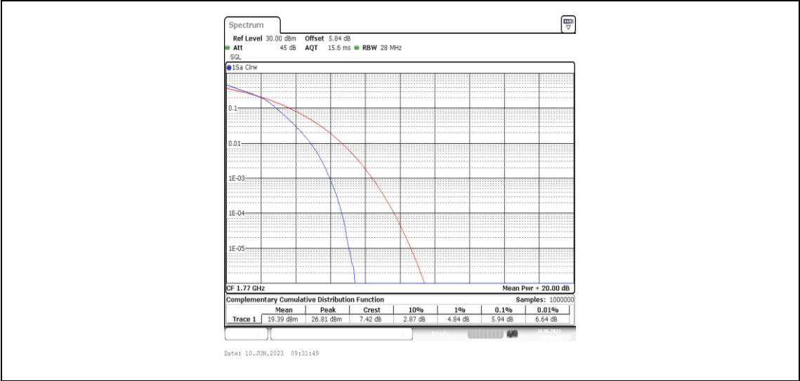
Band66-20MHz-16QAM-132572-100RB#0
