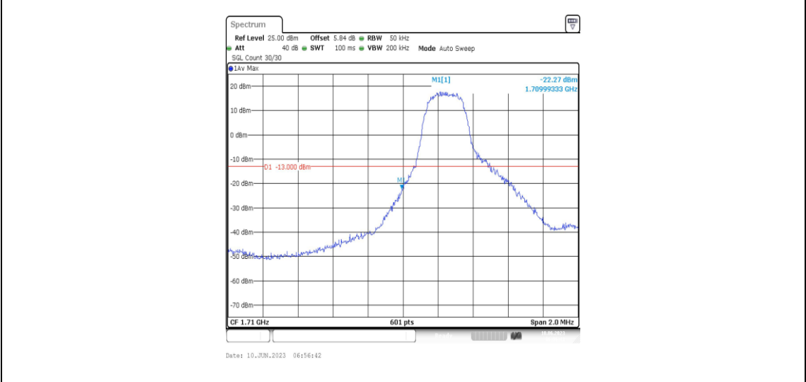
Band66-3MHz-16QAM-131987-1RB#0
