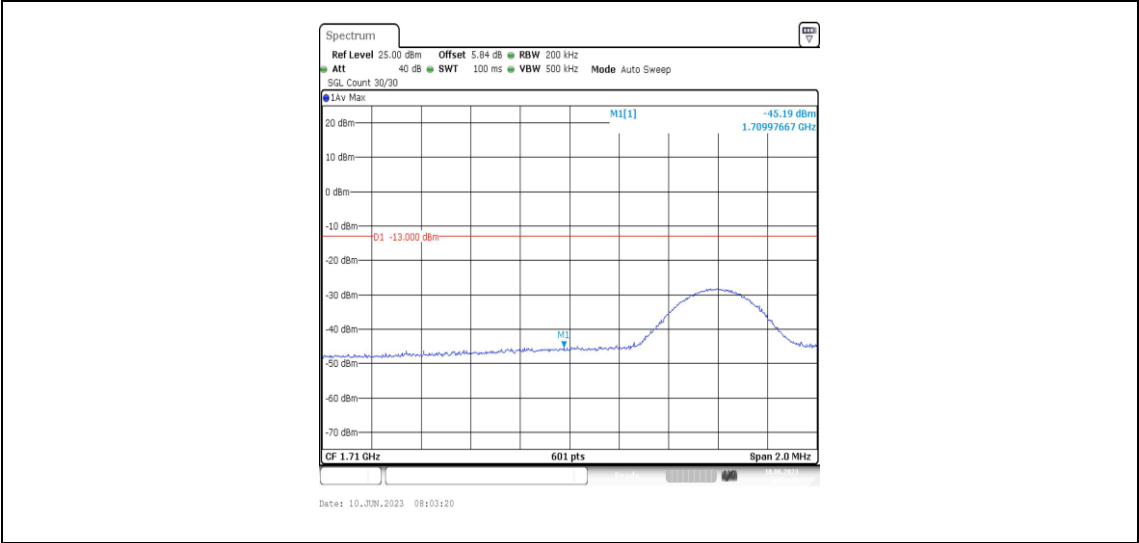
Band66-10MHz-QPSK-132022-1RB#49
