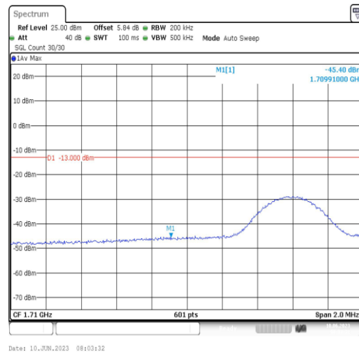
Band66-10MHz-16QAM-132022-1RB#49
