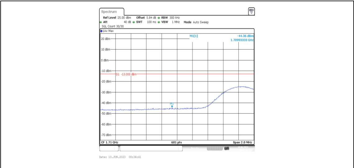
Band66-15MHz-16QAM-132047-1RB#74
