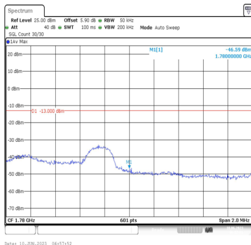
Band66-3MHz-QPSK-132657-1RB#0
