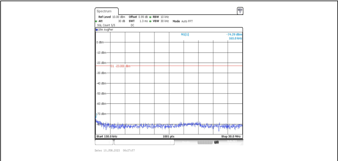
Band66-1.4MHz-16QAM-131979-1RB#0-Range2:0.15~30MHz
