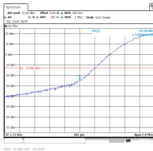
Band66-20MHz-16QAM-132072-1RB#0
