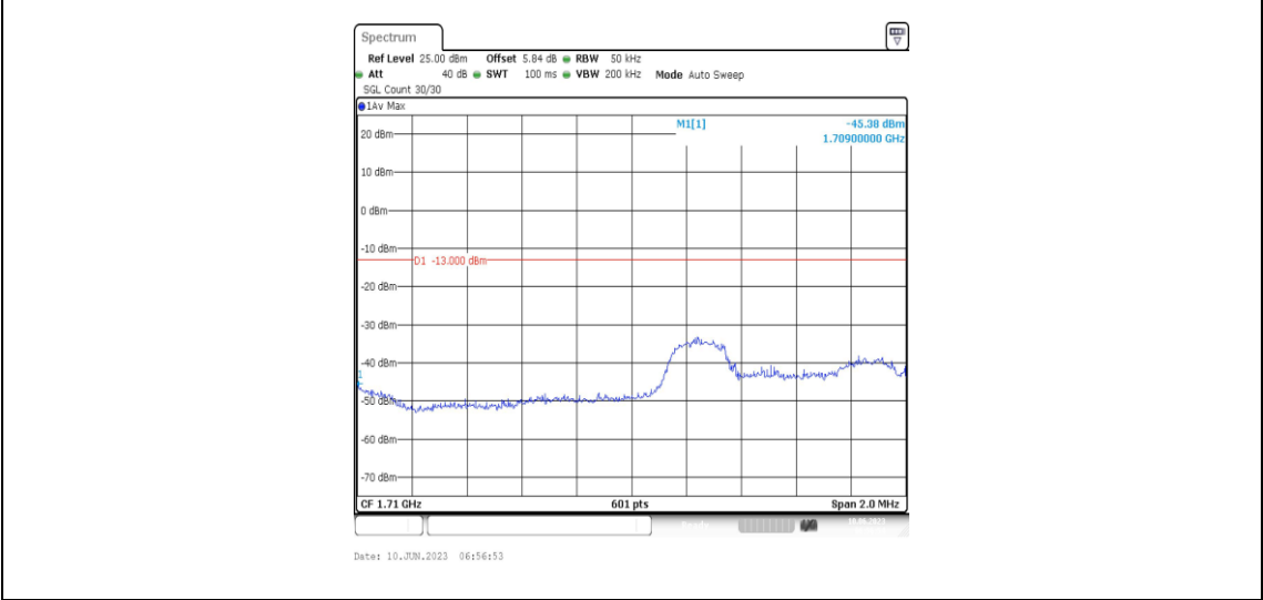
Band66-3MHz-QPSK-131987-1RB#14
