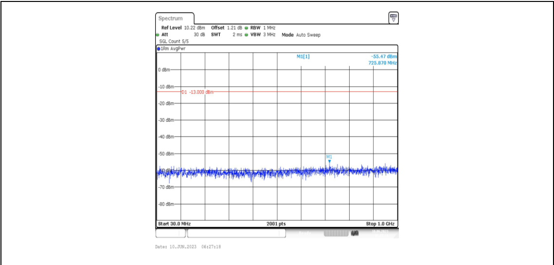
Band66-1.4MHz-QPSK-131979-1RB#0-Range3:30~1000MHz
