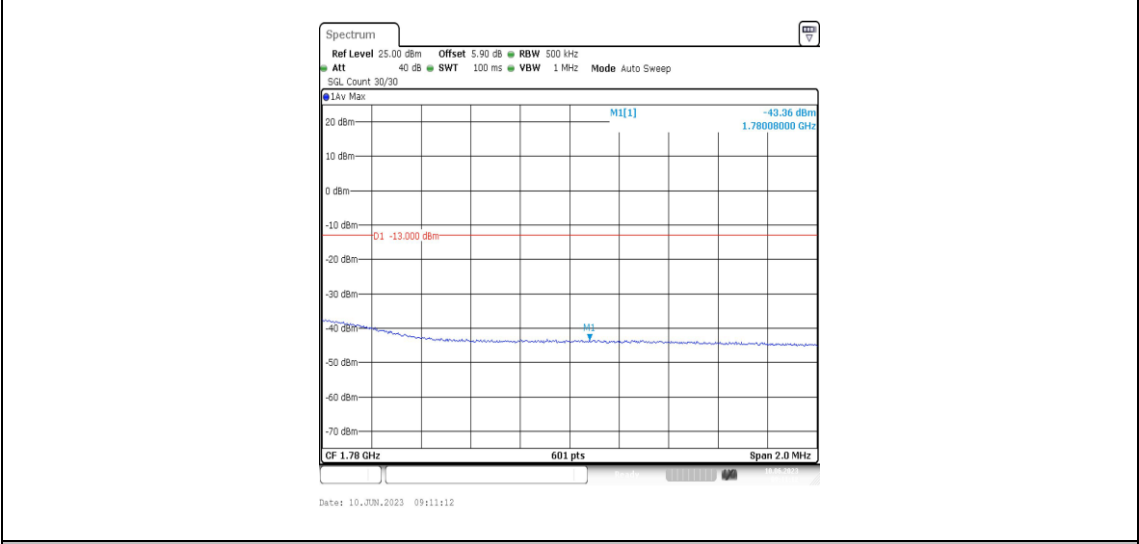
Band66-20MHz-16QAM-132572-1RB#0
