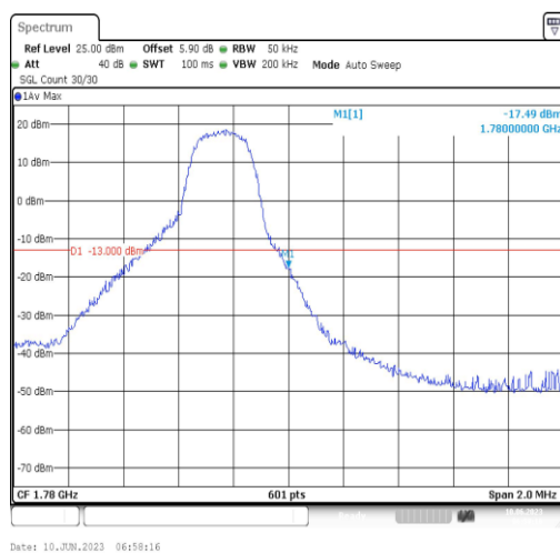
Band66-3MHz-QPSK-132657-1RB#14
