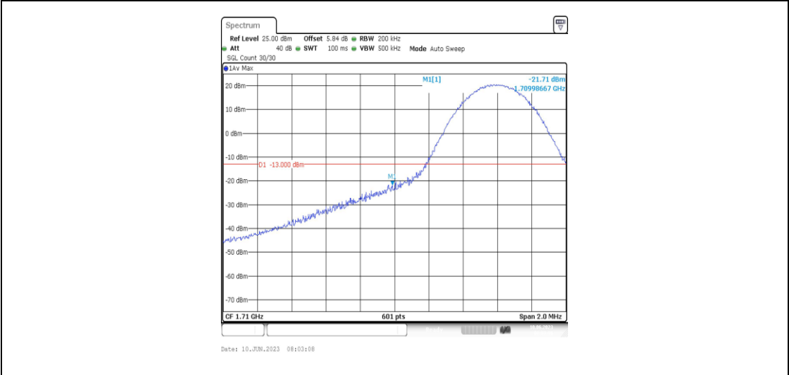
Band66-10MHz-16QAM-132022-1RB#0
