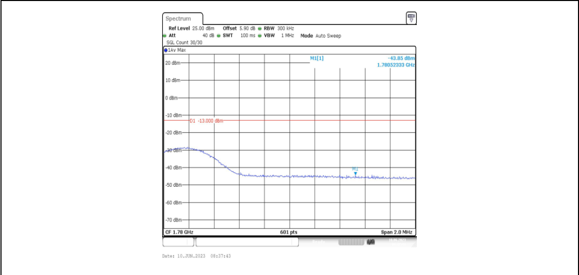
Band66-15MHz-16QAM-132597-1RB#0
