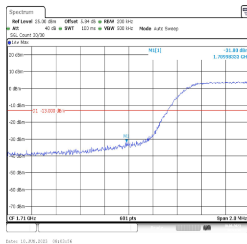
Band66-10MHz-16QAM-132022-50RB#0
