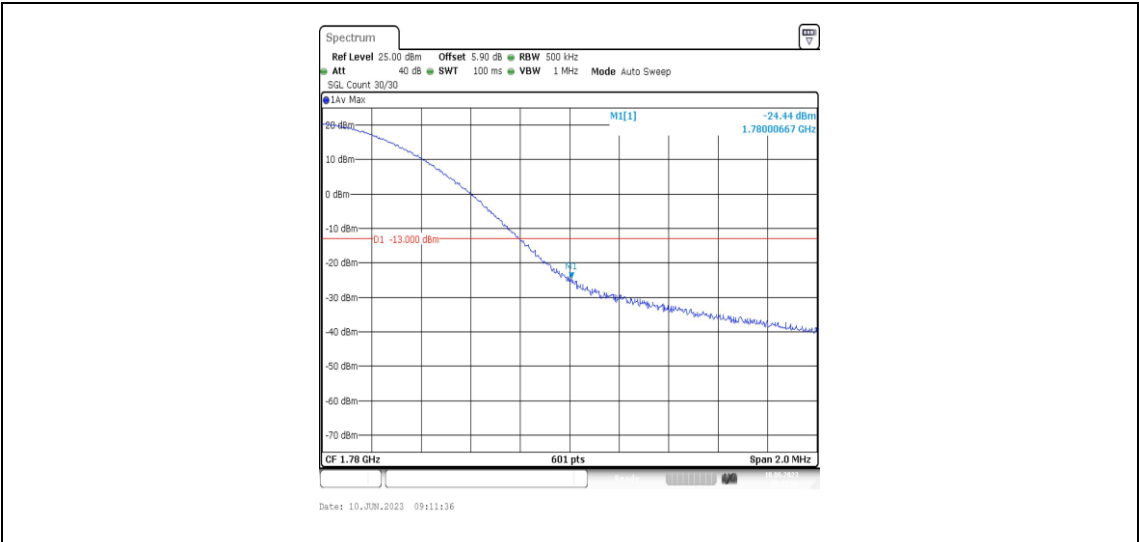
Band66-20MHz-16QAM-132572-1RB#99
