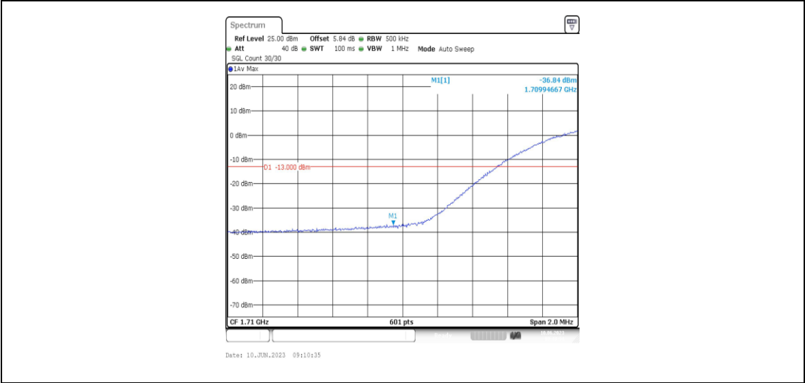
Band66-20MHz-16QAM-132072-100RB#0
