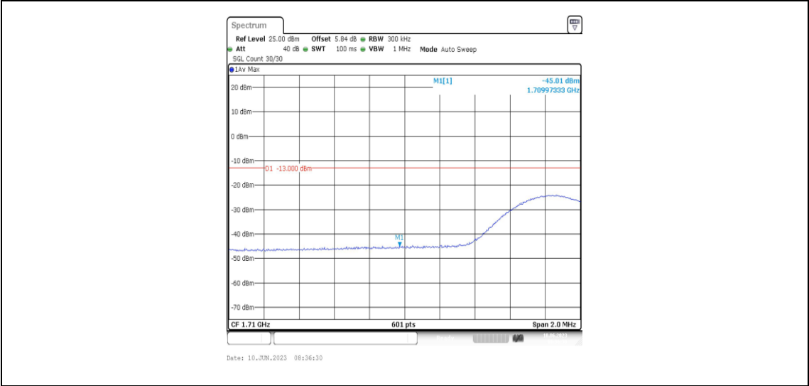
Band66-15MHz-QPSK-132047-1RB#74
