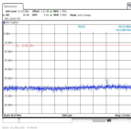
Band66-3MHz-16QAM-132657-1RB#0-Range3:30~1000MHz
