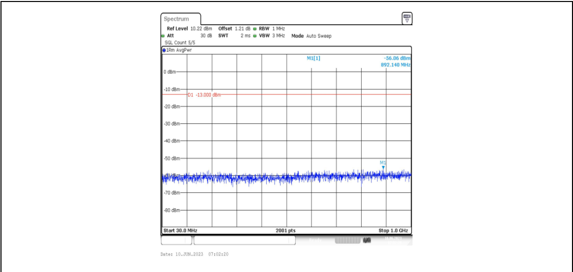
Band66-3MHz-16QAM-132322-1RB#0-Range3:30~1000MHz
