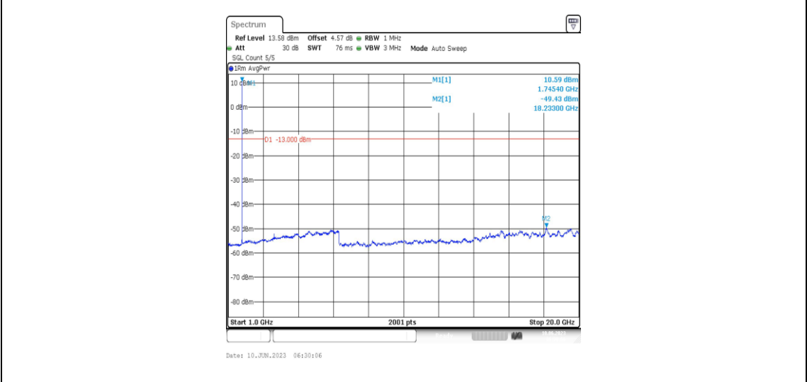
Band66-1.4MHz-16QAM-132322-1RB#0-Range4:1000~20000MHz
