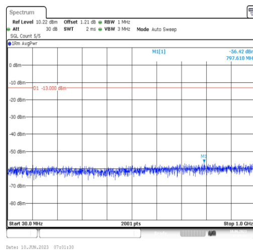
Band66-3MHz-QPSK-132322-1RB#0-Range3:30~1000MHz
