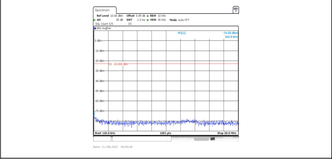
Band66-1.4MHz-QPSK-132322-1RB#0-Range2:0.15~30MHz
