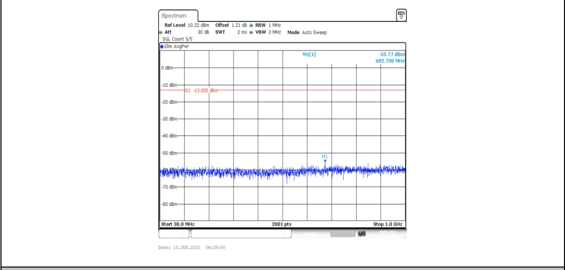
Band66-1.4MHz-QPSK-132322-1RB#0-Range3:30~1000MHz
