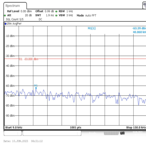
Band66-1.4MHz-16QAM-132665-1RB#0-Range1:0.009~0.15MHz
