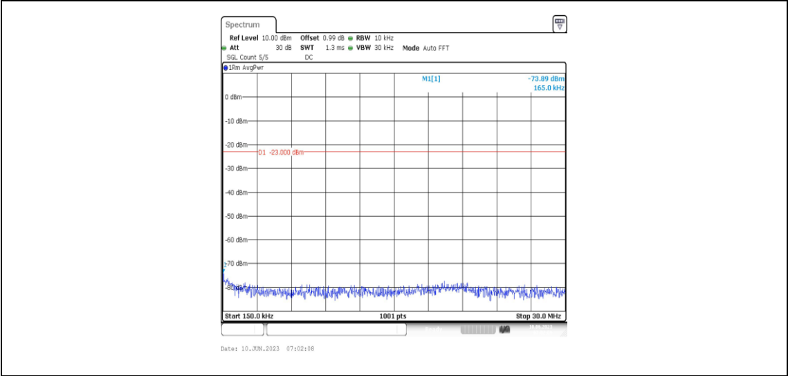
Band66-3MHz-16QAM-132322-1RB#0-Range2:0.15~30MHz
