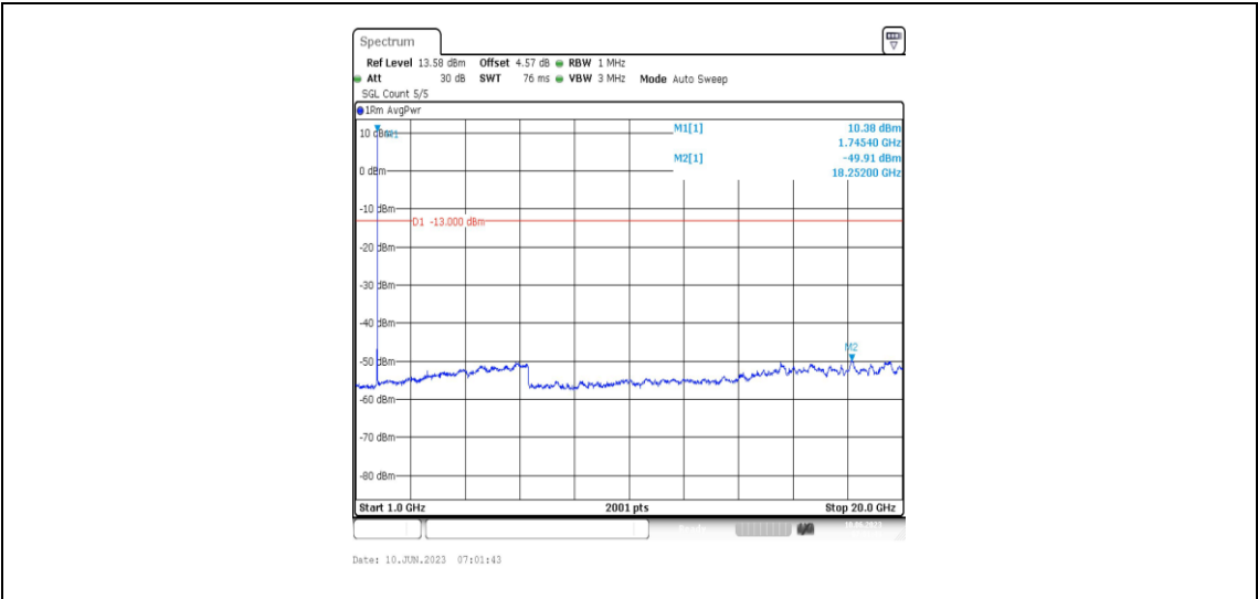
Band66-3MHz-QPSK-132322-1RB#0-Range4:1000~20000MHz
