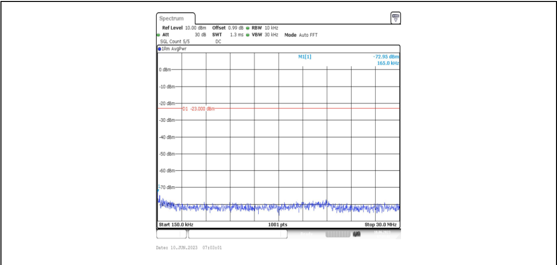
Band66-3MHz-QPSK-132657-1RB#0-Range2:0.15~30MHz
