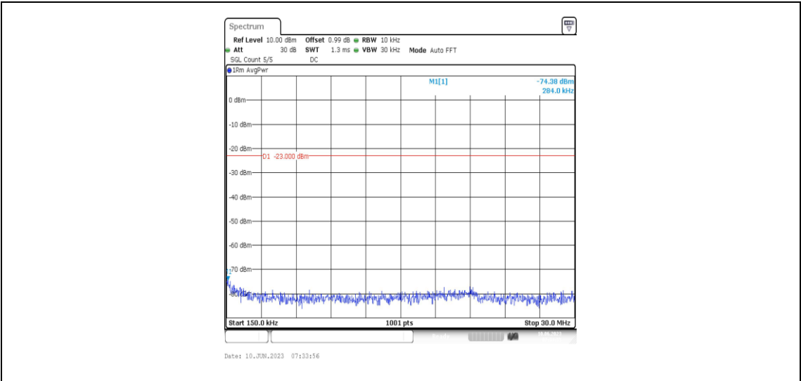
Band66-5MHz-16QAM-131997-1RB#0-Range2:0.15~30MHz
