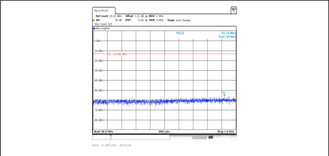
Band66-1.4MHz-QPSK-132665-1RB#0-Range3:30~1000MHz
