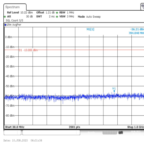
Band66-1.4MHz-16QAM-132665-1RB#0-Range3:30~1000MHz
