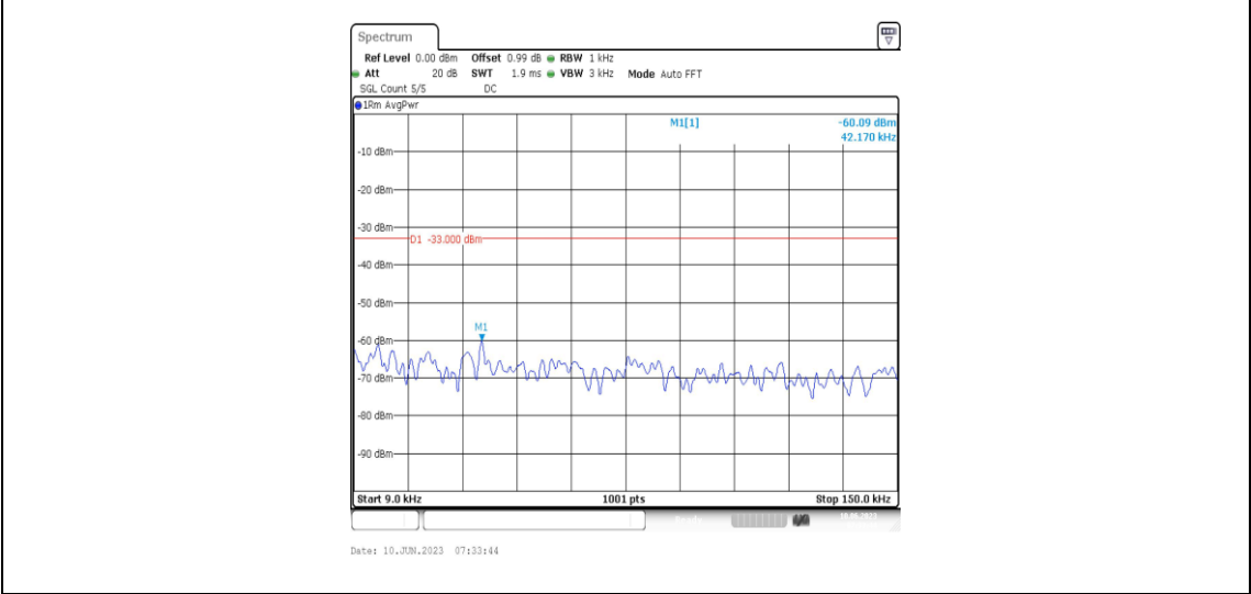
Band66-5MHz-16QAM-131997-1RB#0-Range1:0.009~0.15MHz
