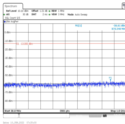
Band66-5MHz-QPSK-132322-1RB#0-Range3:30~1000MHz
