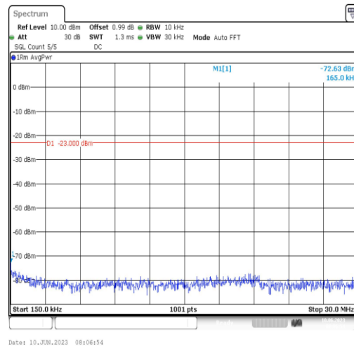
Band66-10MHz-16QAM-132022-1RB#0-Range2:0.15~30MHz
