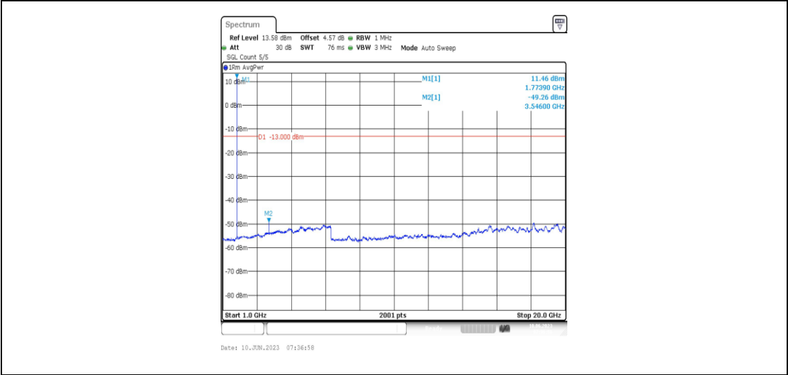
Band66-5MHz-QPSK-132647-1RB#0-Range4:1000~20000MHz
