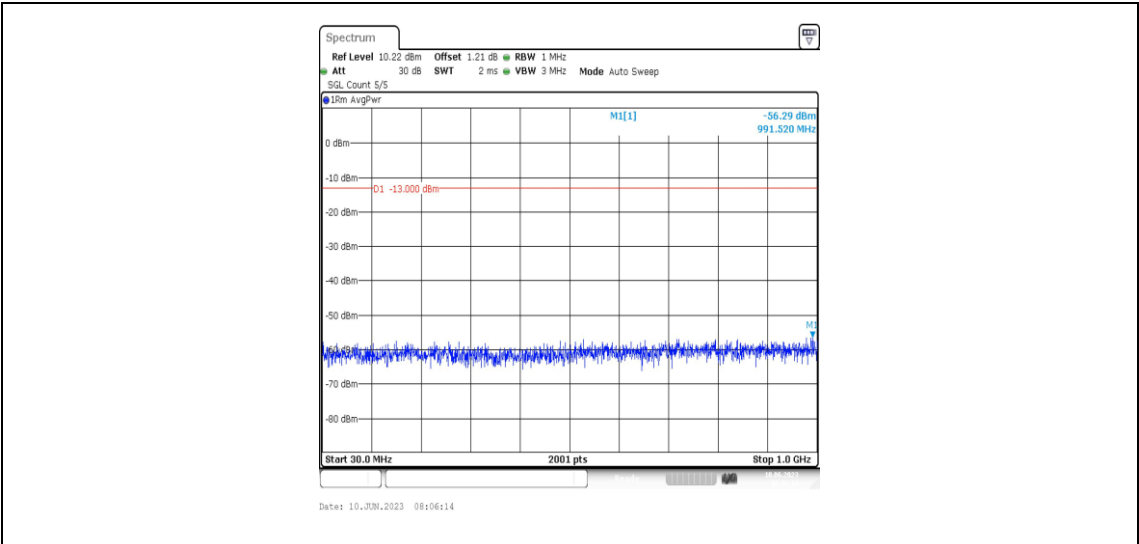
Band66-10MHz-QPSK-132022-1RB#0-Range3:30~1000MHz
