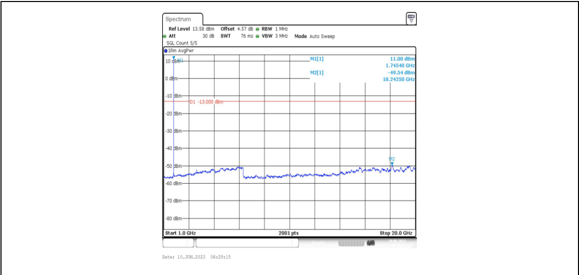
Band66-1.4MHz-QPSK-132322-1RB#0-Range4:1000~20000MHz
