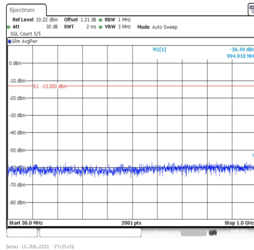
Band66-5MHz-16QAM-132322-1RB#0-Range3:30~1000MHz
