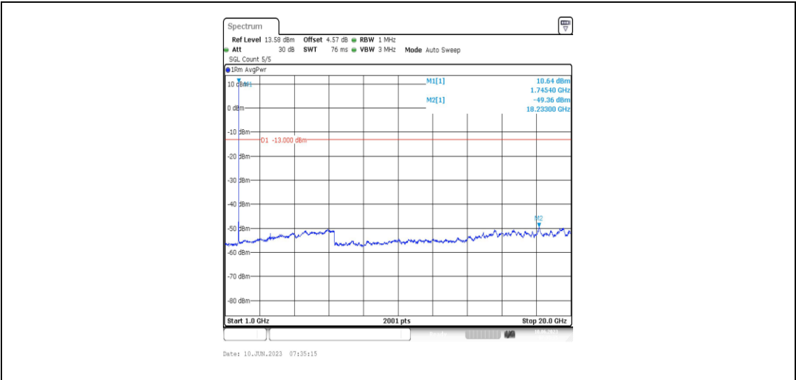
Band66-5MHz-QPSK-132322-1RB#0-Range4:1000~20000MHz
