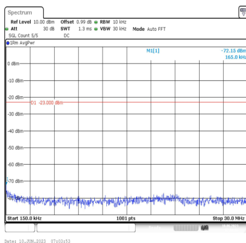
Band66-3MHz-16QAM-132657-1RB#0-Range2:0.15~30MHz
