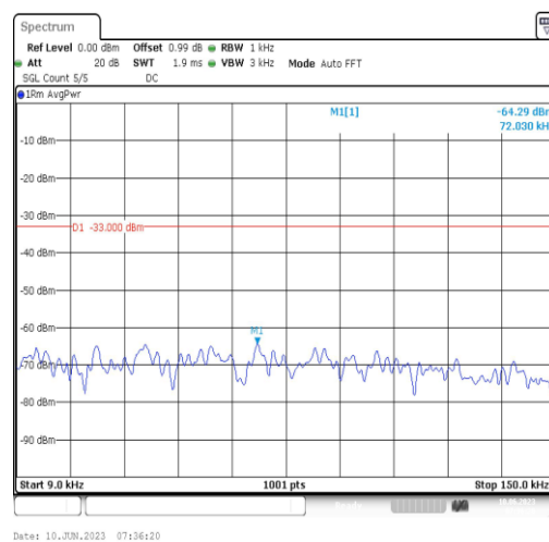
Band66-5MHz-QPSK-132647-1RB#0-Range1:0.009~0.15MHz
