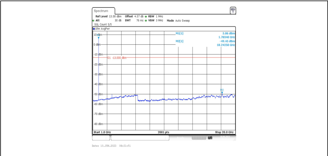
Band66-1.4MHz-16QAM-132665-1RB#0-Range4:1000~20000MHz
