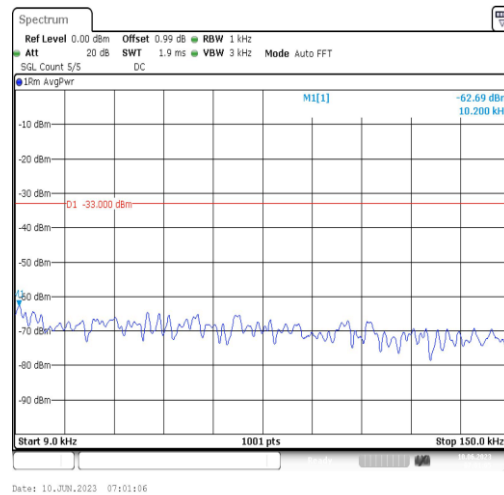
Band66-3MHz-QPSK-132322-1RB#0-Range1:0.009~0.15MHz
