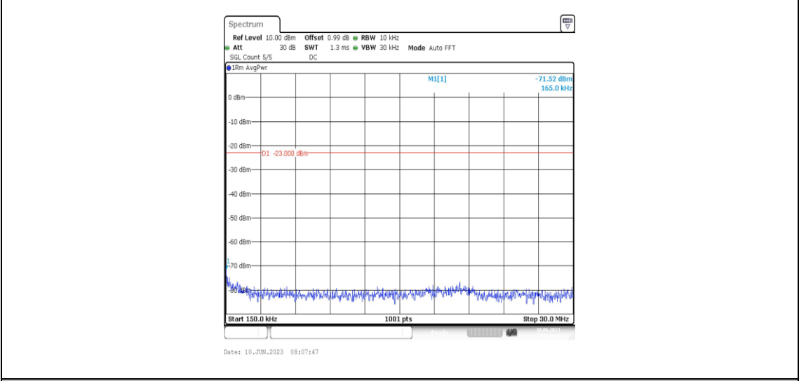
Band66-10MHz-QPSK-132322-1RB#0-Range2:0.15~30MHz
