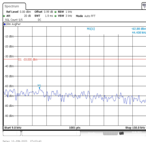
Band66-3MHz-16QAM-132657-1RB#0-Range1:0.009~0.15MHz
