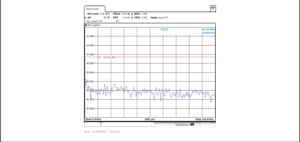
Band66-1.4MHz-QPSK-132665-1RB#0-Range1:0.009~0.15MHz
