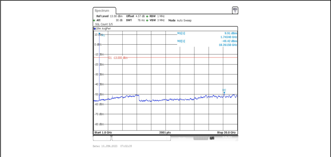
Band66-3MHz-16QAM-132322-1RB#0-Range4:1000~20000MHz
