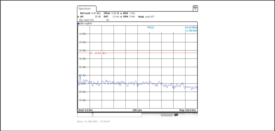
Band66-3MHz-QPSK-132657-1RB#0-Range1:0.009~0.15MHz
