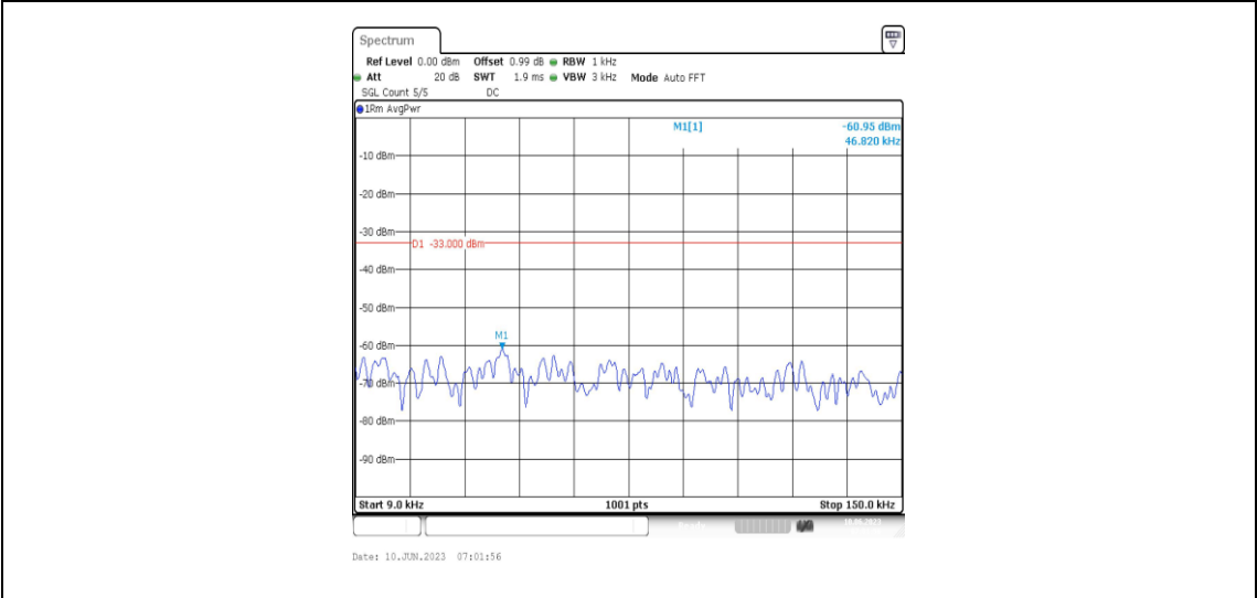
Band66-3MHz-16QAM-132322-1RB#0-Range1:0.009~0.15MHz
