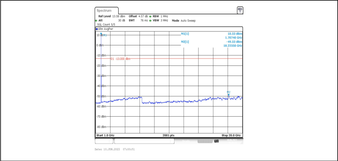
Band66-3MHz-16QAM-131987-1RB#0-Range4:1000~20000MHz
