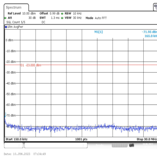
Band66-5MHz-QPSK-132322-1RB#0-Range2:0.15~30MHz
