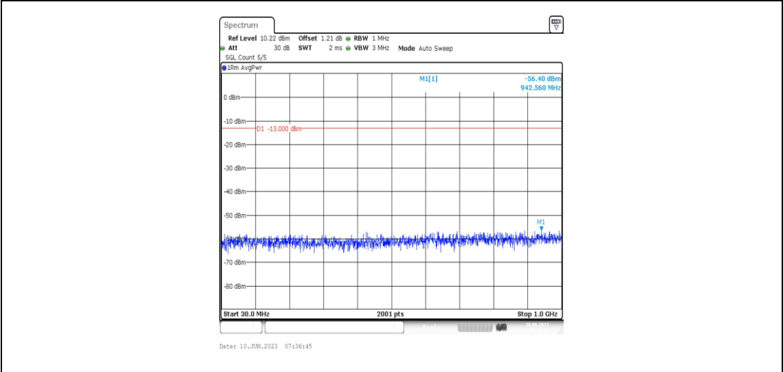
Band66-5MHz-QPSK-132647-1RB#0-Range3:30~1000MHz
