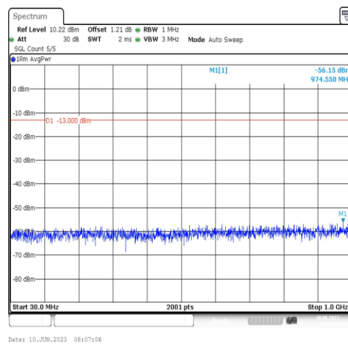
Band66-10MHz-16QAM-132022-1RB#0-Range3:30~1000MHz
