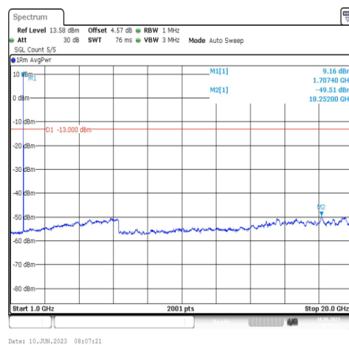
Band66-10MHz-16QAM-132022-1RB#0-Range4:1000~20000MHz
