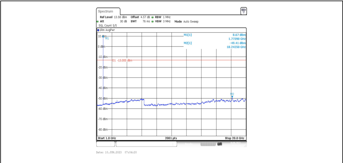
Band66-3MHz-16QAM-132657-1RB#0-Range4:1000~20000MHz
