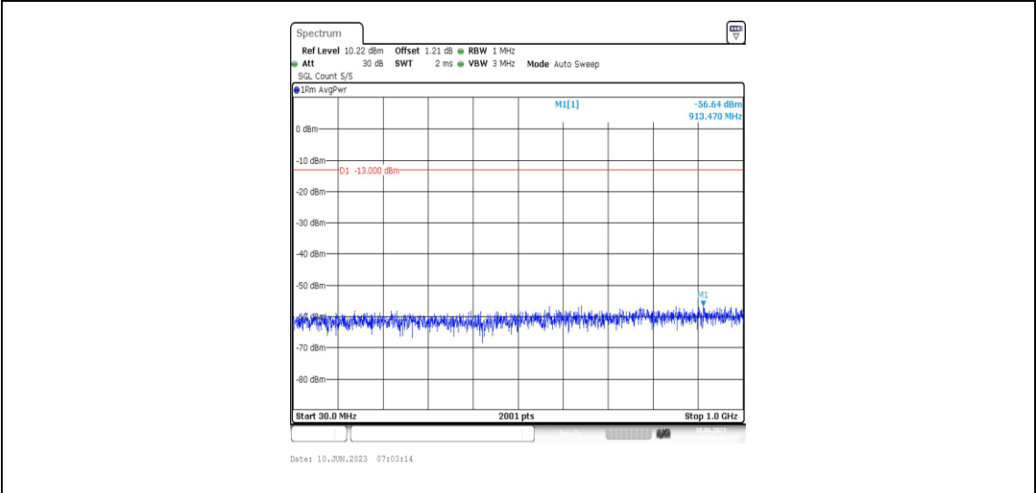
Band66-3MHz-QPSK-132657-1RB#0-Range3:30~1000MHz
