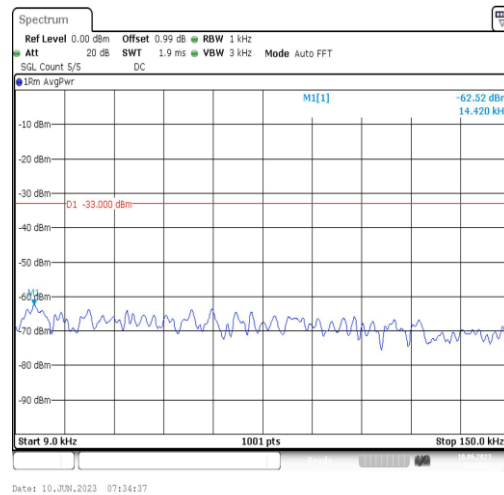
Band66-5MHz-QPSK-132322-1RB#0-Range1:0.009~0.15MHz
