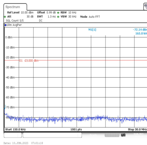
Band66-3MHz-QPSK-132322-1RB#0-Range2:0.15~30MHz
