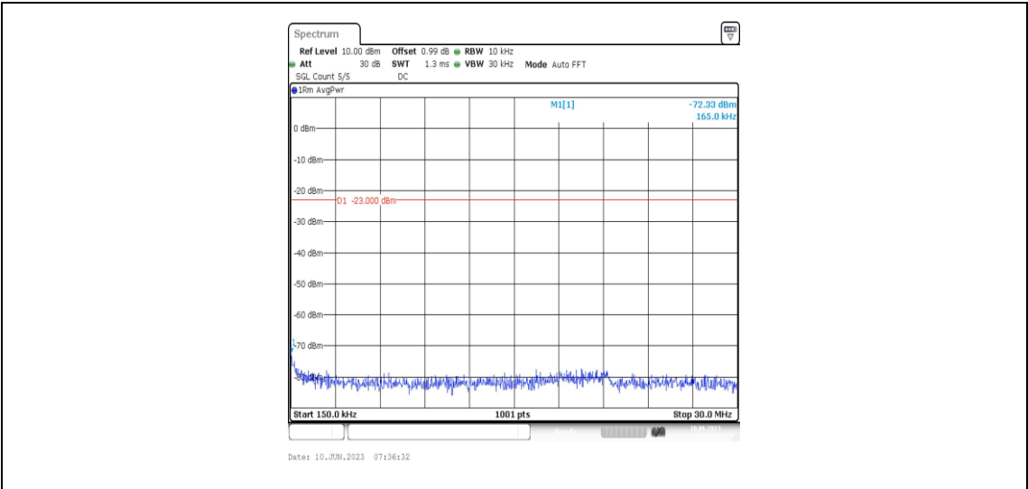
Band66-5MHz-QPSK-132647-1RB#0-Range2:0.15~30MHz
