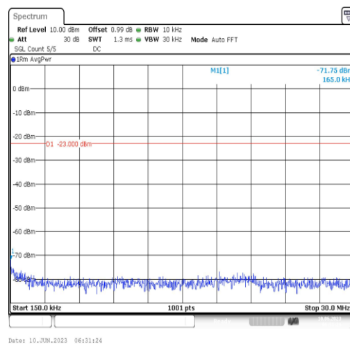
Band66-1.4MHz-16QAM-132665-1RB#0-Range2:0.15~30MHz
