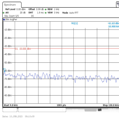
Band66-10MHz-16QAM-132622-1RB#0-Range1:0.009~0.15MHz
