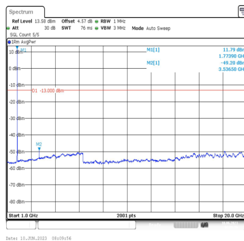
Band66-10MHz-QPSK-132622-1RB#0-Range4:1000~20000MHz
