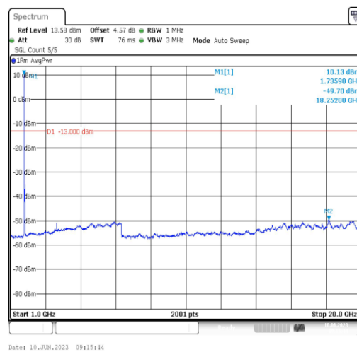
Band66-20MHz-16QAM-132322-1RB#0-Range4:1000~20000MHz
