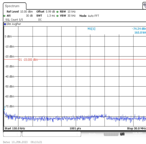
Band66-10MHz-16QAM-132622-1RB#0-Range2:0.15~30MHz
