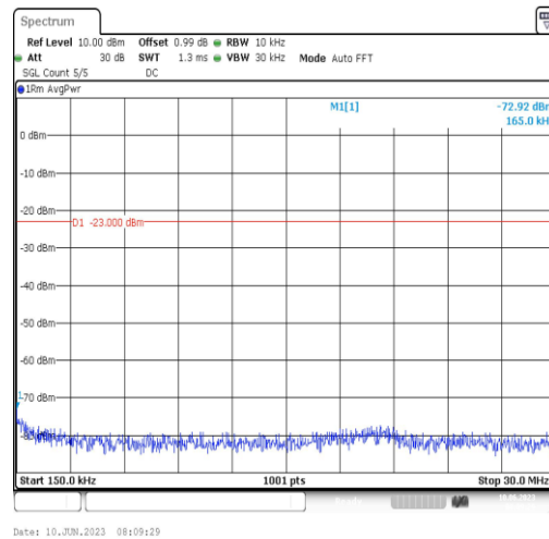
Band66-10MHz-QPSK-132622-1RB#0-Range2:0.15~30MHz
