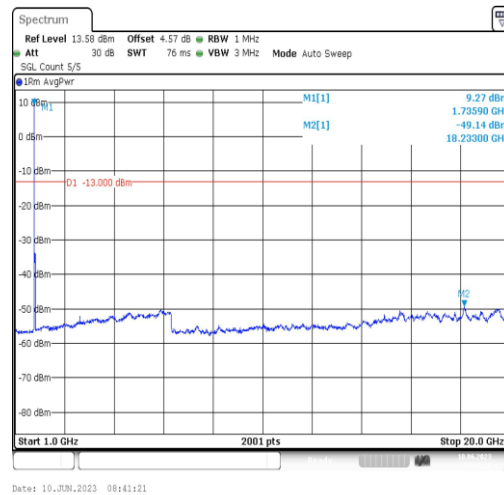
Band66-15MHz-QPSK-132322-1RB#0-Range4:1000~20000MHz
