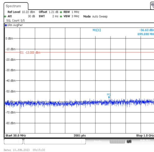
Band66-20MHz-16QAM-132322-1RB#0-Range3:30~1000MHz
