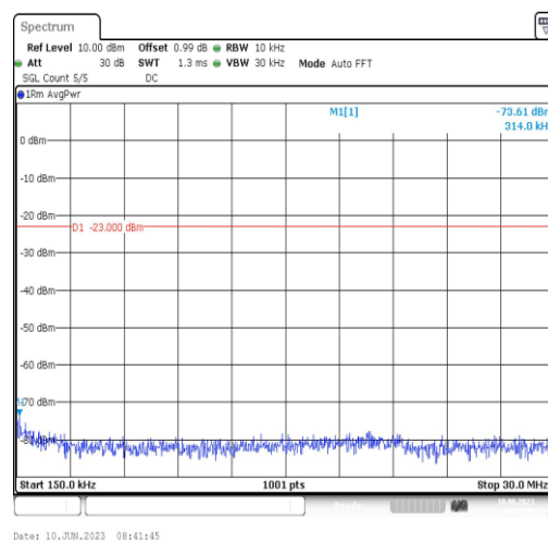
Band66-15MHz-16QAM-132322-1RB#0-Range2:0.15~30MHz
