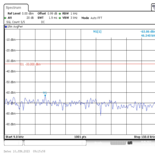
Band66-20MHz-QPSK-132572-1RB#0-Range1:0.009~0.15MHz
