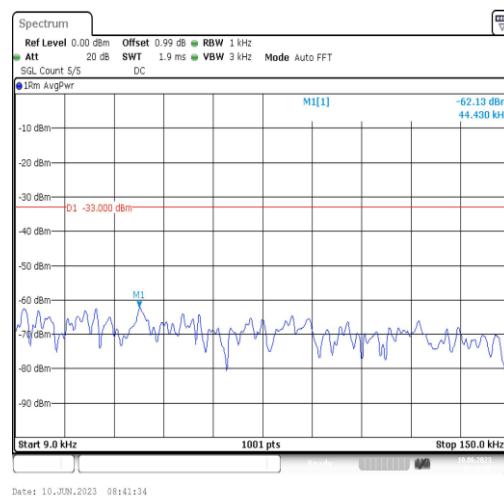
Band66-15MHz-16QAM-132322-1RB#0-Range1:0.009~0.15MHz
