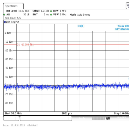
Band66-10MHz-QPSK-132622-1RB#0-Range3:30~1000MHz
