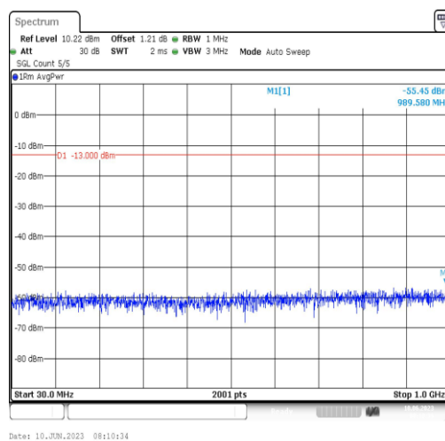
Band66-10MHz-16QAM-132622-1RB#0-Range3:30~1000MHz
