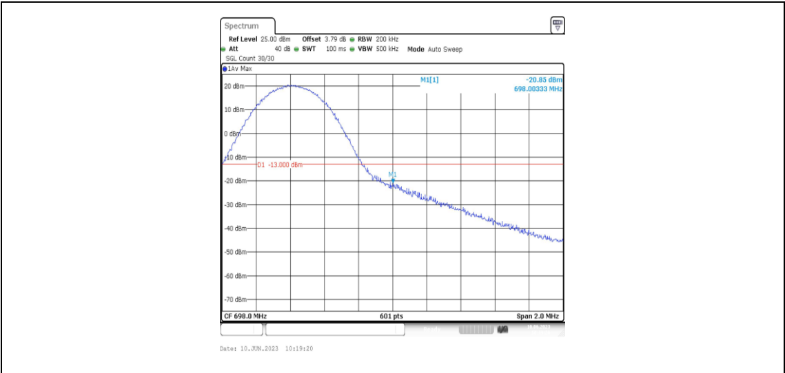
Band71-10MHz-16QAM-133422-1RB#49
