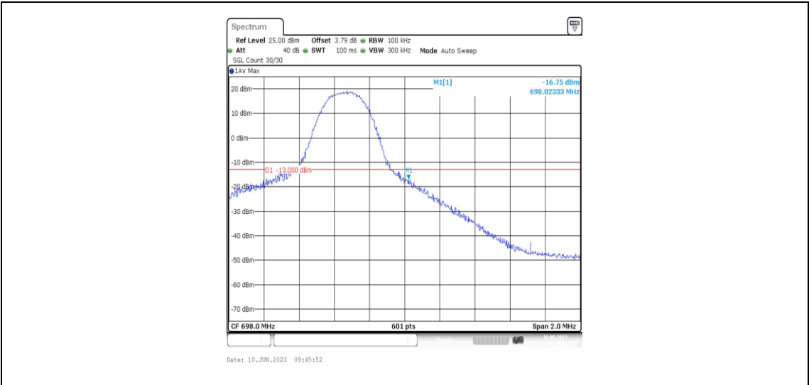
Band71-5MHz-16QAM-133447-1RB#24
