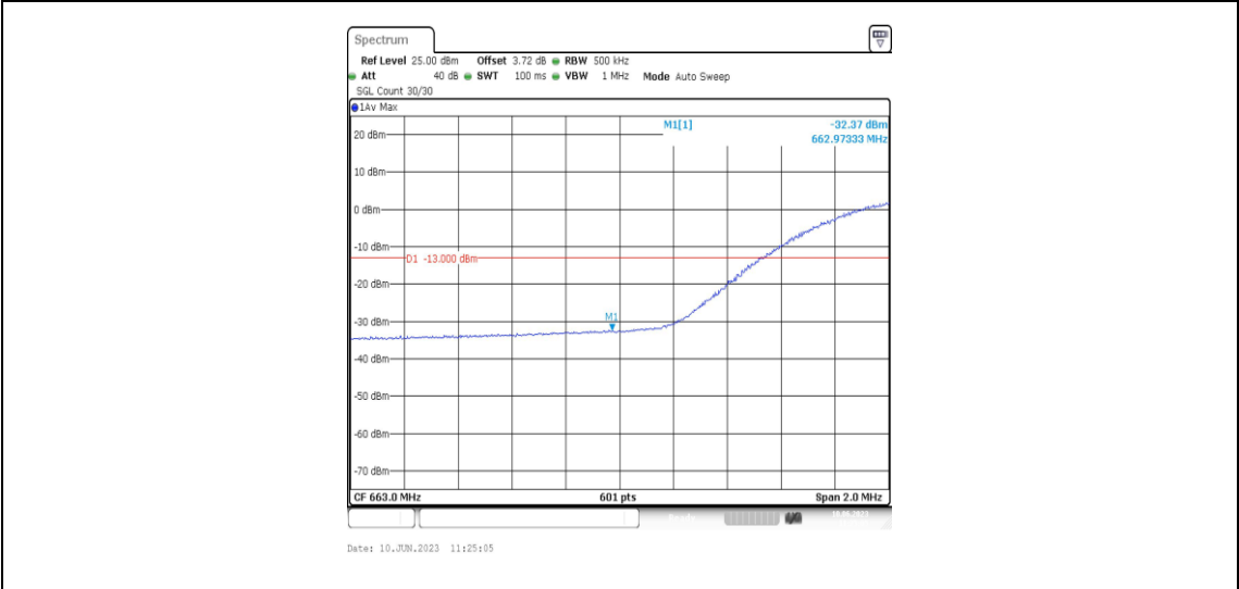
Band71-20MHz-QPSK-133222-100RB#0
