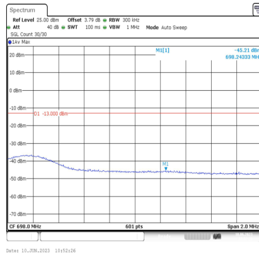
Band71-15MHz-QPSK-133397-1RB#0
