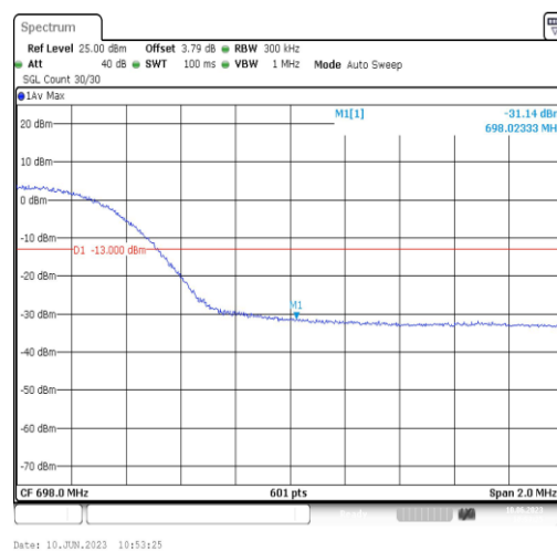
Band71-15MHz-16QAM-133397-75RB#0
