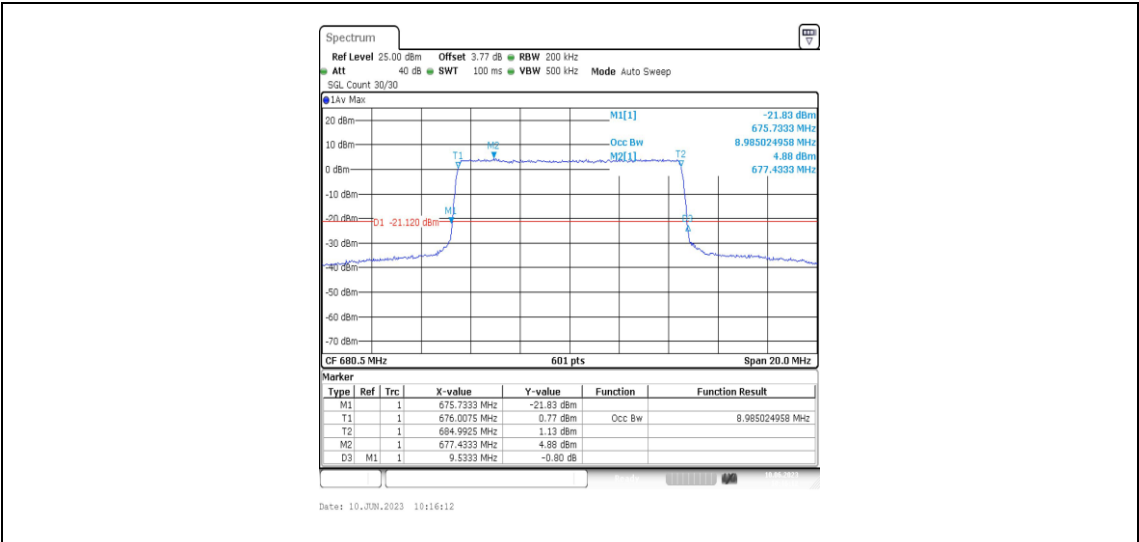
Band71-10MHz-16QAM-133297-50RB#0-8.985
