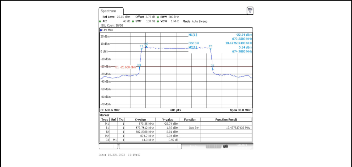
Band71-15MHz-QPSK-133297-75RB#0-13.478
