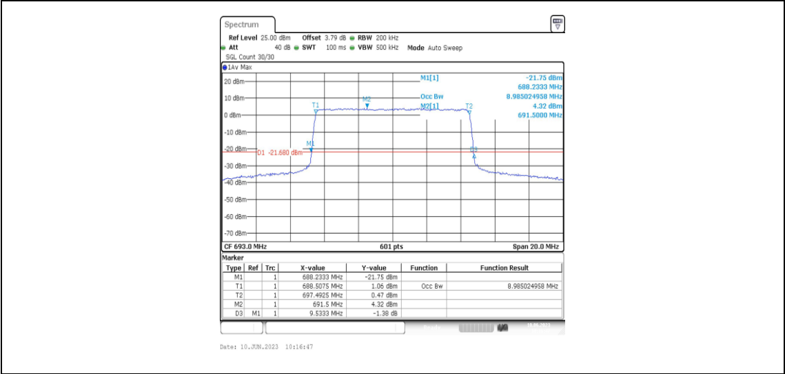
Band71-10MHz-16QAM-133422-50RB#0-8.985
