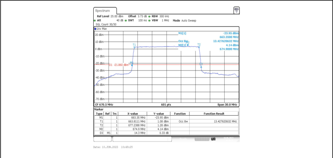
Band71-15MHz-16QAM-133197-75RB#0-13.428
