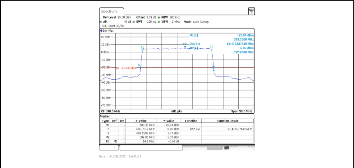
Band71-15MHz-QPSK-133397-75RB#0-13.478
