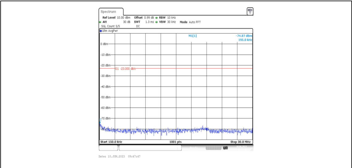
Band71-5MHz-16QAM-133147-1RB#0-Range2:0.15~30MHz
