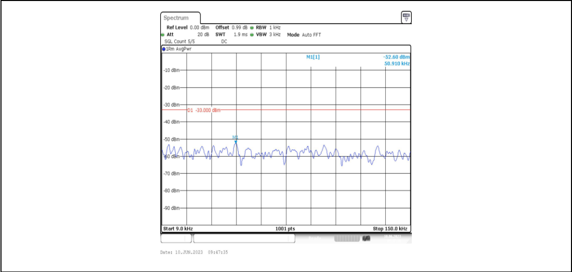
Band71-5MHz-16QAM-133147-1RB#0-Range1:0.009~0.15MHz
