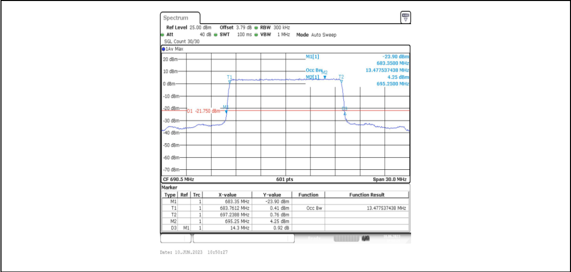
Band71-15MHz-16QAM-133397-75RB#0-13.478
