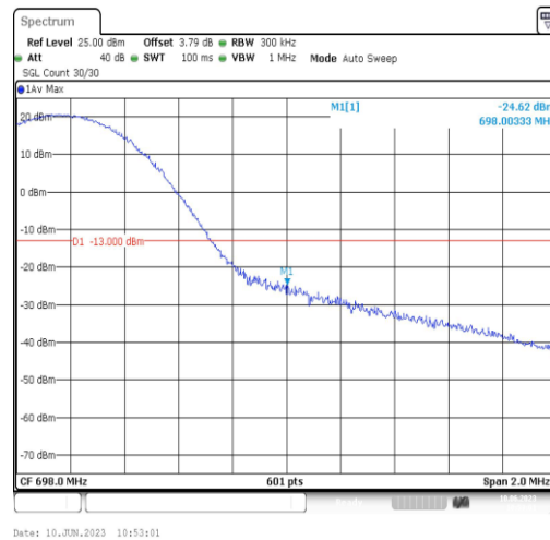
Band71-15MHz-16QAM-133397-1RB#74
