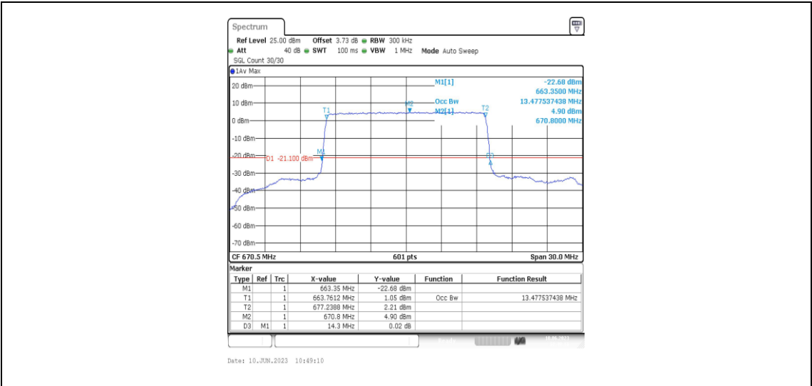
Band71-15MHz-QPSK-133197-75RB#0-13.478
