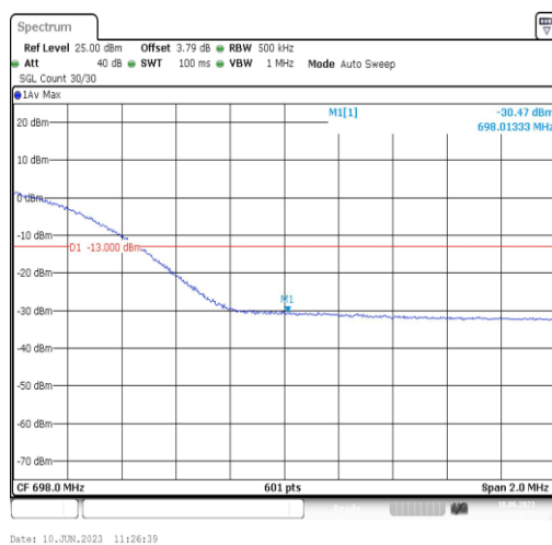
Band71-20MHz-16QAM-133372-100RB#0
