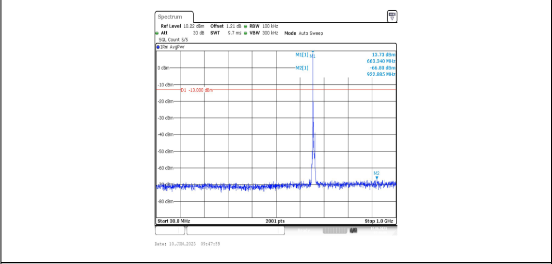
Band71-5MHz-16QAM-133147-1RB#0-Range3:30~1000MHz
