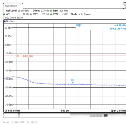
Band71-15MHz-16QAM-133397-1RB#0
