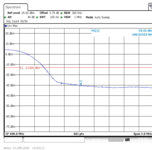
Band71-15MHz-QPSK-133397-75RB#0
