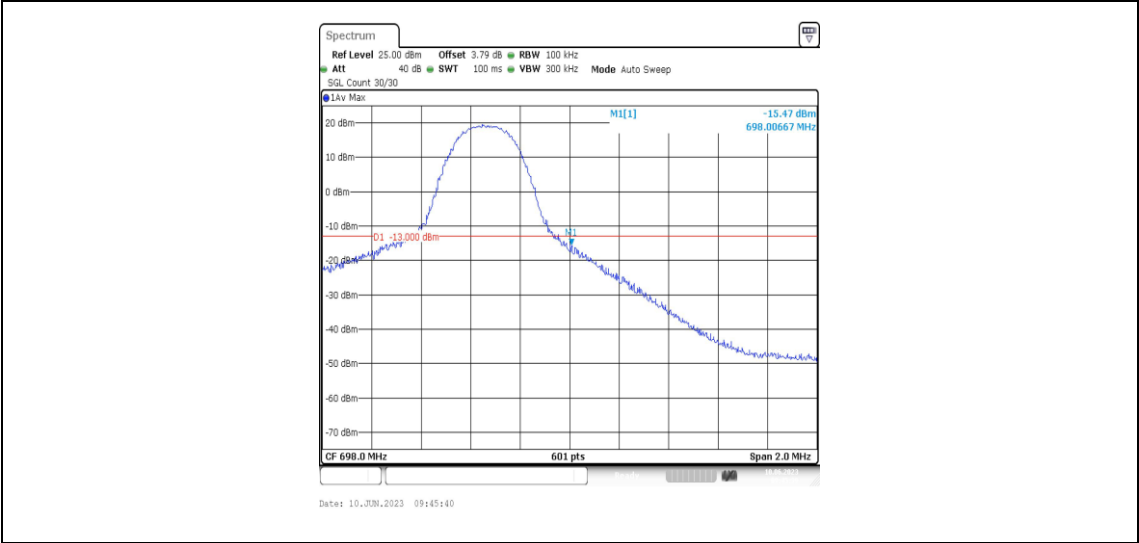
Band71-5MHz-QPSK-133447-1RB#24
