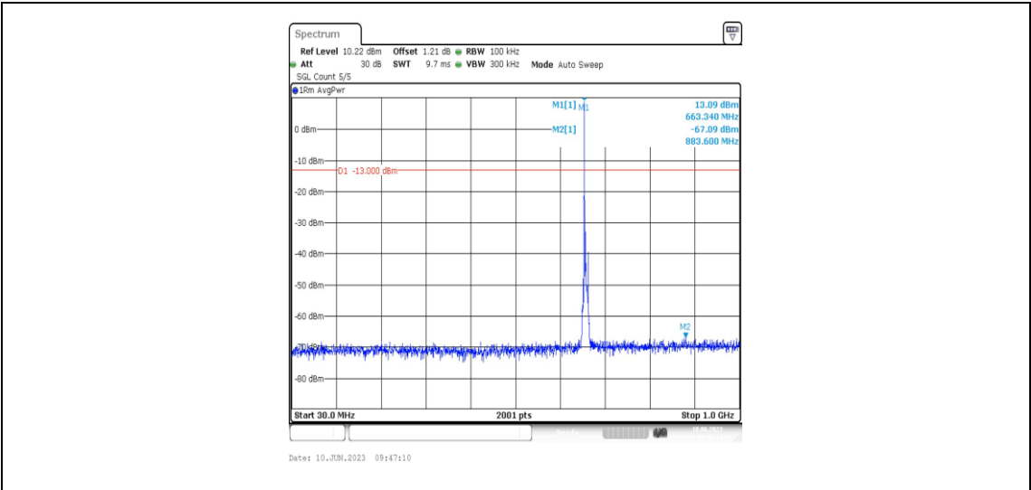
Band71-5MHz-QPSK-133147-1RB#0-Range3:30~1000MHz
