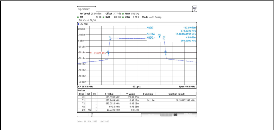
Band71-20MHz-16QAM-133322-100RB#0-18.103
