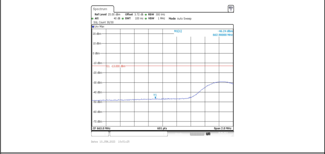
Band71-15MHz-QPSK-133197-1RB#74
