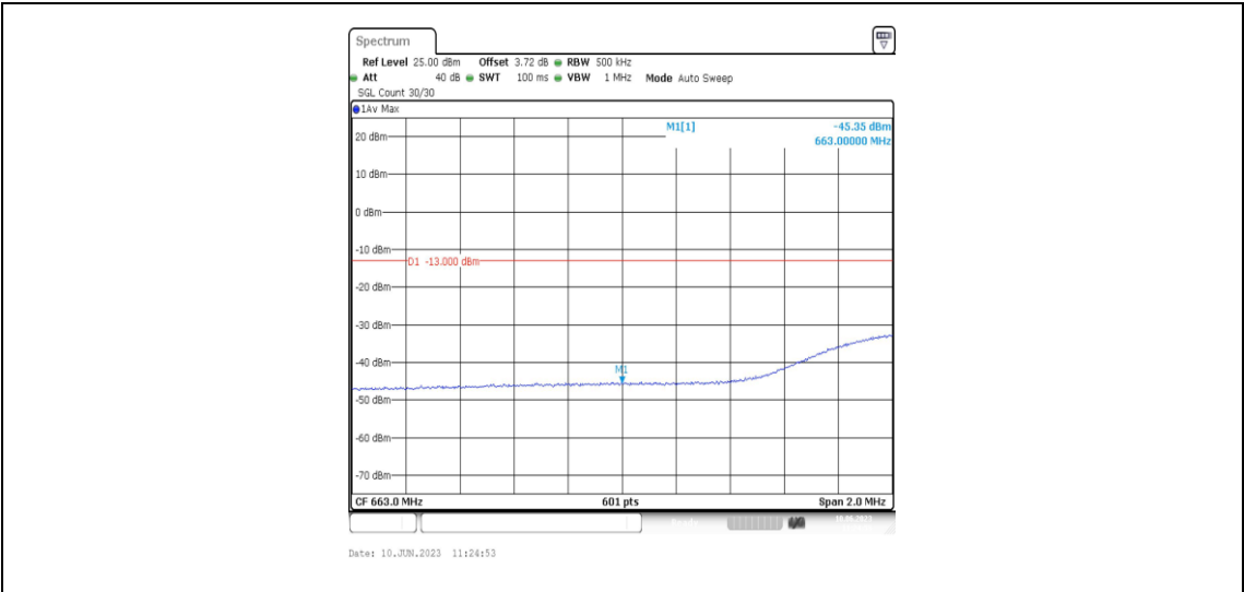
Band71-20MHz-16QAM-133222-1RB#99
