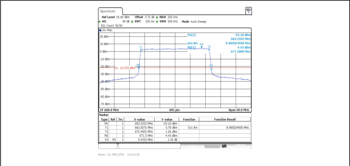
Band71-10MHz-16QAM-133172-50RB#0-8.985
