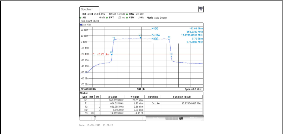
Band71-20MHz-QPSK-133222-100RB#0-17.97
