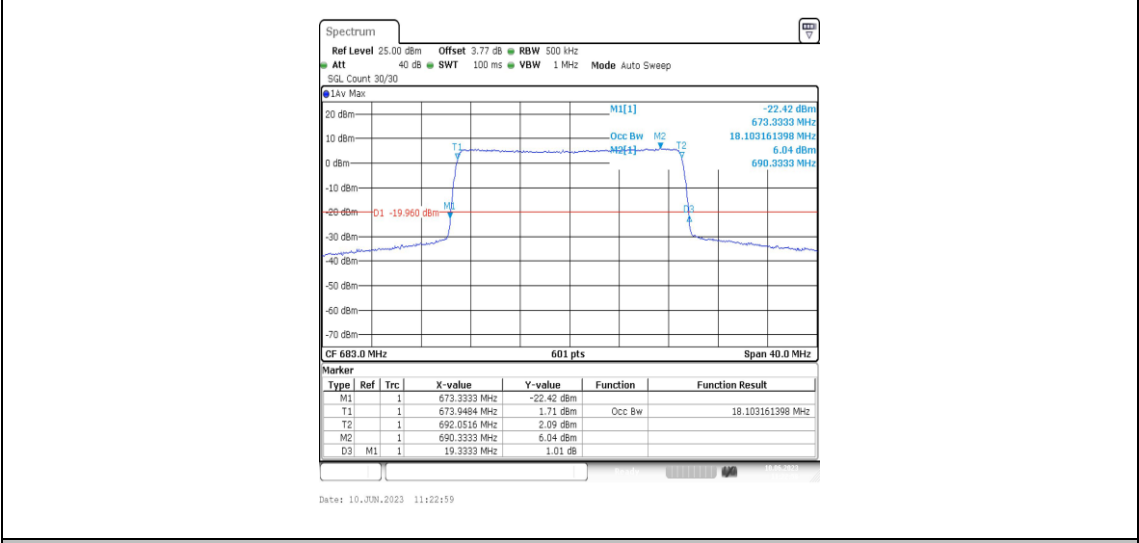
Band71-20MHz-QPSK-133322-100RB#0-18.103
