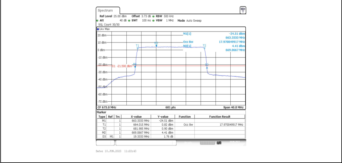
Band71-20MHz-16QAM-133222-100RB#0-17.97
