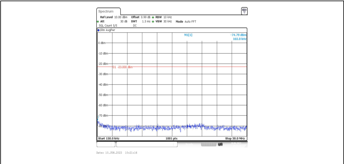
Band71-10MHz-16QAM-133172-1RB#0-Range2:0.15~30MHz
