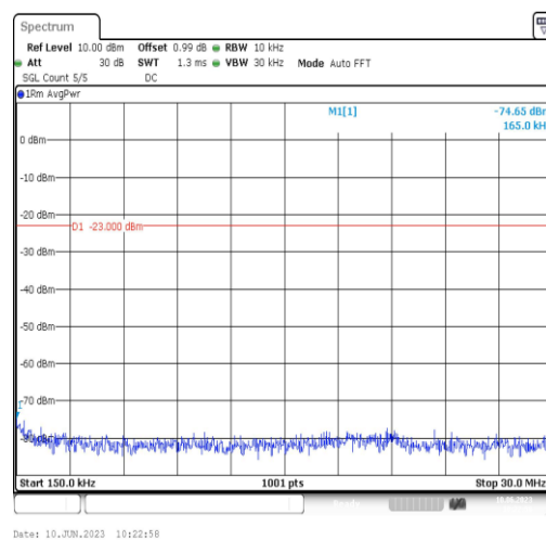
Band71-10MHz-16QAM-133297-1RB#0-Range2:0.15~30MHz
