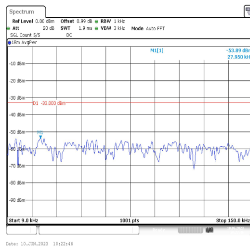
Band71-10MHz-16QAM-133297-1RB#0-Range1:0.009~0.15MHz
