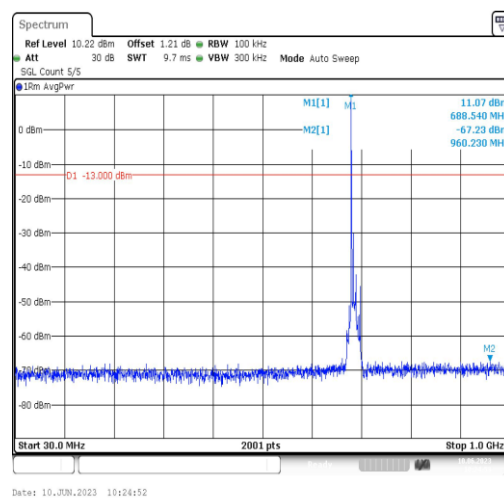
Band71-10MHz-16QAM-133422-1RB#0-Range3:30~1000MHz
