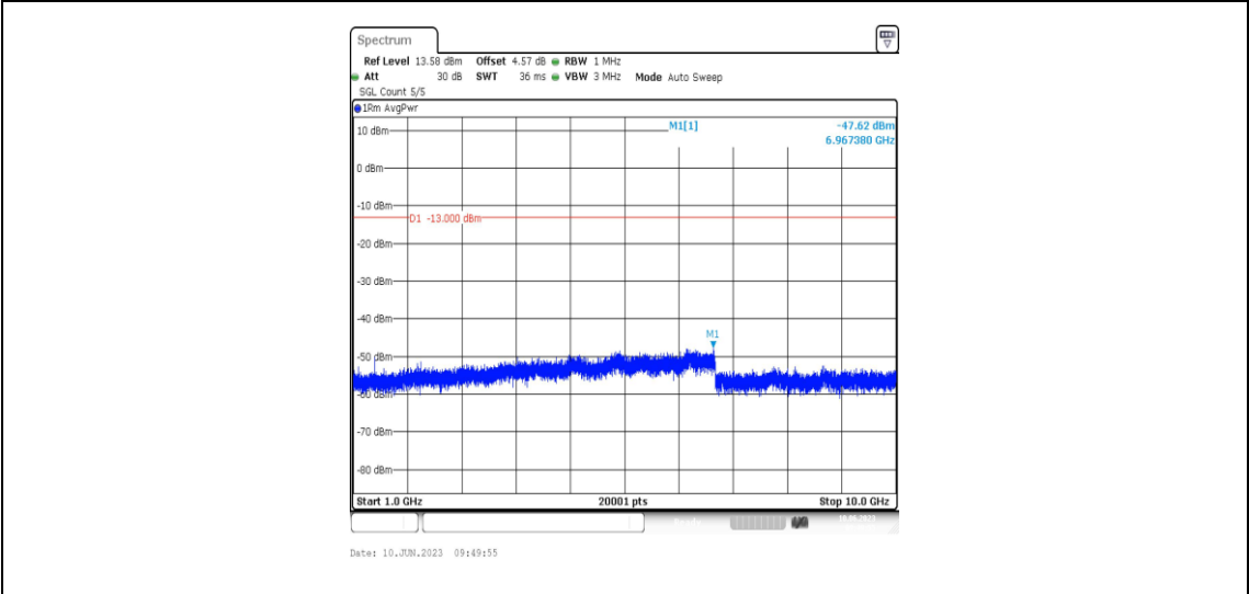
Band71-5MHz-16QAM-133297-1RB#0-Range4:1000~10000MHz
