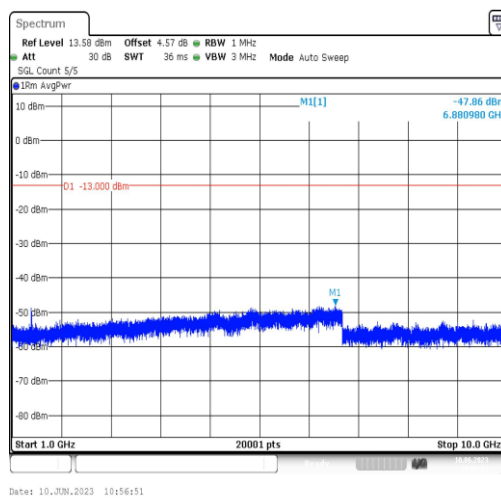
Band71-15MHz-16QAM-133297-1RB#0-Range4:1000~10000MHz
