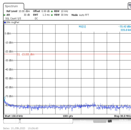
Band71-10MHz-16QAM-133422-1RB#0-Range2:0.15~30MHz
