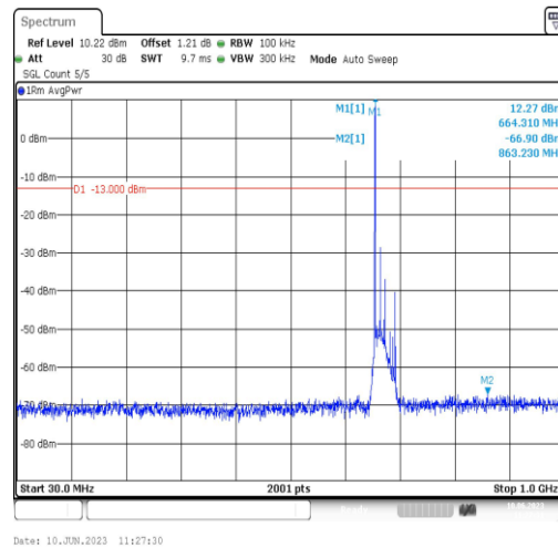
Band71-20MHz-QPSK-133222-1RB#0-Range3:30~1000MHz
