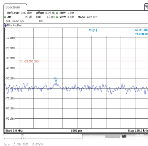
Band71-20MHz-16QAM-133222-1RB#0-Range1:0.009~0.15MHz
