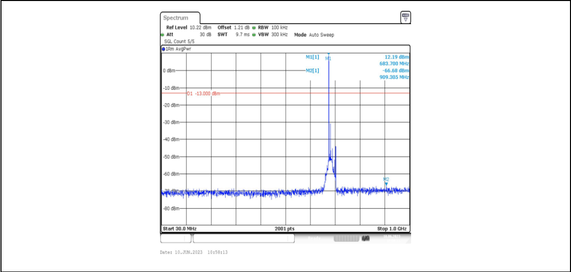
Band71-15MHz-16QAM-133397-1RB#0-Range3:30~1000MHz
