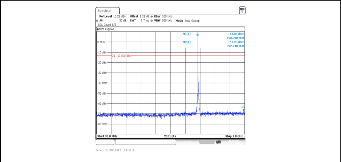
Band71-5MHz-16QAM-133447-1RB#0-Range3:30~1000MHz
