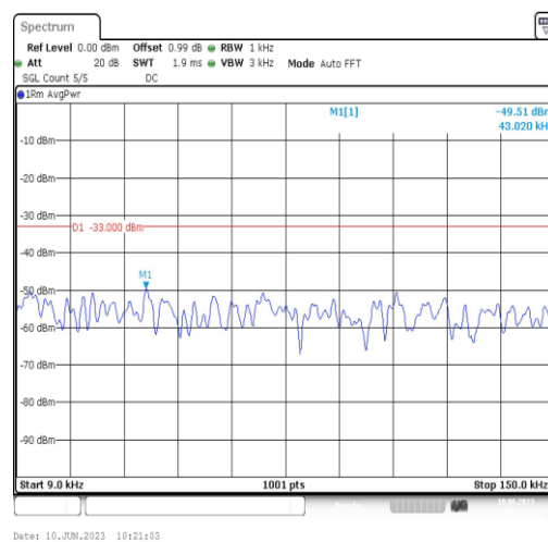
Band71-10MHz-16QAM-133172-1RB#0-Range1:0.009~0.15MHz
