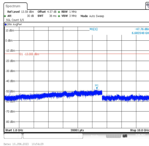
Band71-15MHz-QPSK-133197-1RB#0-Range4:1000~10000MHz
