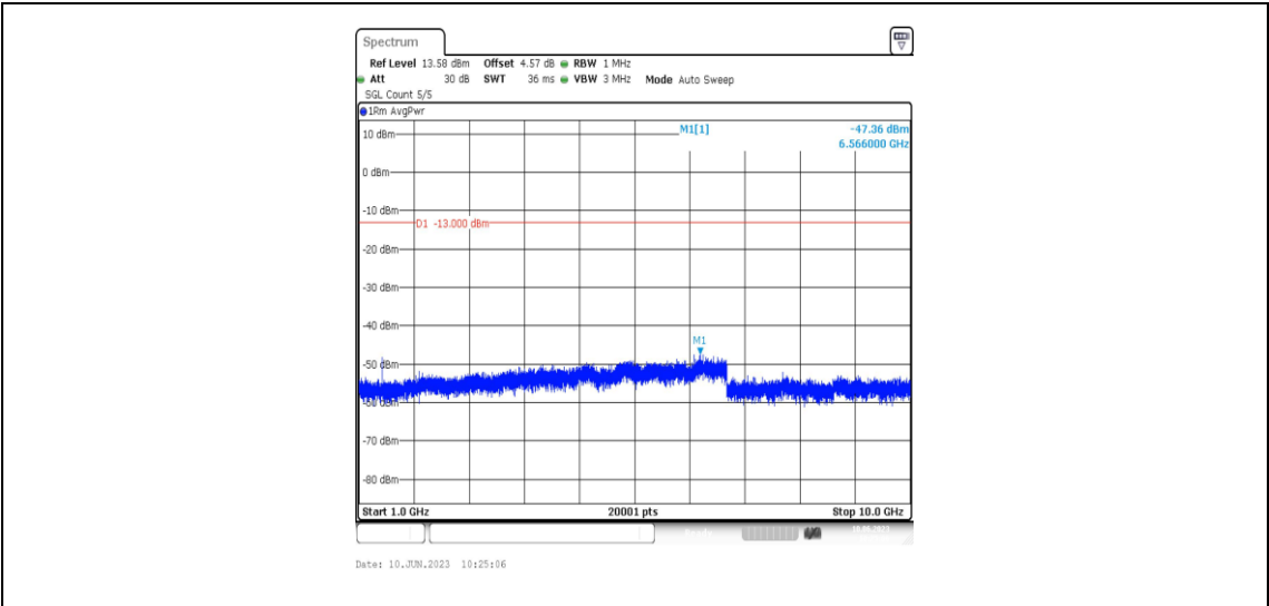
Band71-10MHz-16QAM-133422-1RB#0-Range4:1000~10000MHz
