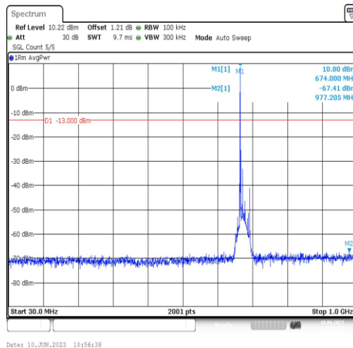
Band71-15MHz-16QAM-133297-1RB#0-Range3:30~1000MHz
