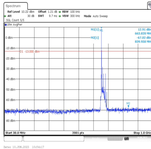
Band71-15MHz-QPSK-133197-1RB#0-Range3:30~1000MHz
