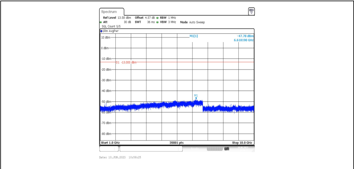
Band71-15MHz-16QAM-133397-1RB#0-Range4:1000~10000MHz
