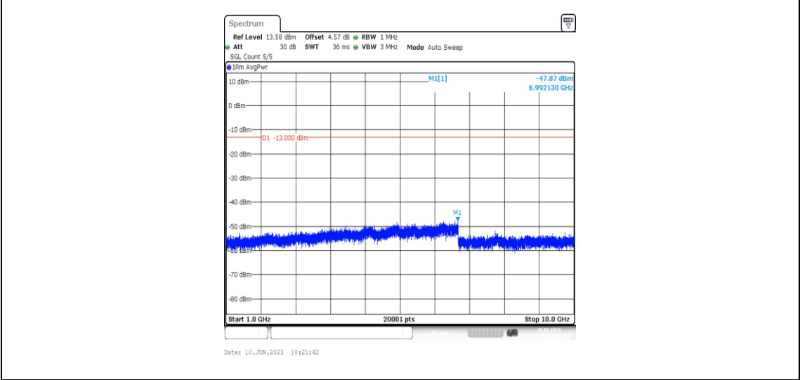
Band71-10MHz-16QAM-133172-1RB#0-Range4:1000~10000MHz
