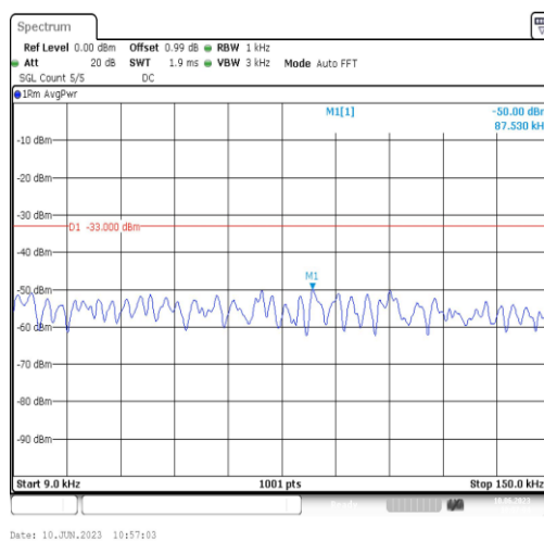
Band71-15MHz-QPSK-133397-1RB#0-Range1:0.009~0.15MHz
