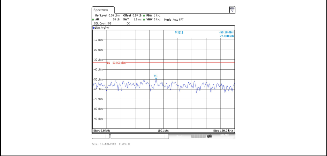
Band71-20MHz-QPSK-133222-1RB#0-Range1:0.009~0.15MHz
