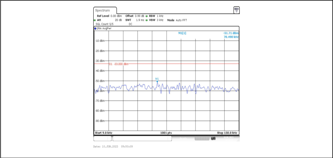
Band71-5MHz-QPSK-133447-1RB#0-Range1:0.009~0.15MHz
