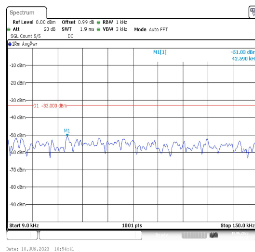
Band71-15MHz-16QAM-133197-1RB#0-Range1:0.009~0.15MHz
