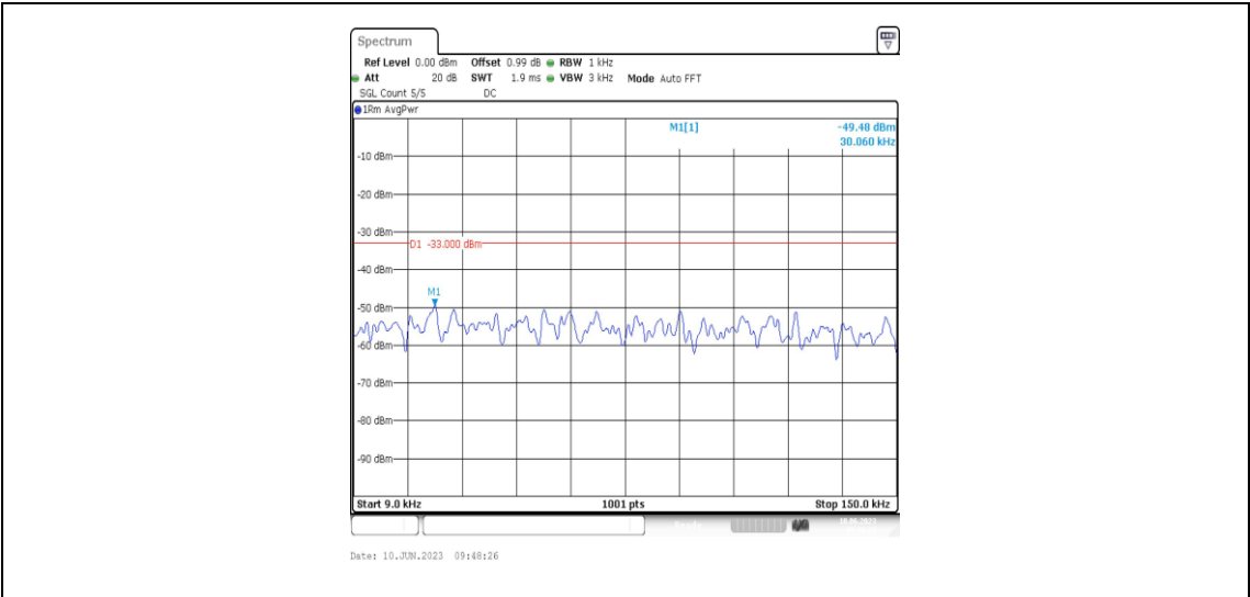
Band71-5MHz-QPSK-133297-1RB#0-Range1:0.009~0.15MHz
