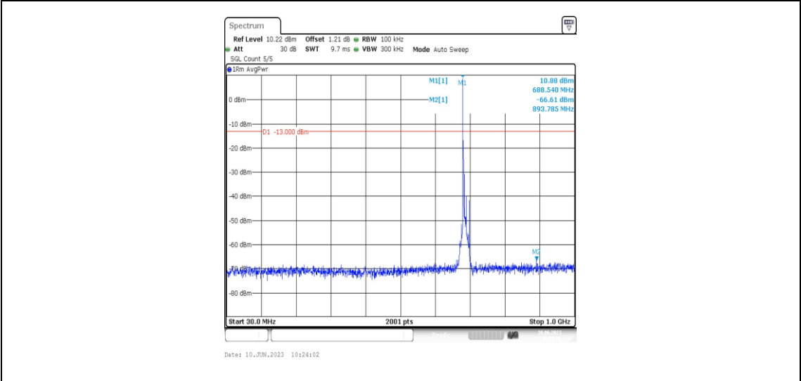
Band71-10MHz-QPSK-133422-1RB#0-Range3:30~1000MHz
