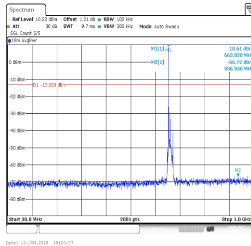
Band71-10MHz-QPSK-133172-1RB#0-Range3:30~1000MHz
