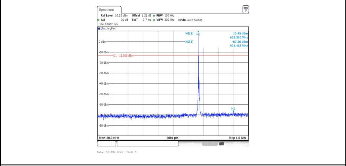
Band71-5MHz-QPSK-133297-1RB#0-Range3:30~1000MHz
