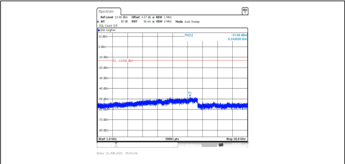
Band71-5MHz-16QAM-133447-1RB#0-Range4:1000~10000MHz
