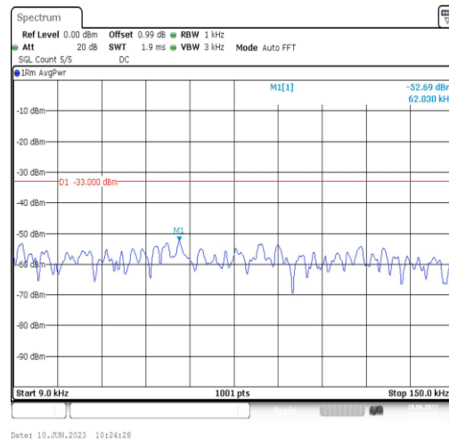
Band71-10MHz-16QAM-133422-1RB#0-Range1:0.009~0.15MHz
