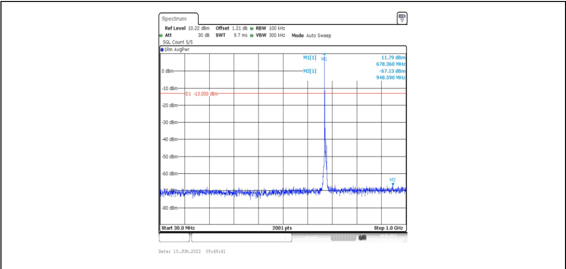
Band71-5MHz-16QAM-133297-1RB#0-Range3:30~1000MHz
